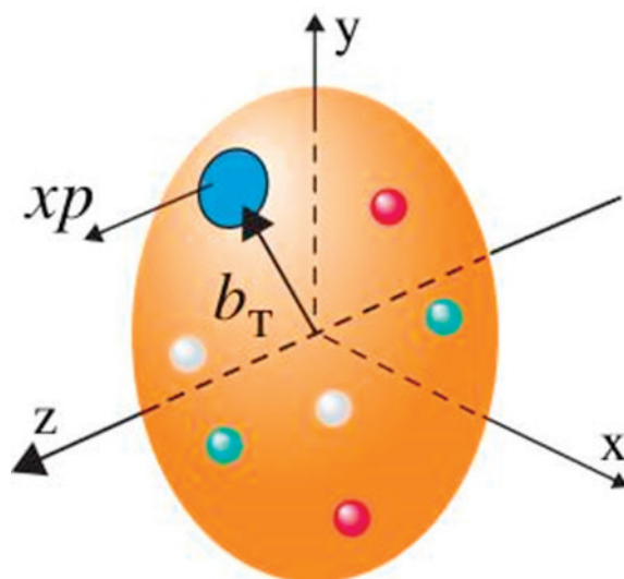
FIGURE 2.1.1 Schematic depiction of a nucleon containing a parton with longitudinal momentum xp and transverse position b_T = (b_x, b_y) . The z -direction is the beam direction. The transverse momentum (not shown) of the parton is k_T = (k_x, k_y) .
