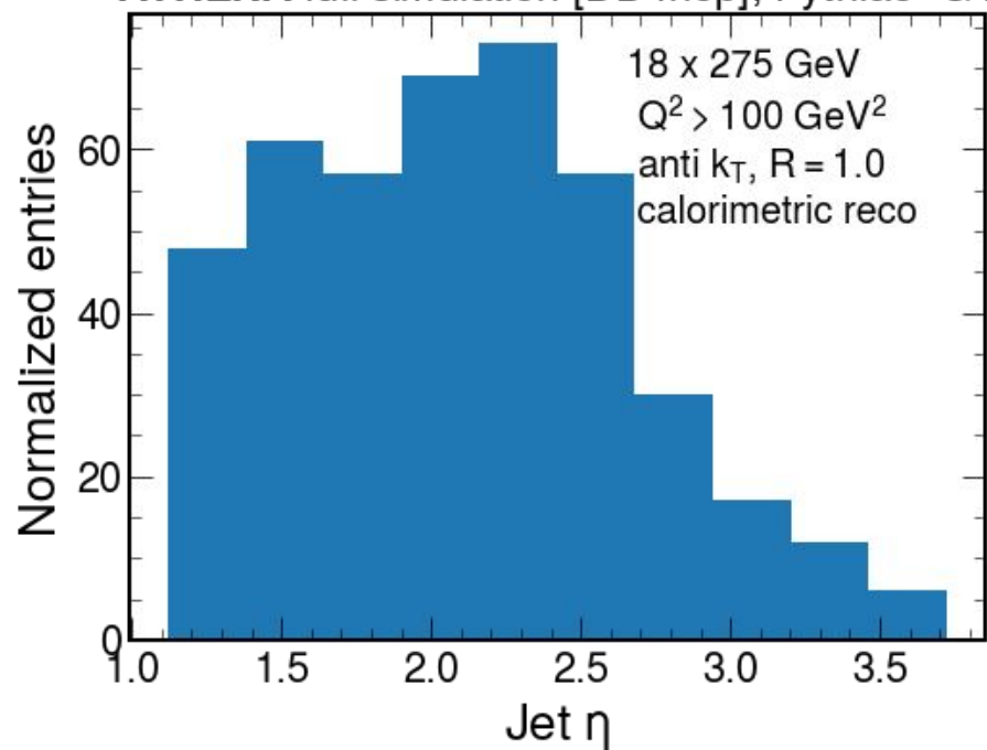
ATHENA full simulation [DD4hep], Pythia8+G4
