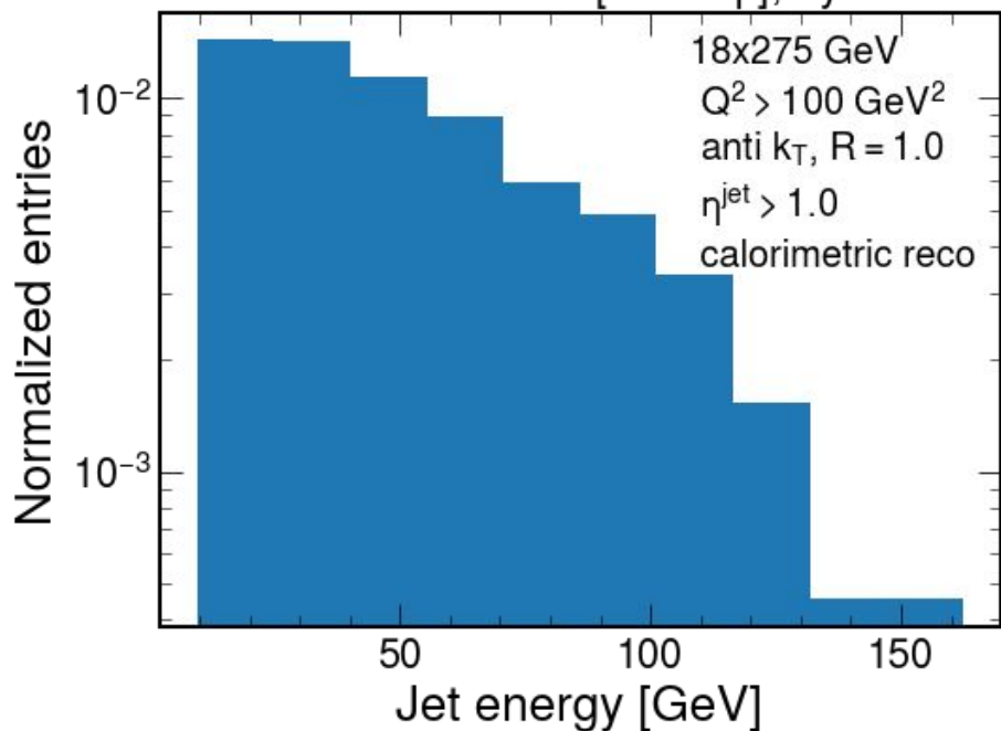
ATHENA full simulation [DD4hep], Pythia8+G4
