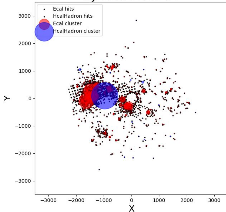
ATHENA simulation [DD4HEP] Pythia8+Geant4
