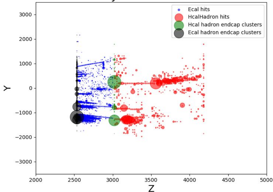
ATHENA simulation [DD4hep] Pythia8+Geant4
