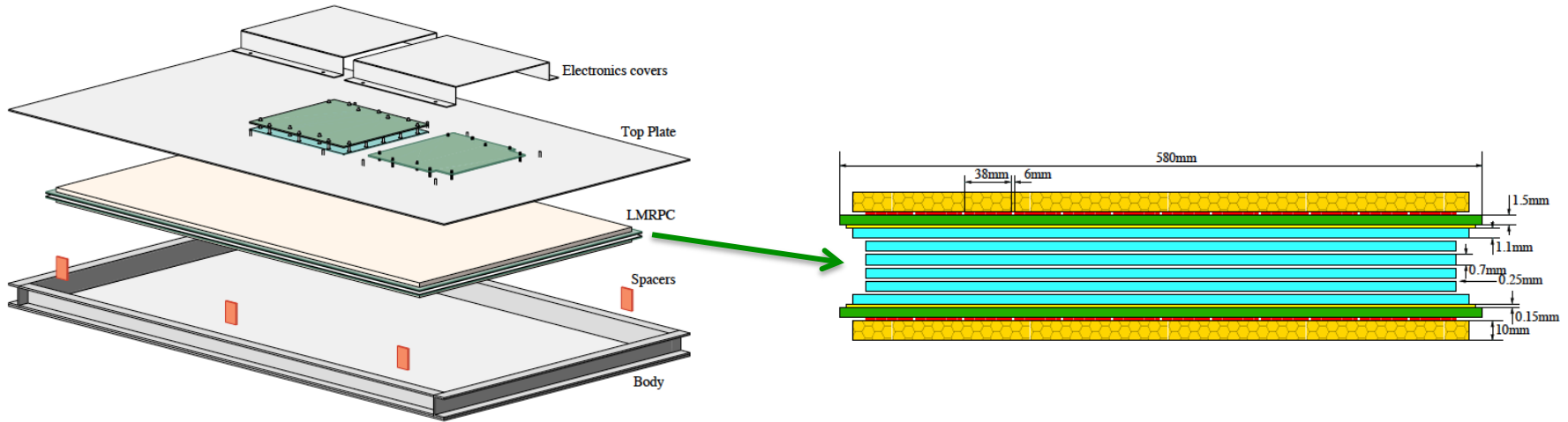
Figure 33. An exploded view of an MTD tray.
