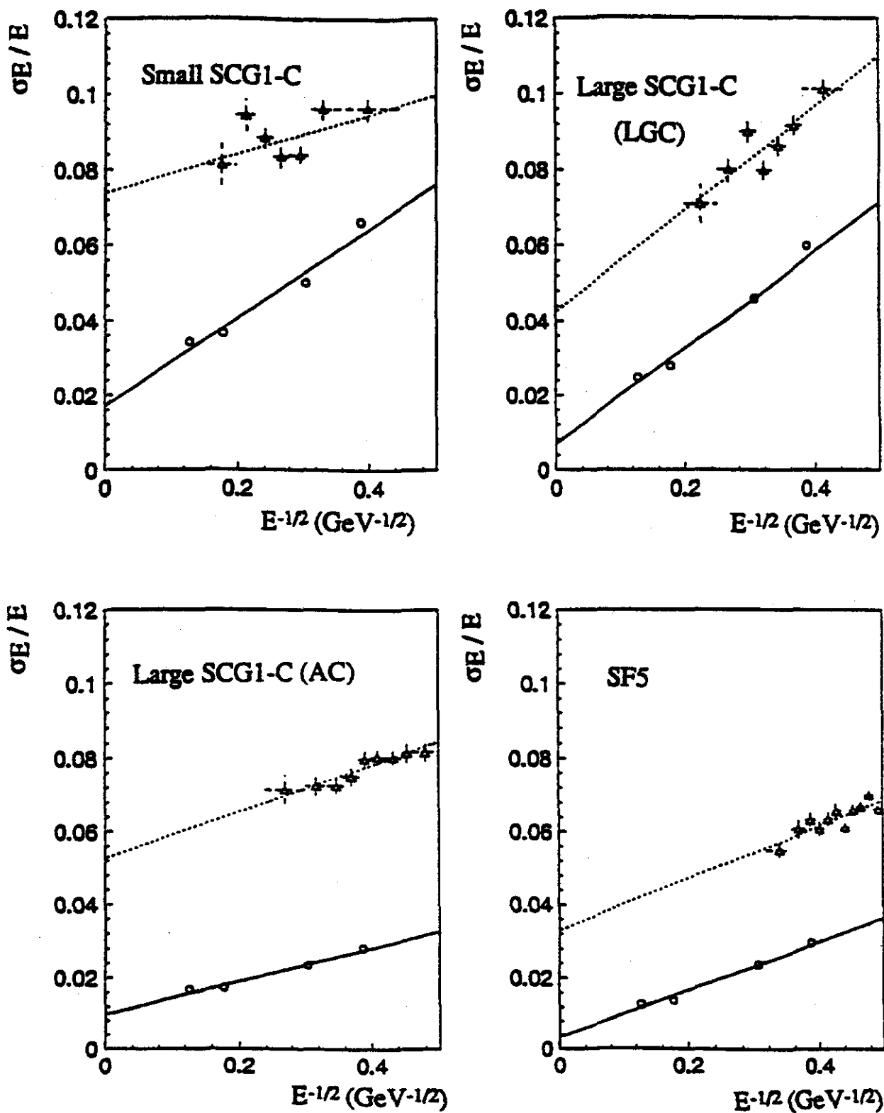
Figure 11. Fractional energy resolution \sigma(E)/E in various detector regions from calibration data (open circles) and electron/positron pairs in ordinary data (open triangles)
