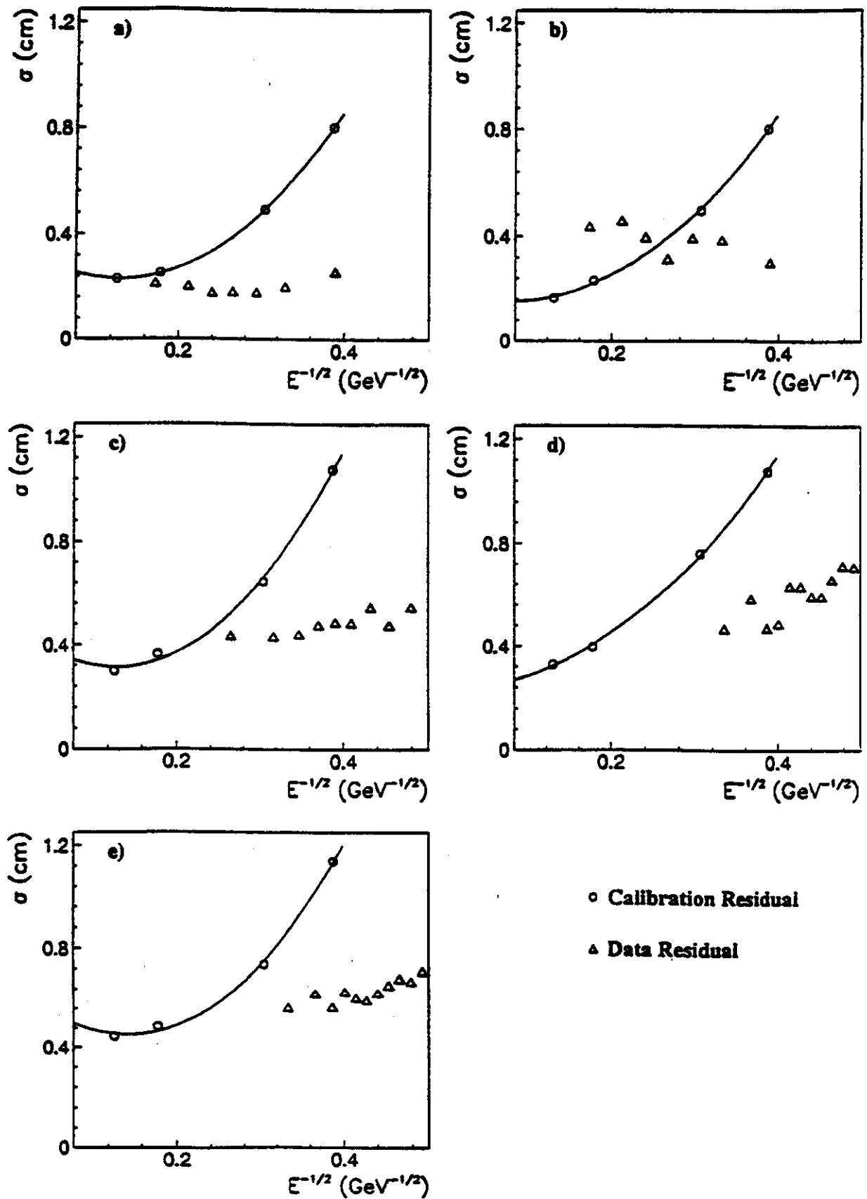
Figure 14. Position resolutions in various regions for calibration data (open circles) and electron/positron pairs from ordinary data (open triangles). The regions shown are (a) LGC, horizontal view; (b) LGC, vertical view; (c) GTH, single-tube width horizontal view; (d) GTH, vertical view; (e) GTH, double tube width horizontal view
