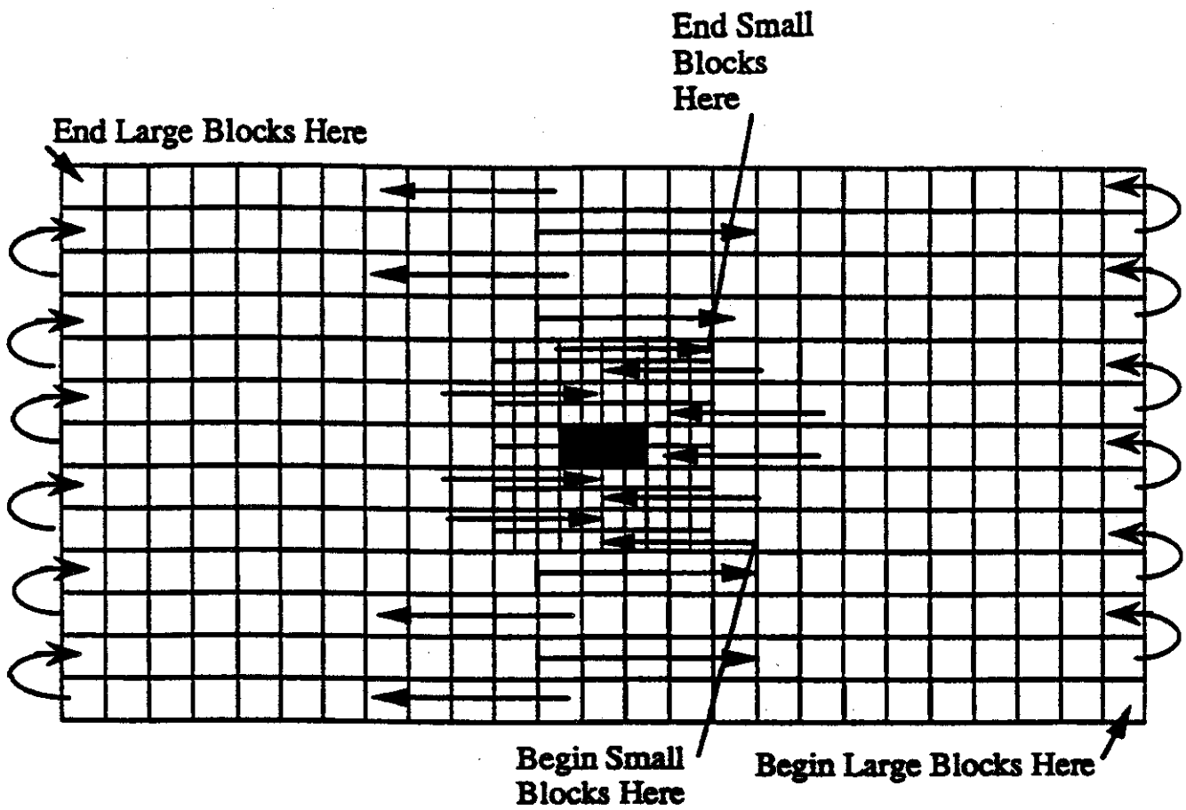
Figure 8. The Main Array glass block calibration sequence
