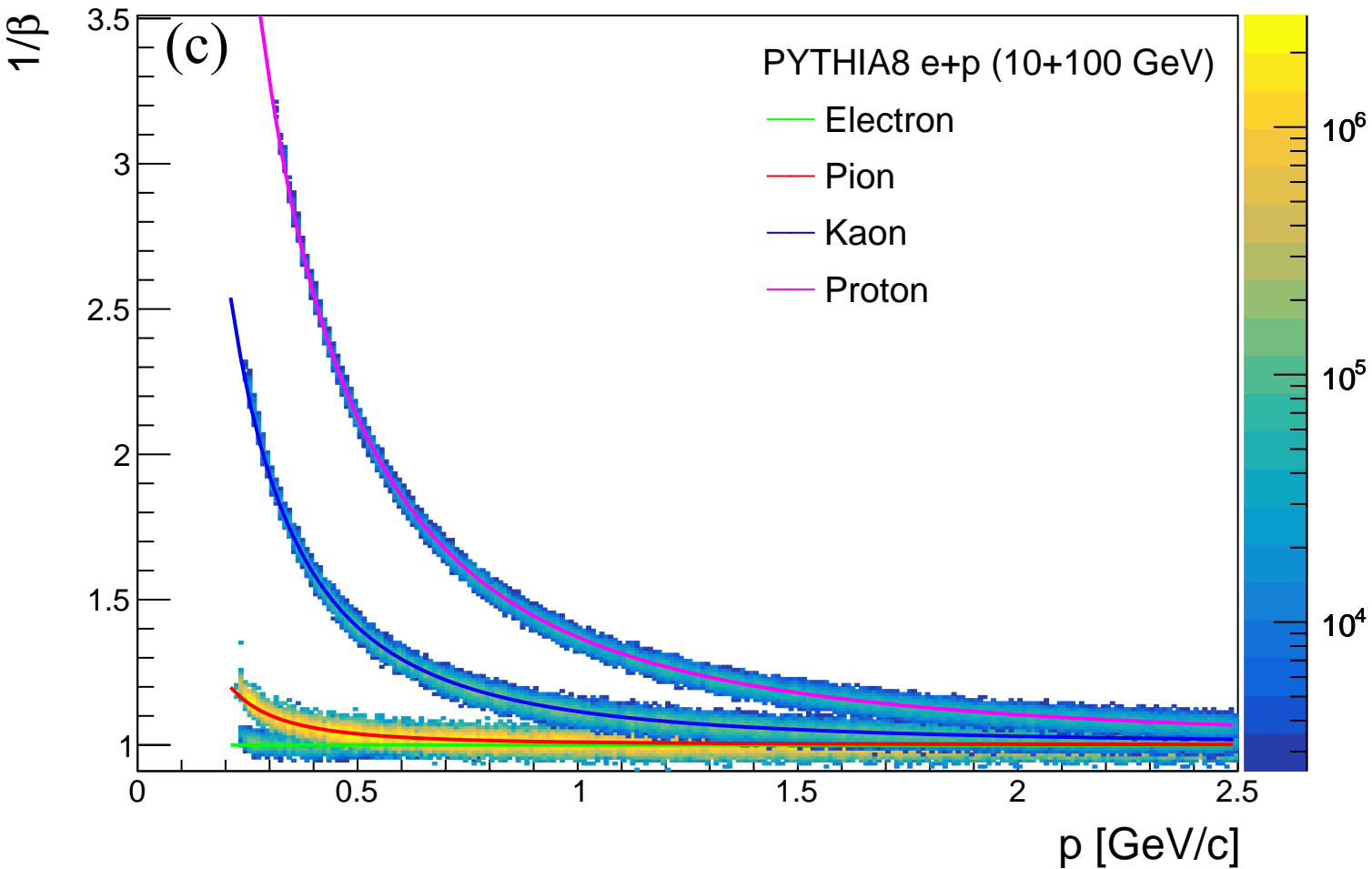
1/β vs momentum from ATHENA Barrel TOF at η=0
