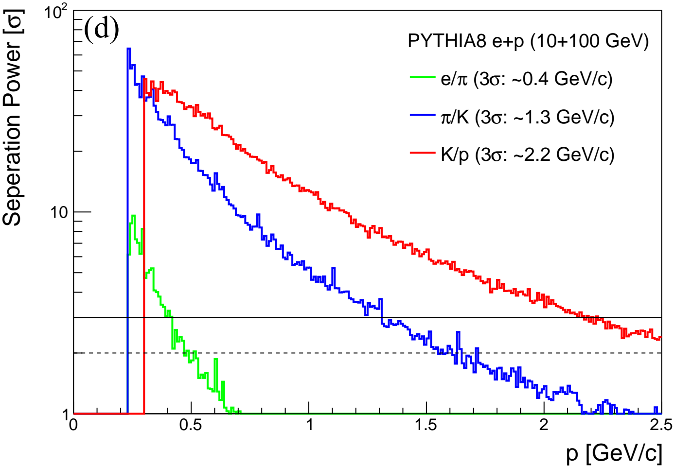
PID Separation Power by ATHENA Barrel TOF at \eta=0
