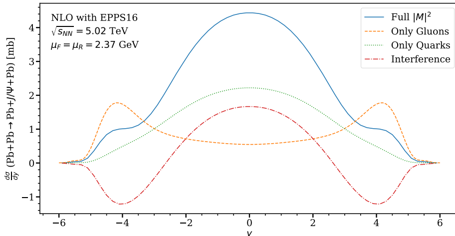
FIG. 7. Decomposition of the exclusive rapidity-differential J/\psi photoproduction cross section, computed with EPPS16 nPDFs at our “optimal” scale, in 5.02 TeV Pb+Pb UPCs (solid blue curve “Full |\mathcal{M}|^2 ”) into the contributions with zero quark distributions (dashed orange curve “Only Gluons”), with zero gluon distributions (dotted green curve “Only Quarks”) and the one with a mixing of the quark and gluon distributions in the square of the full NLO amplitude (red dashed-dotted curve “Interference”).
