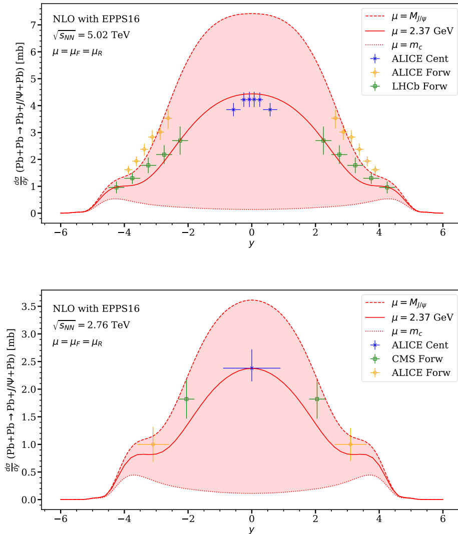
FIG. 1. Upper panel: The scale-choice uncertainty-envelope of the rapidity-differential exclusive J/\psi photoproduction cross section in ultraperipheral Pb+Pb collisions at \sqrt{s_{NN}} = 5.02 TeV, as a function of the J/\psi rapidity y , calculated to NLO pQCD with the EPPS16 nPDFs [44] and compared with the experimental data from Refs. [38] (ALICE Forw), [36] (ALICE Cent) and [41] (LHCb Forw). The experimental data points are mirrored w.r.t. y = 0 , and their errorbars are obtained by adding the statistical and systematic errors in quadrature. The solid (red) curve shows the NLO result with our “optimal” scale explained in the text. Lower panel: The same but at \sqrt{s_{NN}} = 2.76 TeV and with experimental data from Refs. [39] (ALICE Forw), [37] (ALICE Cent) and [40] (CMS Cent). For the errorbars of the data, all given errors are added in quadrature.
