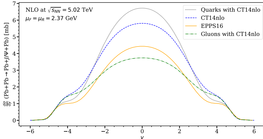
FIG. 9. Rapidity-differential exclusive J/\psi photoproduction cross section in 5.02 TeV Pb+Pb UPCs, computed with the EPPS16 nPDFs (solid orange curve), with CT14NLO PDFs (dashed blue curve), with CT14NLO gluons and EPPS16 quarks (dotted-dashed green curve), and with CT14NLO quarks and EPPS16 gluons. Notice that turning off the nuclear effects in gluons reduces the cross section at y = 0 – for explanation, see the text.
