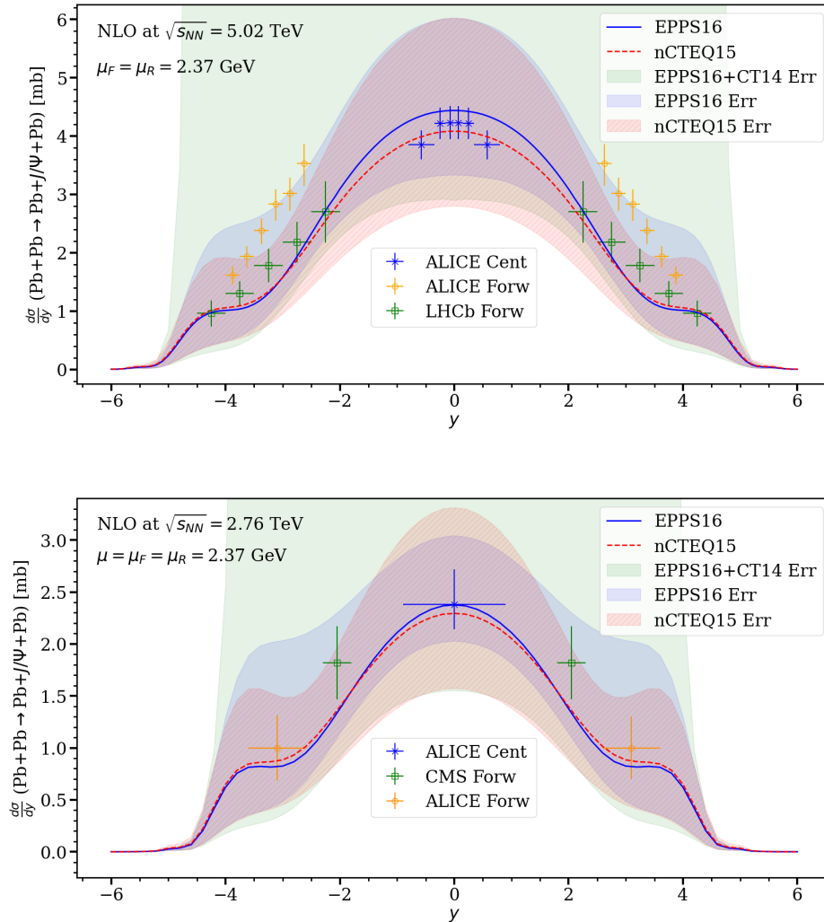
FIG. 13. Upper panel: Uncertainties originating from the nPDFs/PDFs in the rapidity-differential exclusive J/\psi photoproduction NLO cross sections in 5.02 TeV Pb+Pb UPCs, computed at our “optimal” scale \mu = 2.37 GeV using the EPPS16+CT14NLO and nCTEQ15 error sets. The solid (dashed) line shows the EPPS16+CT14NLO (nCTEQ15) central-set result, and the corresponding uncertainty bands are explained in the text. The experimental datapoints are from Run2 and the same as in the upper panel of Fig. 1. Lower panel: The same but for \sqrt{s_{NN}} = 2.76 TeV and with the same Run1 data as in the lower panel of Fig. 1.
