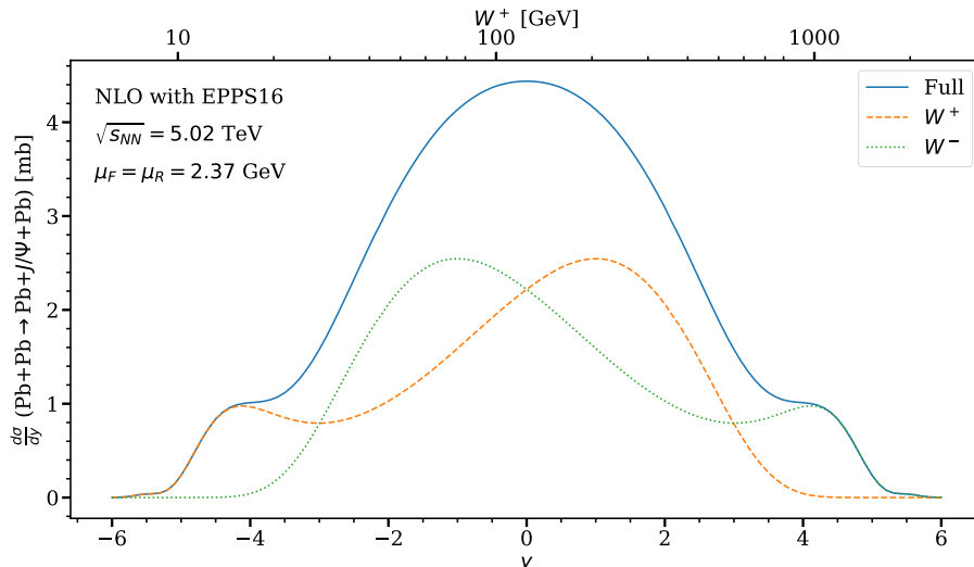
FIG. 5. Contributions from the W^+ (dashed, red curve) and W^- (dotted, green curve) terms in Eq. (4) to the NLO exclusive rapidity-differential J/\psi photoproduction cross section in 5.02 TeV Pb+Pb UPCs as a function of the J/\psi rapidity y , computed using EPPS16 nPDFs and with our “optimal” scale. The second x axis on the top shows the values of W^+ corresponding to each y .
