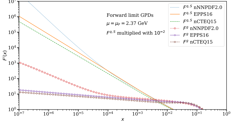
FIG. 11. The nPDF gluon distributions xg(x, \mu) and the quark singlet distributions F_i^{q,S} = \sum_q [q(x, \mu) + \bar{q}(x, \mu)] as given by EPPS16 (solid lines), nCTEQ15 (dashed) and nNNPDF2.0 (dotted) nPDFs at the “optimal” scale.
