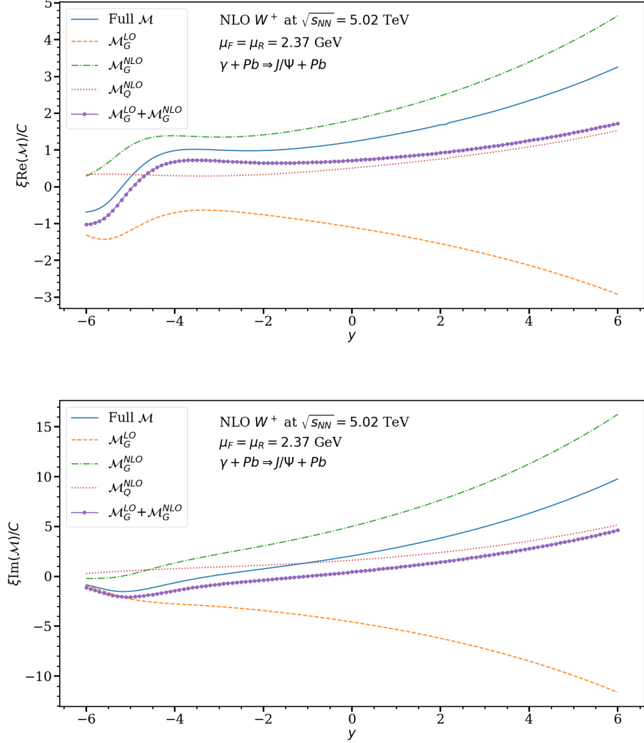
FIG. 8. Upper panel: The \xi/C -scaled real parts of the full amplitude \mathcal{M} (solid blue curve), LO gluon term \mathcal{M}_G^{LO} (dashed orange), NLO gluon term \mathcal{M}_G^{NLO} (dashed dotted green), sum of the LO and NLO gluon terms \mathcal{M}_G^{LO} + \mathcal{M}_G^{NLO} (solid purple with filled circles), and NLO quark term \mathcal{M}_Q^{NLO} (dotted red), as a function of the J/\psi rapidity y , for the contribution W^+ . For the definition of the scaling factor, see Eq. (13). Lower panel: The same but for the imaginary parts of the amplitudes. Notice the different vertical scale.
