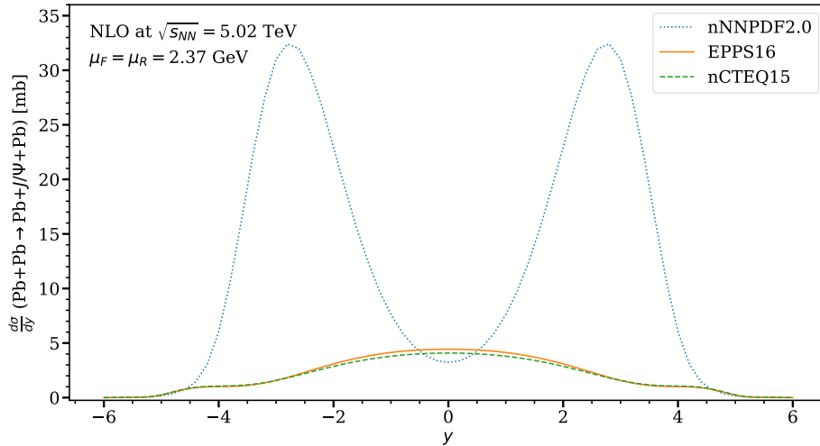
FIG. 10. Rapidity-differential exclusive photoproduction of J/\psi in 5.02 TeV Pb+Pb UPCs, computed at our “optimal” scale using the EPPS16 [44] (solid orange curve), nCTEQ15 [43] (dashed green) and nNNPDF2.0 [45] (dotted blue) nPDFs.
