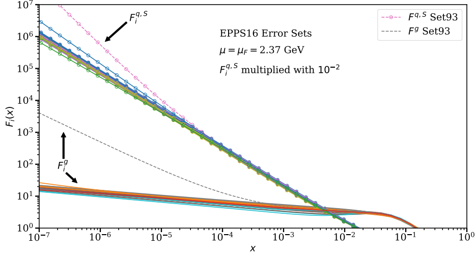
FIG. 12. The error sets of EPPS16&CT14NLO nPDFs&PDFs for the gluon (lower set of curves) and quark-singlet distributions (upper set) as functions of x , at our “optimal” scale. Altogether 96 error sets are plotted, of which the numbers 1-40 in the LHAPDF set-up [82] of EPPS16 are for the nuclear effects and 41-96 for the CT14NLO free-proton PDFs. The CT14NLO-related Set93 is the one clearly standing out from the rest at x \lesssim 10^{-4} .
