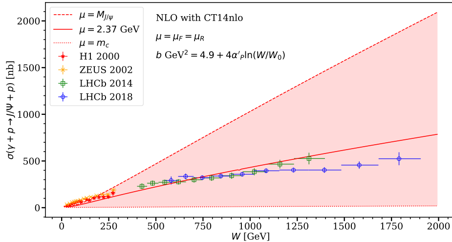
FIG. 2. The scale-choice uncertainty-envelope of exclusive J/\psi photoproduction NLO cross sections in ep and pp collisions as a function of the photon-proton c.m.s. energy W , computed to NLO pQCD with the CT14NLO [62] PDFs and compared against the experimental HERA data from H1 [26] and ZEUS [27], and LHC data from LHCb [28, 29]. The solid (red) line corresponds to the “optimal” scale explained in the text.
