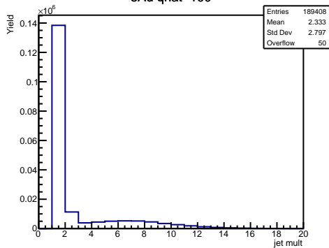
eAu qhat=100
