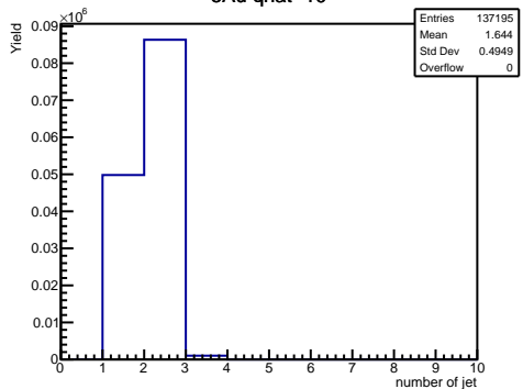
eAu qhat=10
