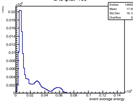
eAu qhat=100
