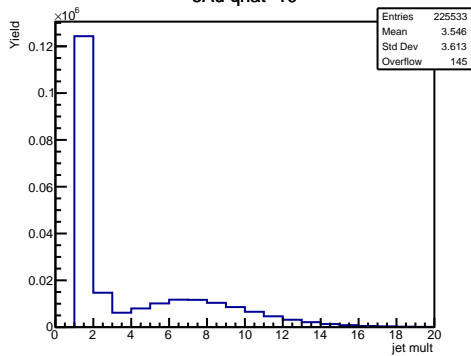
eAu qhat=10
