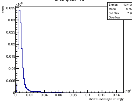
eAu qhat=10
