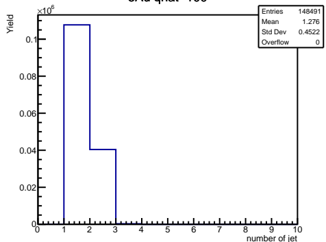
eAu qhat=100
