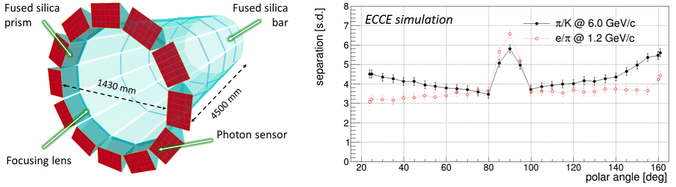
Figure 15: hpDIRC geometry (left) and expected PID performance (right) from the GEANT4 standalone simulation. The e/\pi and \pi/K separation power is shown in units of number of standard deviations (s.d.) as a function of the particle polar angle for e/\pi at 1.2 GeV/c and \pi/K up to 6 GeV/c.
