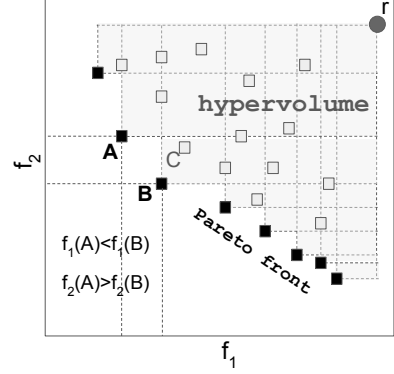
Figure 2: Example of Pareto frontier in a two-dimensional objective space: The point C is not on the frontier and is dominated by both point A and point B. All the other points which are dominated by the Pareto frontier and that satisfy any constraints in the optimization problem are called feasible solutions; The hypervolume is used as a metric for convergence, and is calculated with respect to a reference point r .
