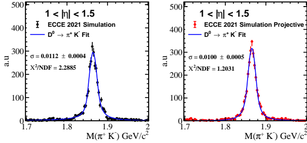
Figure 9: Analysis of SIDIS events with AI-assisted detector designs: The \pi^+ K^- invariant mass obtained from the SIDIS events reconstructed in ECCE. A comparison of the resolution on the D^0 meson obtained with the non-projective and the projective design of the ECCE tracker is shown. In order to emphasize the improvement in the region between 1.0 < |\eta| < 1.5 , a selection was made such that both the tracks \pi^+ or the K^- are within the region of interest. The resolution with the projective design is improved by more than 10% relative to the resolution obtained with the non-projective design.
