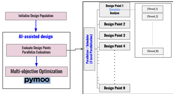
Figure 10: Flowchart of the two-level parallelization implemented for detector design: Multiple design points are produced in parallel, and each design point is parallelized. The design is assisted by an AI-strategy, in this case MOO with evolutionary algorithms supported by pymoo [13].
