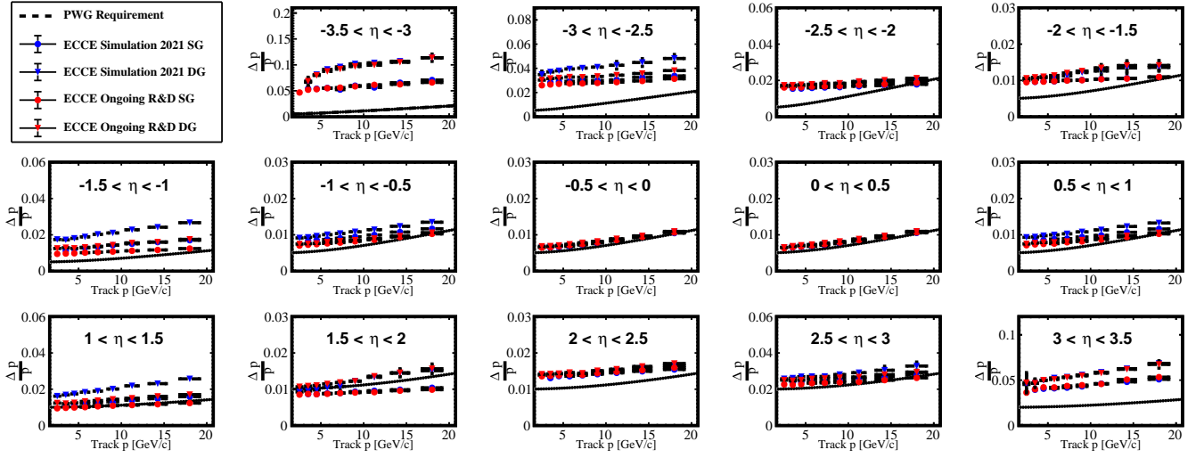
Figure B.13: Momentum resolution for the ECCE tracker reference design and the projective design (ongoing R&D): The \Delta p/p are extracted with single-gaussian (SG) fits (circles) to be consistent with the YR PWG and compared to double-gaussian (DG) fits (triangles). DG (see Eq. (3)) is used in the AI-assisted pipelines as it provides more stable fits. DG results are systematically larger than the SG ones as they capture more realistic distributions (see Fig. 6). This effect is larger in 1 < |\eta| < 1.5 for the non-projective design (blue points) since more material is traversed by the tracks; the same effect is moderately present also in 0.5 < |\eta| < 1 for the same reason. In the same bins, the ongoing R&D design shows a significant reduction of the impact of the readout and services and SG (red circle) and DG (red triangles) are close to each other. DG points are systematically large in 3 < \eta < 3.5 and in -3.5 < \eta < 3.0 , and this corresponds to edge effects at large |\eta| values close to the inner radii of the disks in the endcaps. In the region -1 < \eta < 3.0 \Delta p/p is consistent with the YR physics requirements with SG. Note that physics in the backward region relies on the EM calorimeter also, and in the proposal it has been demonstrated that larger resolutions are acceptable.
