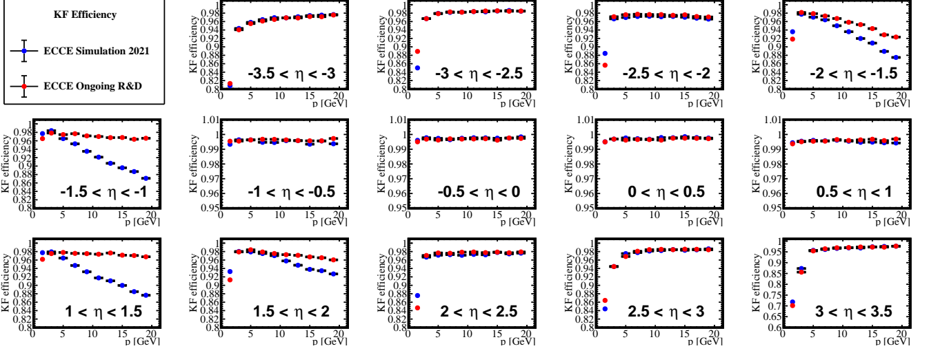
Figure B.15: KF Efficiency for ECCE projective geometry and ECCE simulation: Reconstruction efficiency shows an improvement in the transition region between 1.0 < |\eta| < 1.5 . There is a significant drop in the transition region caused due to multiple scattering of the support structure.
