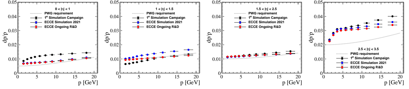
Figure 8: Evolution of momentum resolution driven by the continued MOO: Momentum resolutions in four bins of \eta . From left to right, respectively: |\eta| < 1.0 corresponding to the barrel, 1.0 < |\eta| < 1.5 corresponding to the transition region, and 1.5 < |\eta| < 2.5 and 2.5 < |\eta| < 3.5 corresponding to the two end-caps. Black points represent the first simulation campaign, and a preliminary detector concept in phase-I optimization which did not have a developed support structure; blue points represent the fully developed simulations for the final ECCE detector proposal concept; red points the ongoing R&D for the optimization of the support structure. Compared to black, there is an improvement in performance in all \eta bins with the exception of the transition region, an artifact that depends on the fact that black points do not include a realistic simulation of the material budget in the transition region. In the transition region, it can be also appreciate the improvement provided by the projective design.
