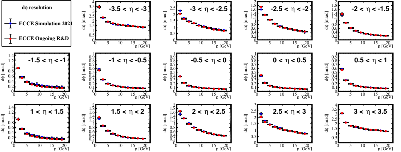
Figure B.16: Angular resolution ( d\phi ) for ECCE projective geometry and ECCE simulation: The resolution shows an improvement in the transition region between 1.0 < |\eta| < 1.5 . These plots have been produced using double-Gaussian fits.
