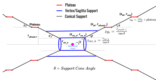
Figure A.12: Parametrization of the support cone for the inner tracker: The inner tracker support is characterised by five variables: \theta (the angle of projection of the support cone structure), r_{\text{vtx}} (radius of vertex support structure), r_{\mu\text{rwell}-1} \mu\text{Rwell-1} radius, plateau length, r_{\text{max}} maximum allowed radius of inner tracker).
