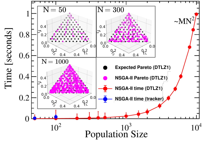
Figure 11: The computing time taken by the genetic algorithm and the sorting in NSGA-II: Performance has been benchmarked with test problems like DTLZ1 [16] (red points) and the scaling \sim MN^2 (see Table 1) has been verified with convergence to the Pareto front. The simulation time dominates the AI time during the optimization process (blue point). A two-level parallelization has been introduced in the framework to reduce this bottleneck. The AI contribution typically becomes dominant when very large population size is needed to accurately approximate the Pareto front (cf.[31]).
