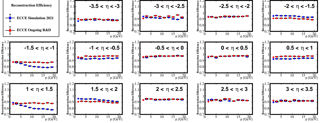
Figure B.17: Reconstruction efficiency for ECCE projective geometry and ECCE simulation: Reconstruction efficiency shows an improvement in the transition region between 1.0 < |\eta| < 1.5
