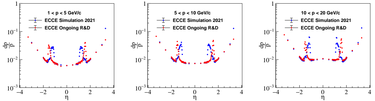
Figure B.18: Comparison between non-projective and projective inner tracker: a comparison in momentum resolution as a function of the pseudorapidity \eta between the non-projective and the projective designs in three bins of momentum. The projective design concentrates the material in a smaller dead area resulting in better resolution on a wider range of the pseudorapidity.
