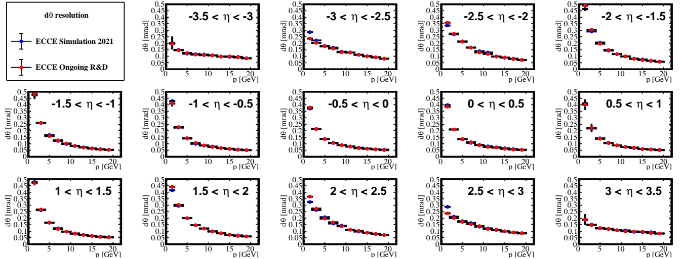
Figure B.14: Angular resolution ( d\theta ) for ECCE projective geometry and ECCE simulation: The resolution shows an improvement in the transition region between 1.0 < |\eta| < 1.5 . These plots have been produced using double-Gaussian fits.
