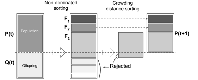
Figure 3: The NSGA Workflow: At time t , an offspring Q(t) is created through a genetic algorithm [15] from an N -sized population of design points P(t) . The two populations are combined into an augmented population which is classified into different non-dominated classes F_i , starting from the first front F_1 . To restore the initial size of the population, the augmented space of solutions is trimmed. A metric called crowding distance is used to reject solutions and eventually provide an updated population of size N at time t + 1 .
