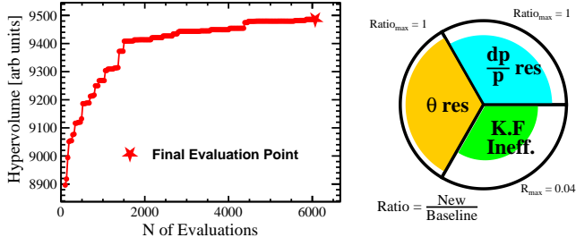
Figure 7: Metric for convergence and performance at Pareto front: (left) The hypervolume can be used as a metric for convergence. Checkpoints are created during the optimization and snapshots of the evolving designs are saved. (right) A petal diagram with the three objectives corresponding to one solution in the Pareto front. The momentum and angular resolutions are expressed as ratios with respect to a baseline design to improve; the KF inefficiency is taken as an absolute value. An optimal design optimizes all of the above defined objectives.
