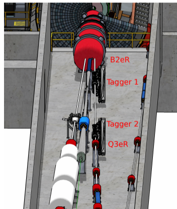
Figure: Low- Q^2 taggers
