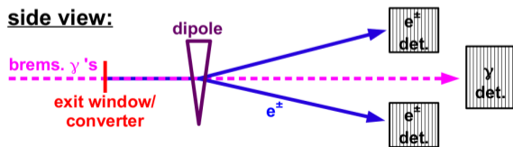
Figure: Luminosity detector
