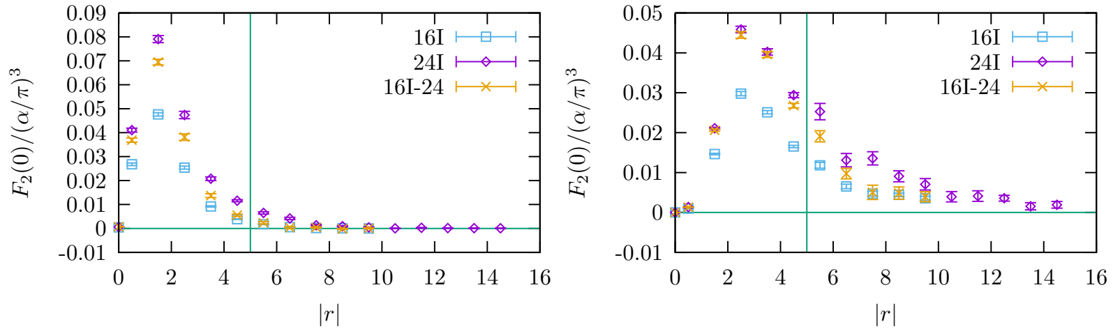
Figure 20. arXiv:1511.05198. Above plots show histograms of the contribution to F_2 from different separations |r| = |x - y| . The sum of all these points gives the final result for F_2 . The vertical lines at |r| = 5 in the plots indicate the value of r_{\max} . The left plot is evaluated with z summed over longer distance region, so the small r region includes most of the contribution. The right plot is evaluated with z summed over longer distance region, so the QCD finite volume is better controlled in the small r region.
