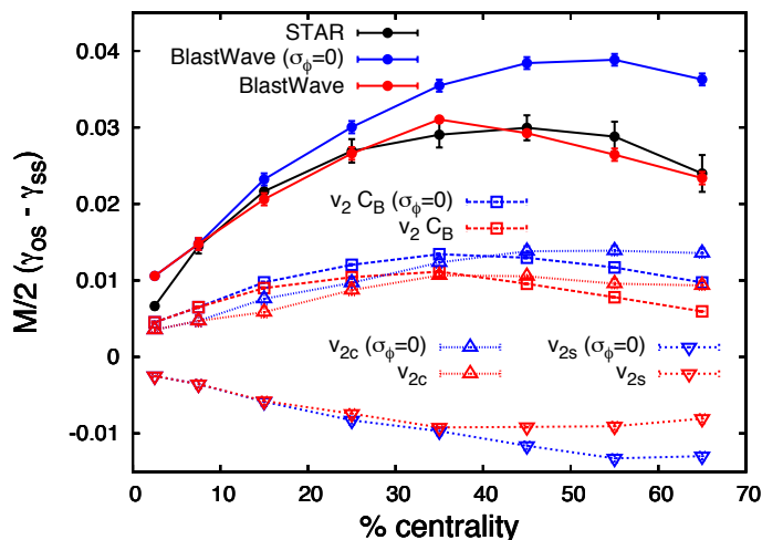
FIG. 4: Model calculations (Blast-Wave) demonstrating that the contribution of local charge conservation coupled with flow can mimic the observed charge separation observed by STAR [30]. This indicates that background effects may account for a large fraction or all of the observed charge separation signal.
