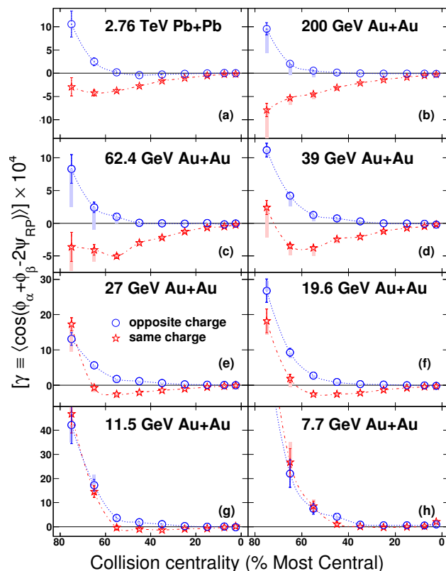
FIG. 2: Charge separation measurements as a function of centrality for 8 collisions energies spanning 7.7 GeV to 2.76 TeV.
