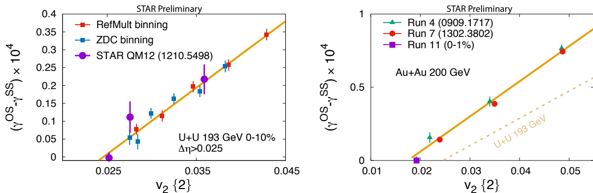
FIG. 3: Charge separation as a function of v_2 for various centrality selections within the 0-10% centrality range in U+U collisions (left) and Au+Au collisions (right).
