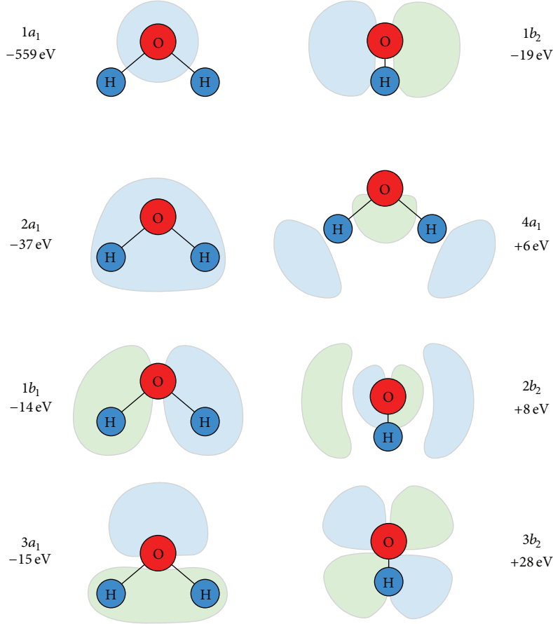
FIGURE 2: The five occupied (negative electron binding energy) and lowest three unoccupied (positive electron binding energy) molecular orbitals of an isolated water molecule. Calculated using the restricted Hartree-Fock wave function [34].
