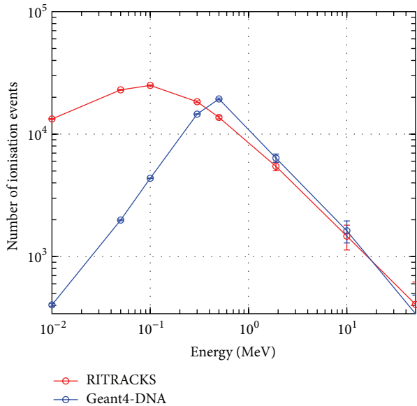
FIGURE 7: Total number of ionisation events recorded in a 7 \mu\text{m} \times 7 \mu\text{m} \times 7 \mu\text{m} water box from the passage of a single proton and secondary electrons in liquid water using Geant4-DNA and RITRACKS.
