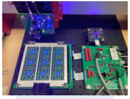
Nine SiPM Daughterboards for EMCal under test; total of 144 SiPMs
