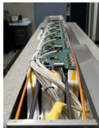
EMCal Sector (96 Towers) with PreAmps, Interface Boards and Cabling Mounted
