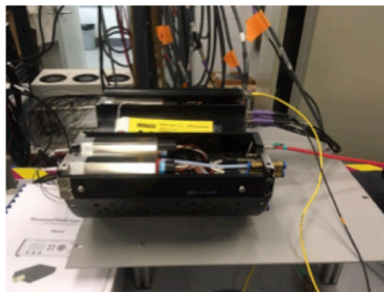
One MBD Section under test
