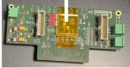
Test board with EIC- ROC0
