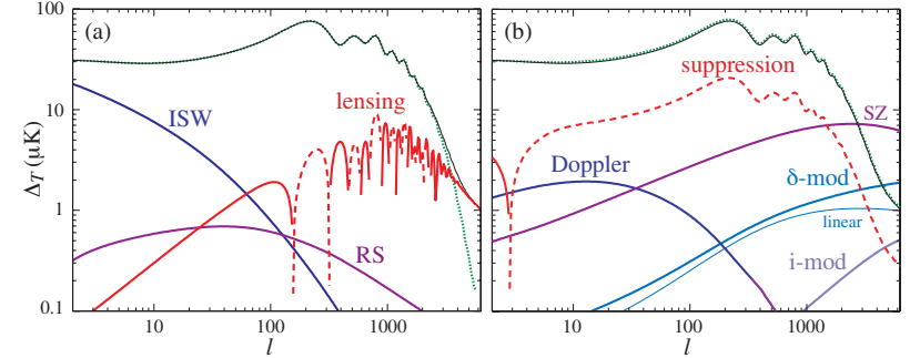
Plate 5: Secondary anisotropies. (a) Gravitational secondaries: ISW, lensing and Rees-Sciama (moving halo) effects. (b) Scattering secondaries: Doppler, density ( \delta ) and ionization ( i ) modulated Doppler, and the SZ effects. Curves and model are described in the text.
