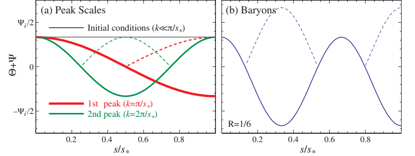
Figure 1: Idealized acoustic oscillations. (a) Peak scales: the wavemode that completes half an oscillation by recombination sets the physical scale of the first peak. Both minima and maxima correspond to peaks in power (dashed lines, absolute value) and so higher peaks are integral multiples of this scale with equal height. Plotted here is the idealization of Equation (15) (constant potentials, no baryon loading). (b) Baryon loading. Baryon loading boosts the amplitudes of every other oscillation. Plotted here is the idealization of Equation (16) (constant potentials and baryon loading R = 1/6 ) for the third peak.
