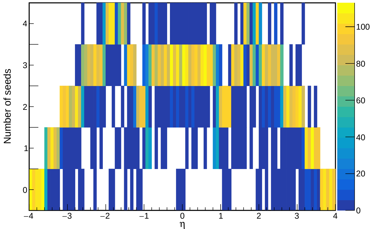
Number of seeds vs. generated particle \eta
