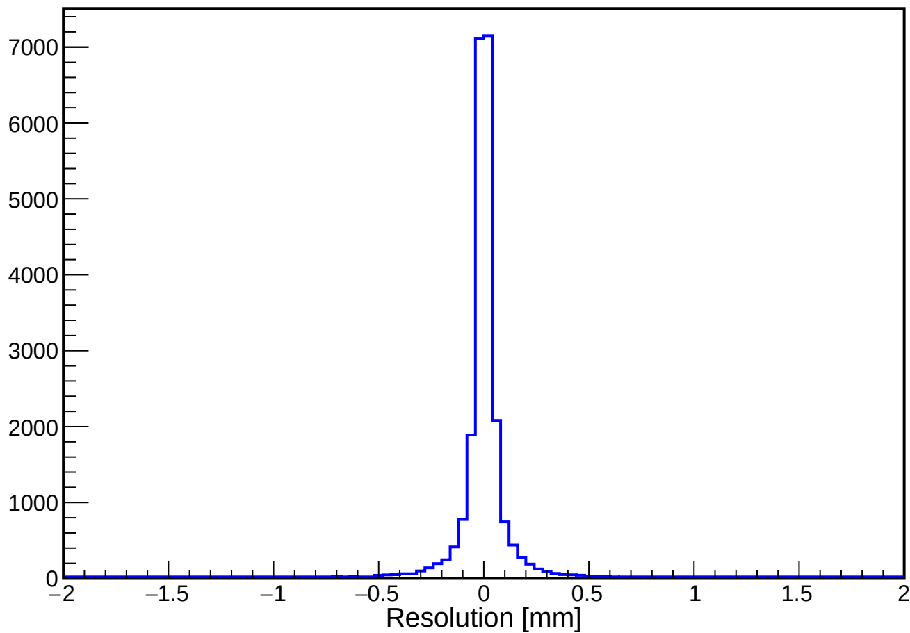
Seed ACTS loc-a Resolution: (seed - true)
