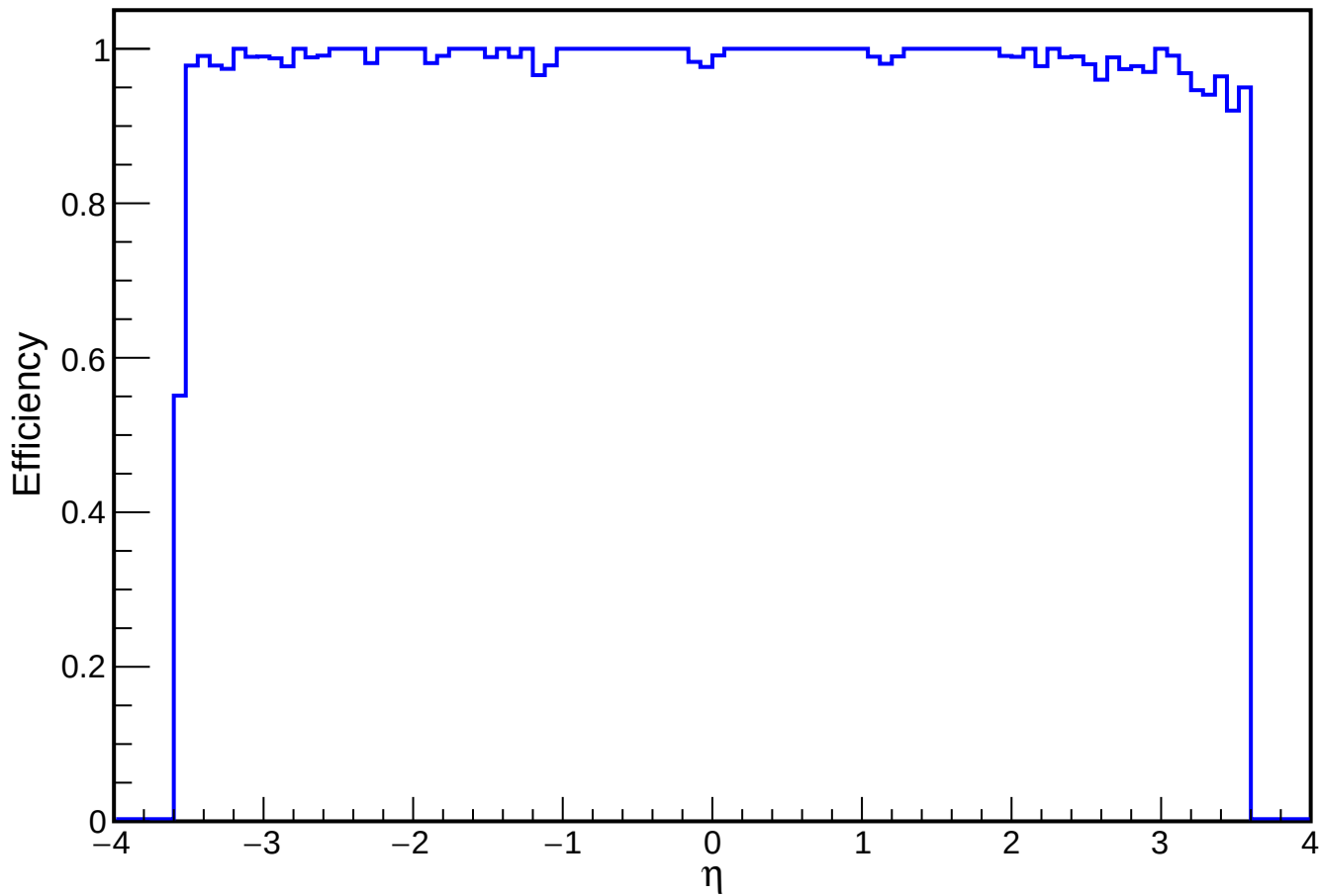
Seeder Efficiency vs. generated particle \eta
