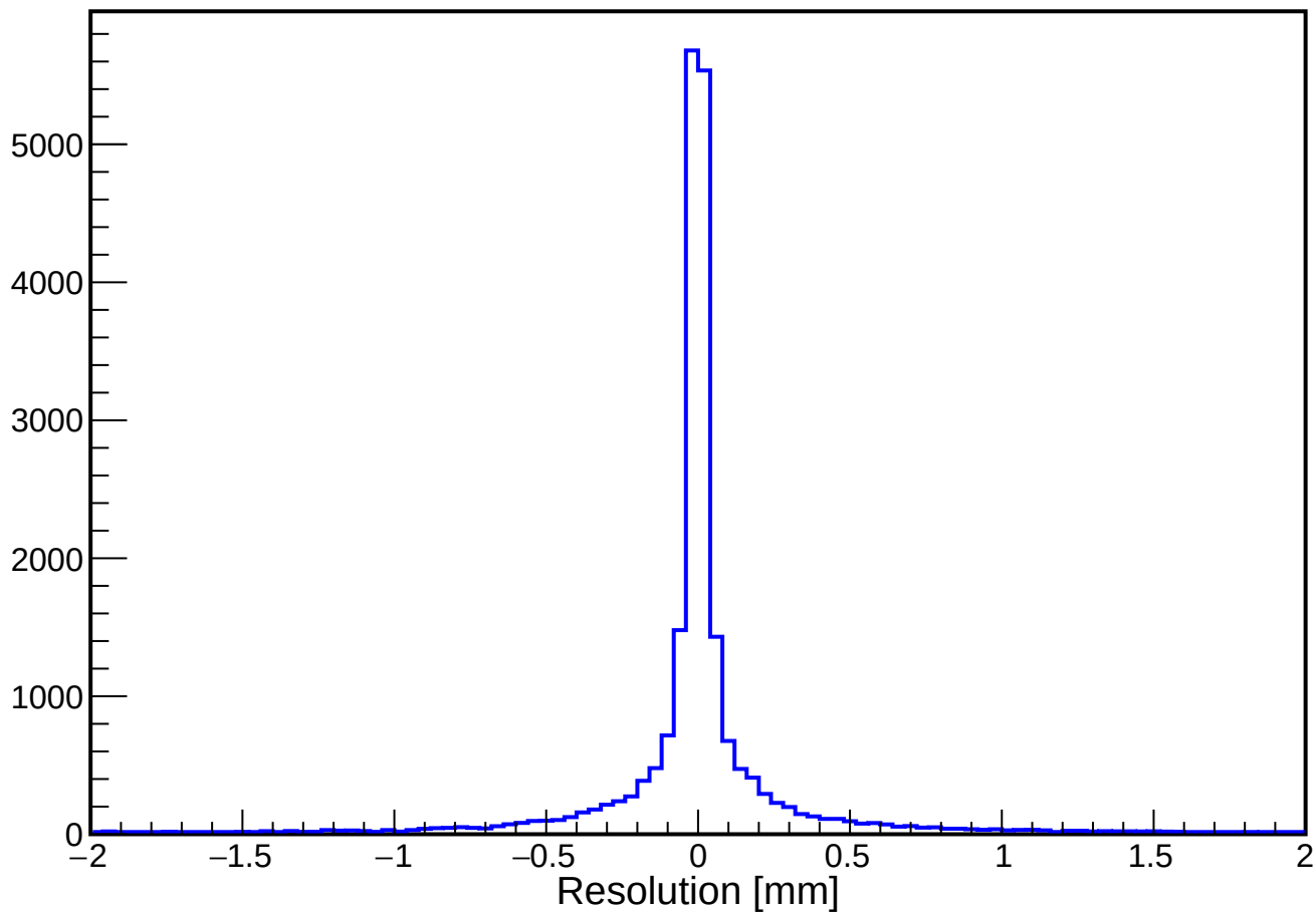
Seed ACTS loc-b Resolution: (seed - true)
