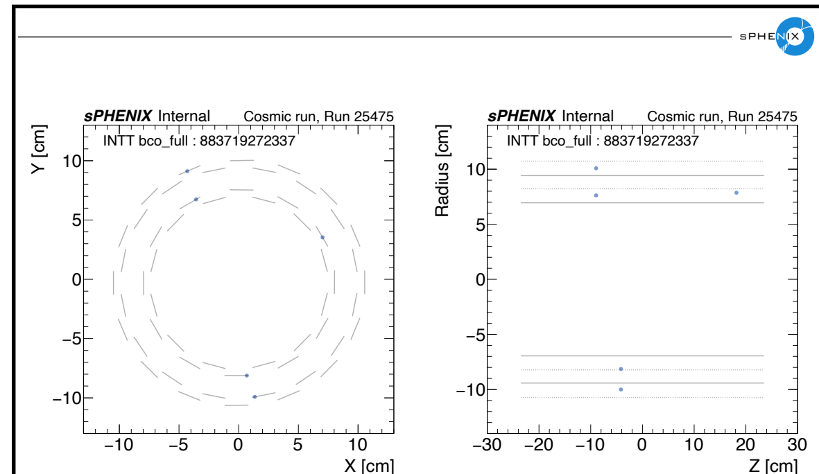
Figure 4: The 2-dimensional event display of the event with BCO 883719272337: (Left) The cluster position in X-Y plane. (Right) The cluster position in Z-Radius plane.
