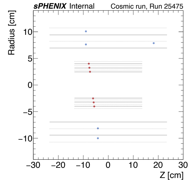
Figure 7: The 2-dimensional event display of MVTX and INTT of the event with INTT BCO 883719272337: (Left) The cluster position and size in X-Y plane. (Right) The cluster position and size in Z-Radius plane.
