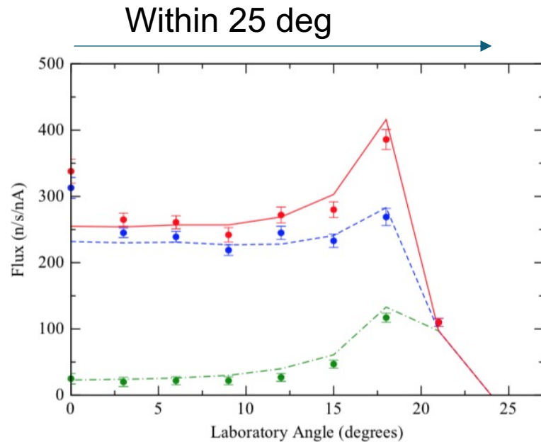
Angular distribution of neutron flux
