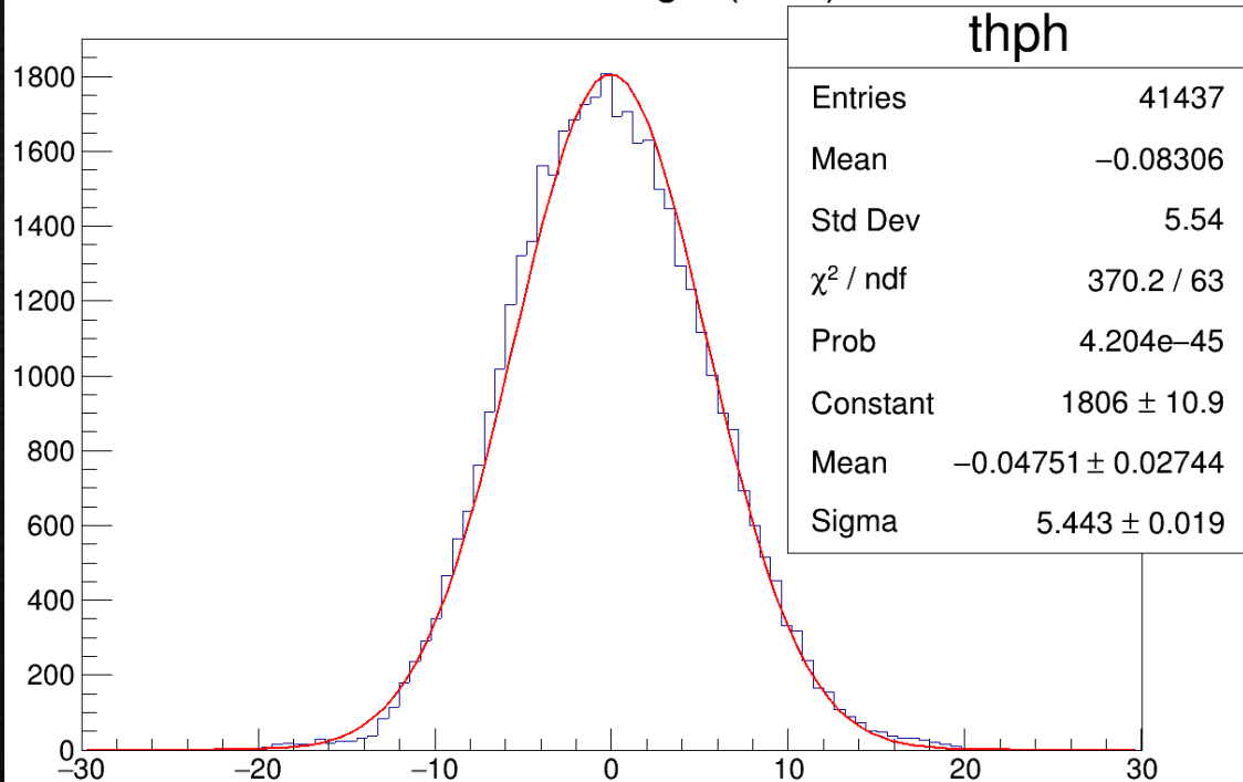
Cherenkov angle (SPE)
