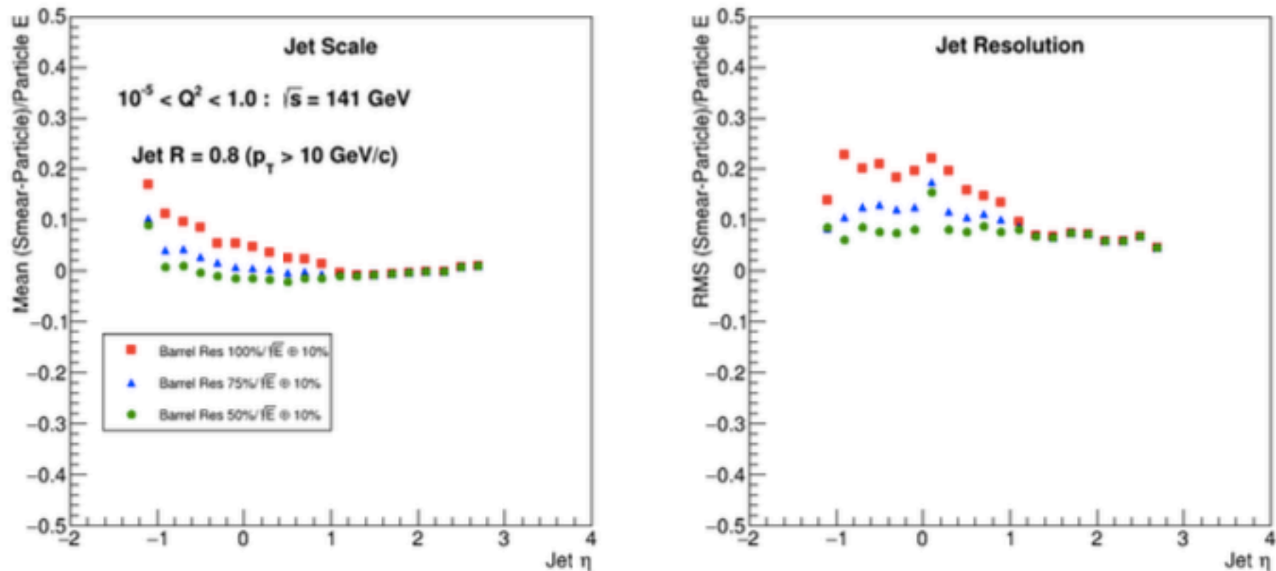
Figure 8.56: Jet energy scale (left) and resolution (right) as a function of jet pseudorapidity when selecting smeared jets with p_T > 10 GeV/c for different values of HCal energy resolution: 100\%/\sqrt{E} \oplus 10\% (red squares), 75\%/\sqrt{E} \oplus 10\% (blue triangles), and 50\%/\sqrt{E} \oplus 10\% (green circles).
