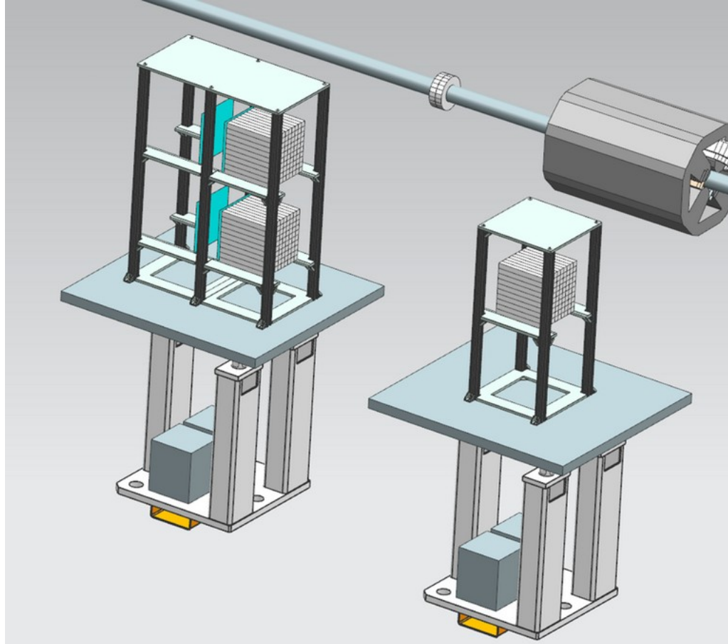
PS and Direct- \gamma CAL on separate tables
