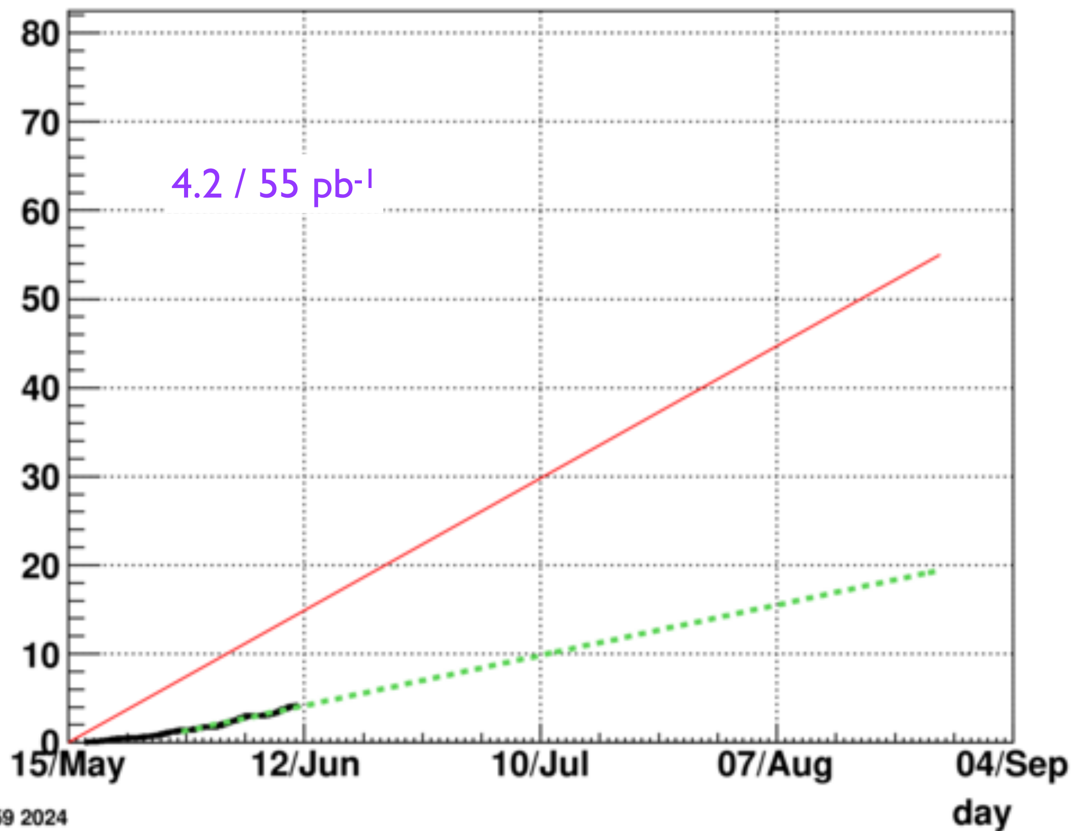
P^2 L [ \text{pb}^{-1} ]
