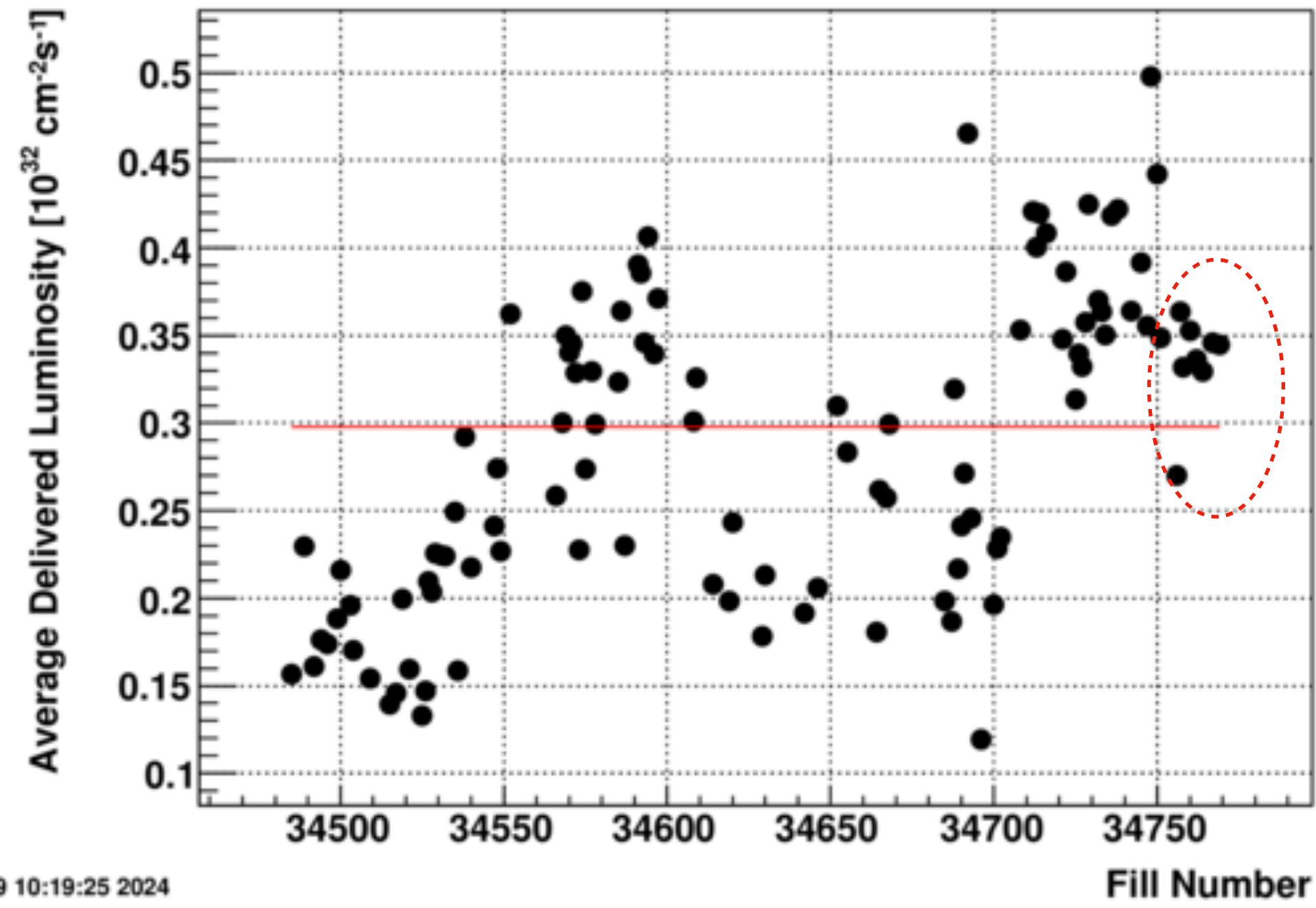
Average Delivered Luminosity [ 10^{32} \text{ cm}^{-2} \text{ s}^{-1} ]
