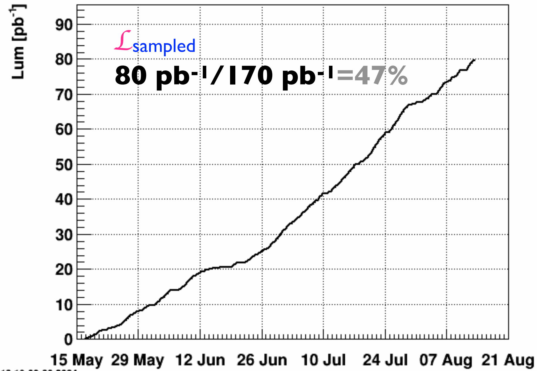
JP2-effective
