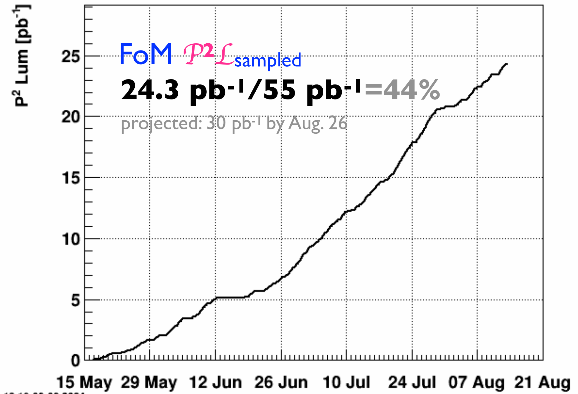
JP2-effective
