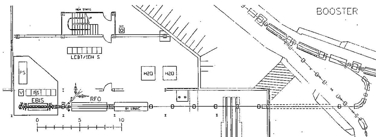
Figure 4-3 Placement of EBIS Pre-Injector in lower equipment bay of 200 MeV Linac.
