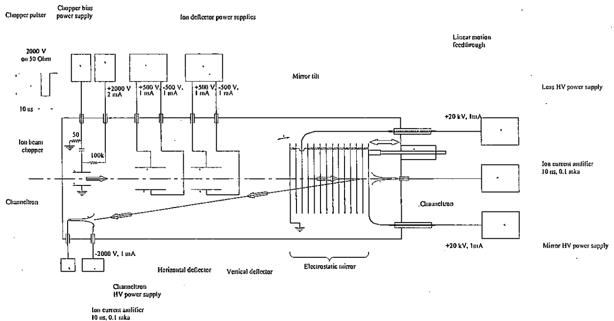
Figure 5-51 Schematic of the Mamyrin time-of-flight diagnostic.
