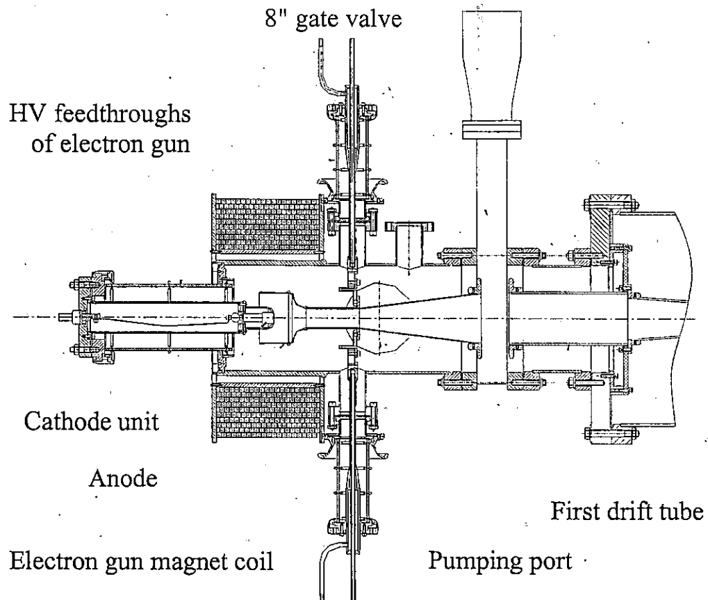
Figure 4-4 Electron Gun Assembly
