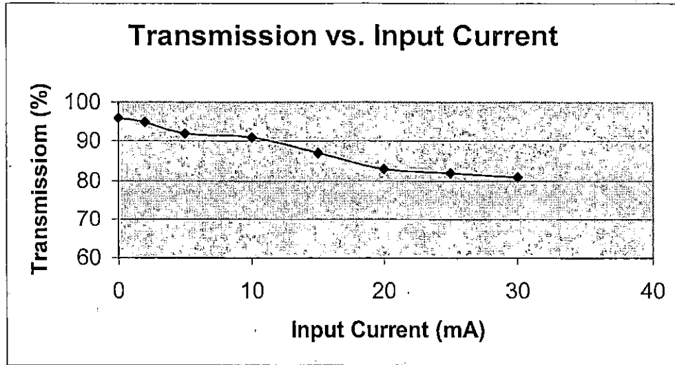
Figure 5-28 RFQ transmission vs. input current for Au +32 .
