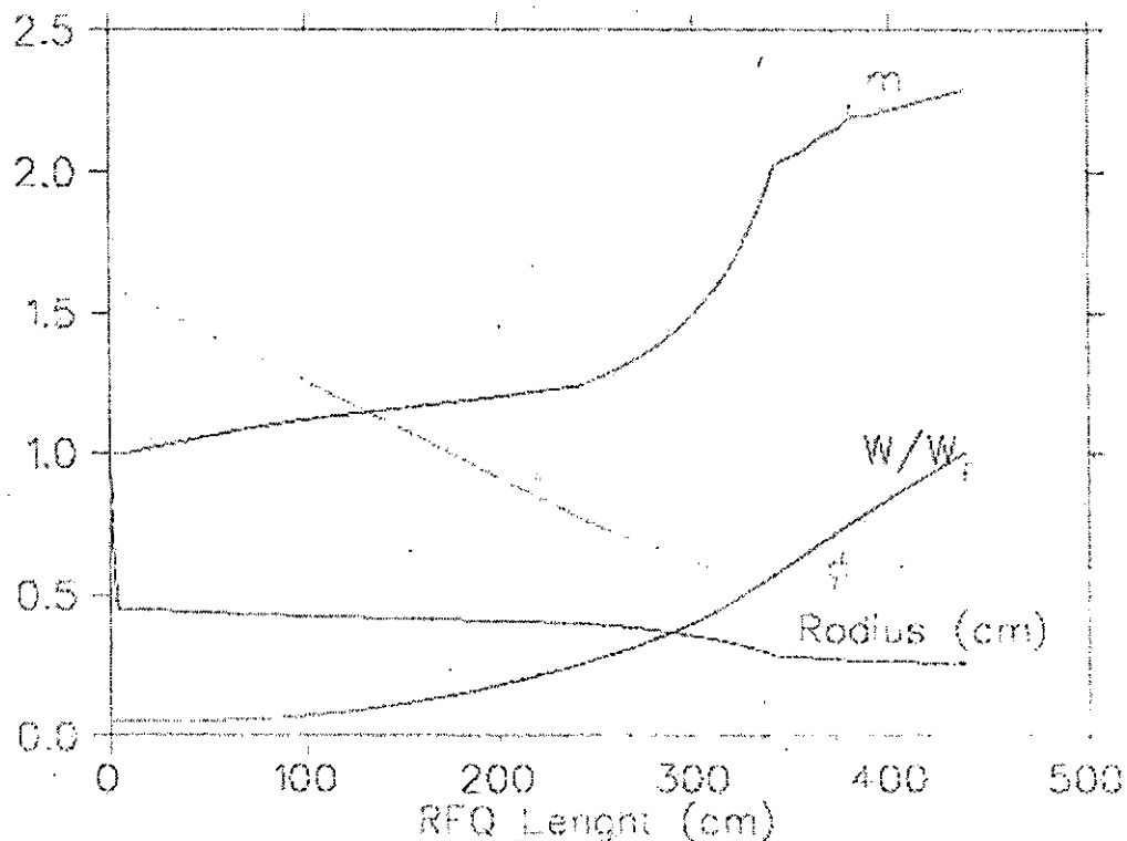
Figure 5-22 Optics design parameters for the RFQ
