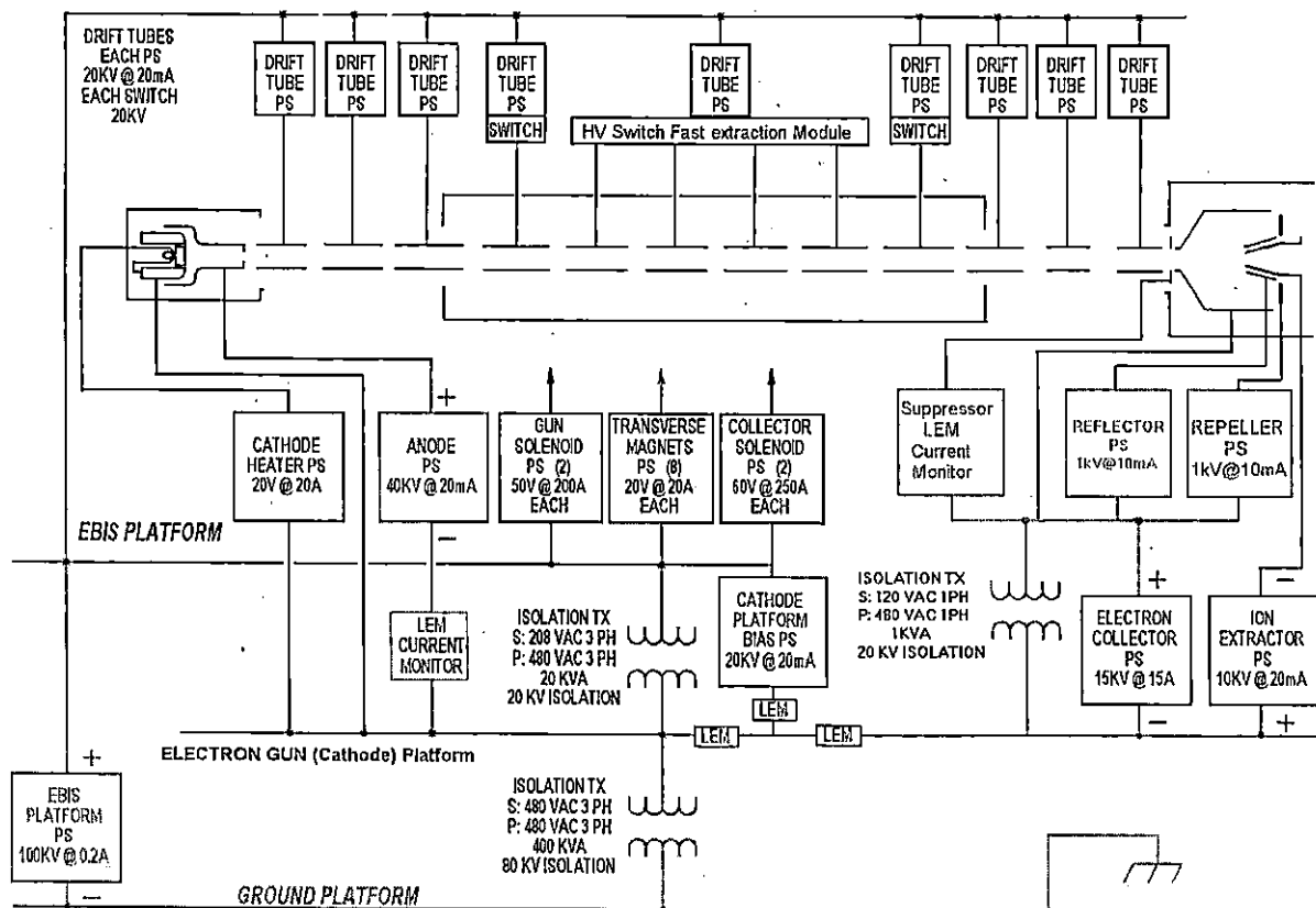
Figure 5-15 Schematic of the EBIS voltage platforms
