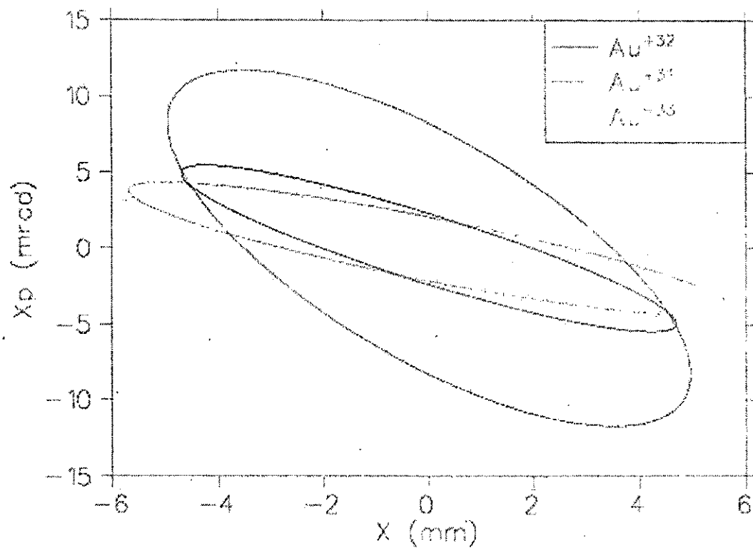
Figure 5-38 Phase space (X-XP) plots for different charge states of Au at end of Linac.
