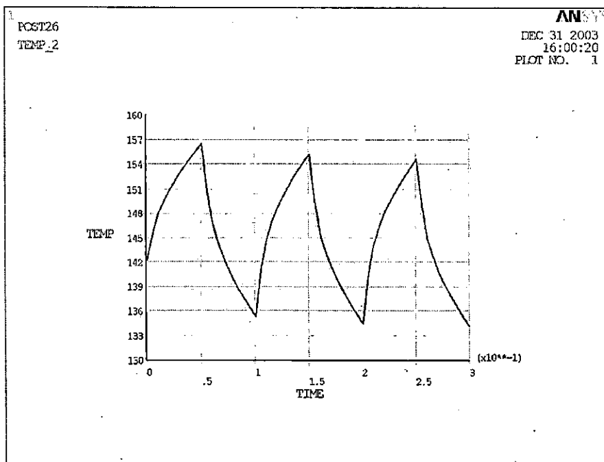
Figure 5-9 Temperature cycling at the hottest node of the EC in equilibrium of medium temperature. (20A, 15 keV, 50 ms on, 50 ms off)
