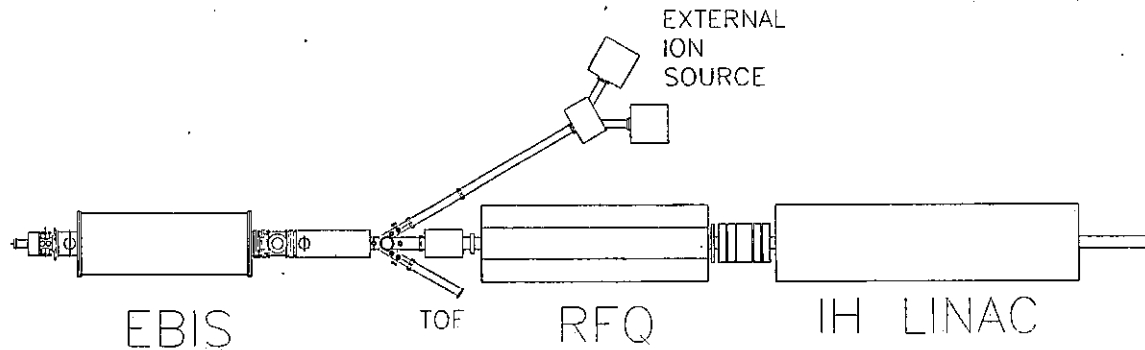
Figure 4-1 Conceptual layout of the pre-injector
