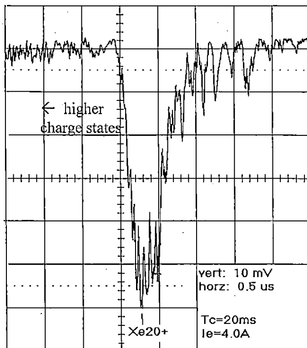
Figure 4-10 \text{Xe}^{20+} produced using a 4A, electron beam and a confinement time of 20ms.
