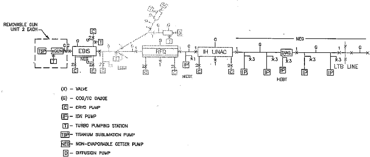
Figure 5-54 Schematic of the vacuum system
