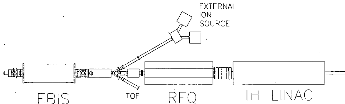
Figure 5-2 Conceptual layout of the pre-injector
