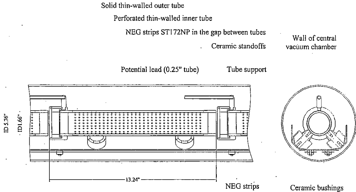
Figure 5-12 Central drift tube (ionization region).
