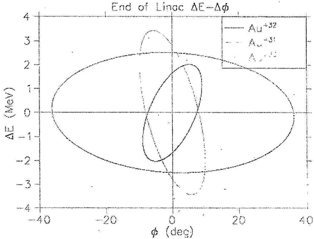
Figure 5-40 Phase space ( \Delta E - \Delta\phi ) plots for different charge states of Au at end of Linac.
