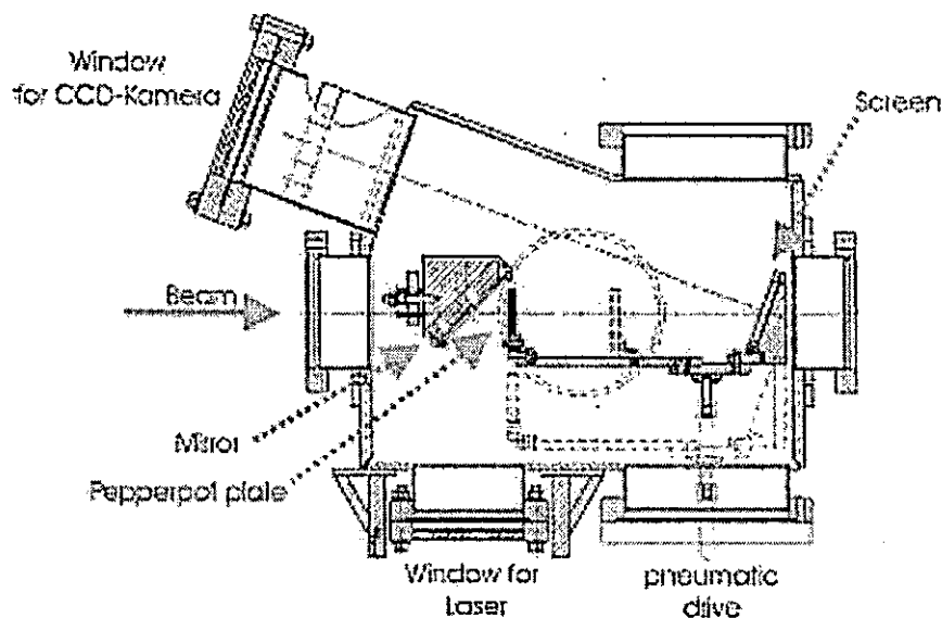
Figure 5-52 Drawing of pepper-pot emittance device and laser calibration system used at GSI. 17
