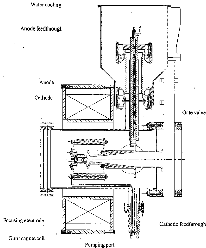
Figure 5-4. Replaceable electron gun unit of RHIC EBIS.
