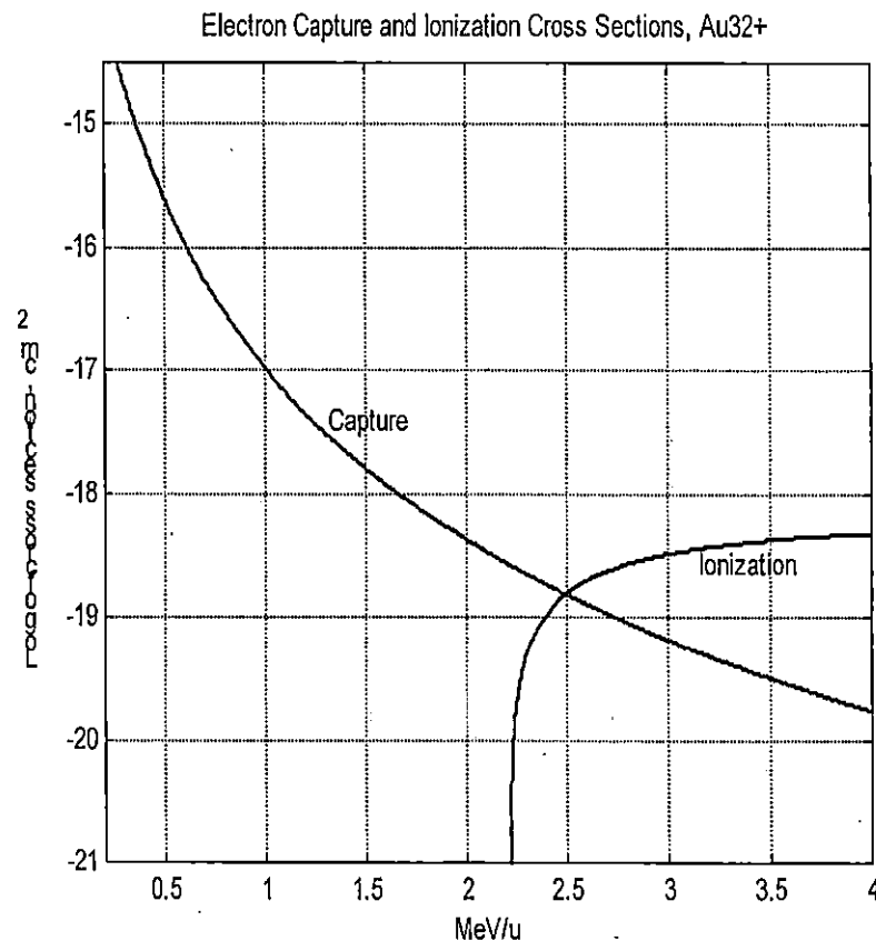
Figure 5-48 Electron capture and ionization cross-sections, for Au 32+ .
