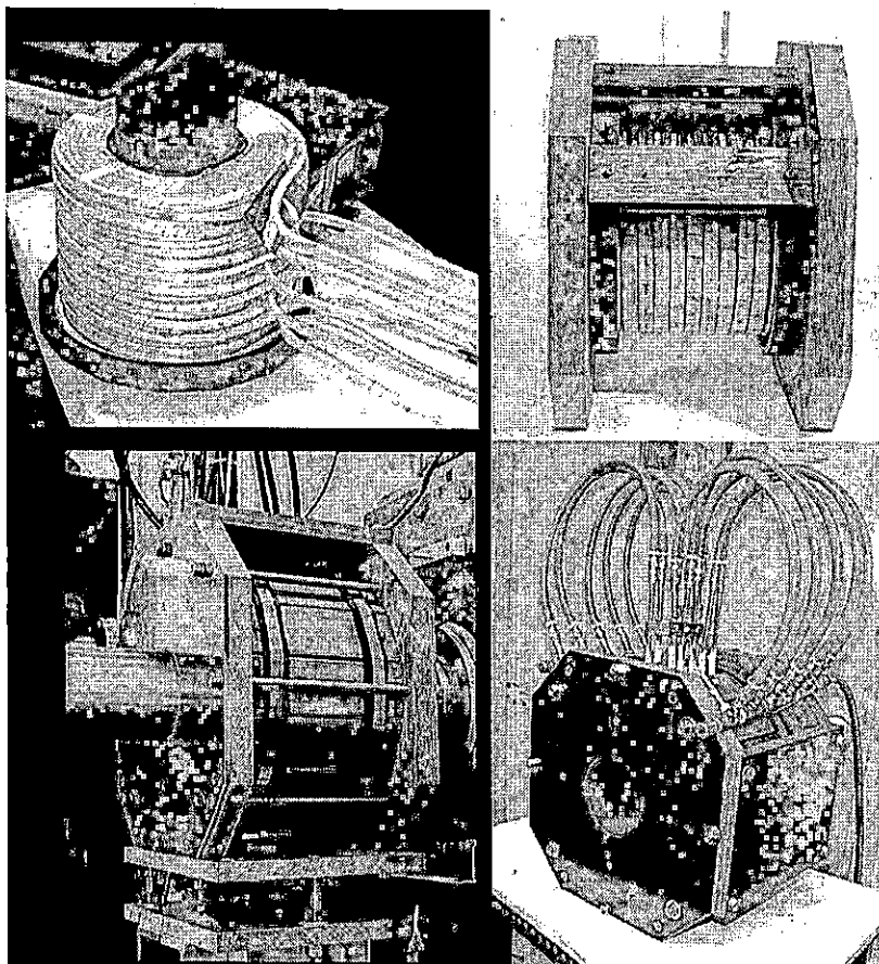
Figure 5-53 Photos showing construction of the H- LEBT solenoid.
