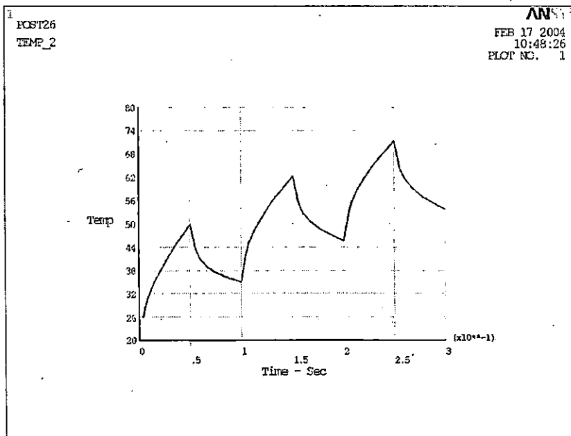
Figure 5-7 Temperature cycling in the hottest node at the beginning of the power load (20A, 15 keV, 50 ms on, 50 ms off).
