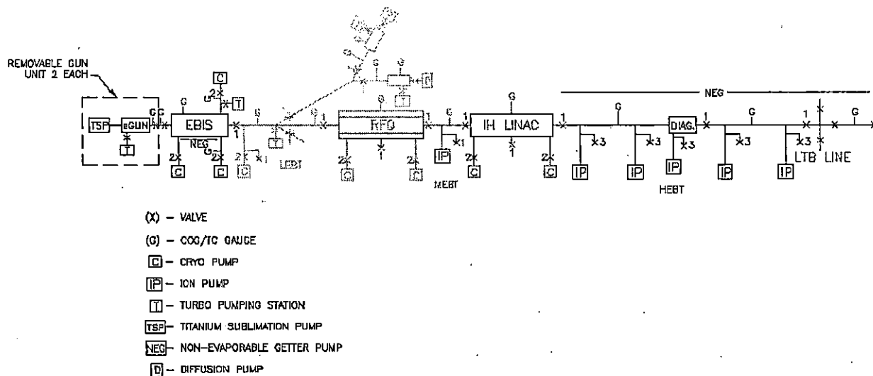
Figure 4-2 Schematic of the vacuum system.
