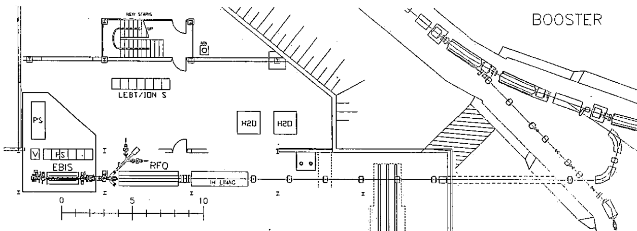
Figure 5-41 Schematic showing the pre-injector in the lower equipment bay of the 200 MeV Linac.
