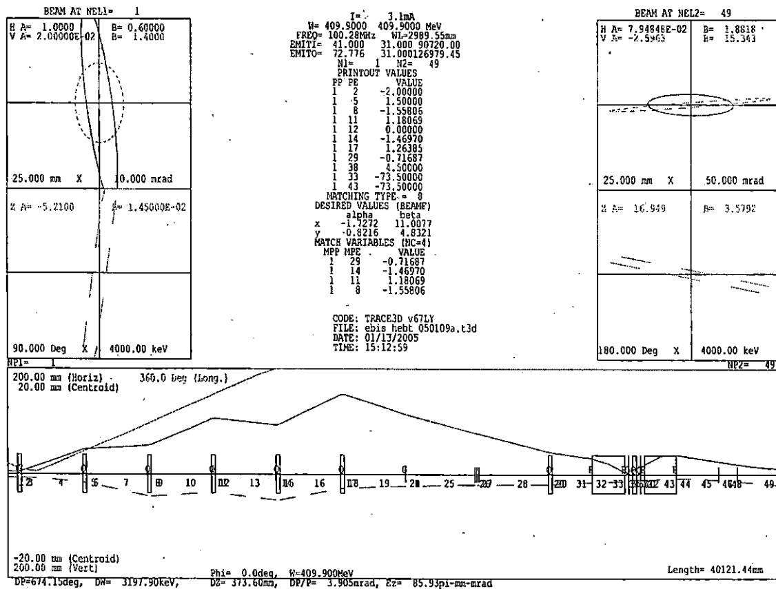
Figure 5-43 Beam envelope (TRACE3D) through the HEBT for Au +31 .
