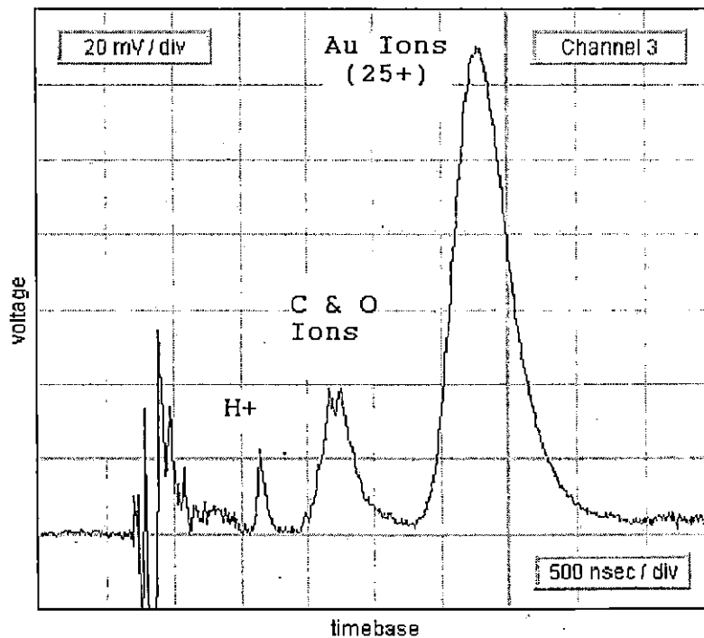
Figure 4-12 Inline Time-of-Flight spectrum showing Au=83%; C&O=15%; H=2%
