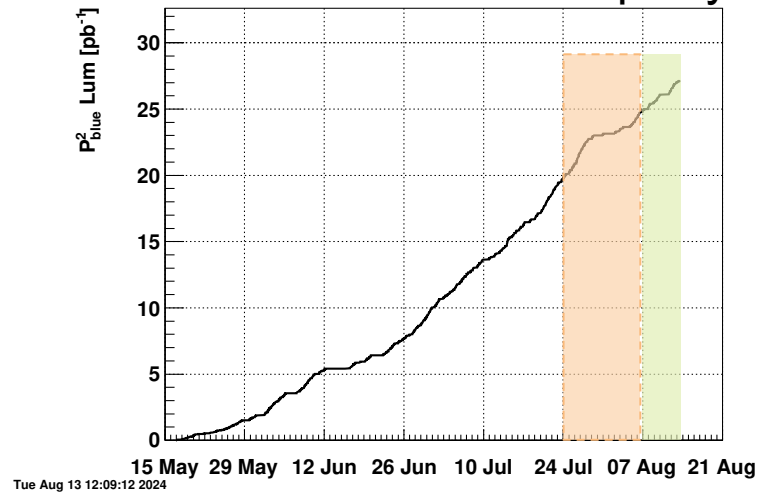
fcsJPsiAsy
