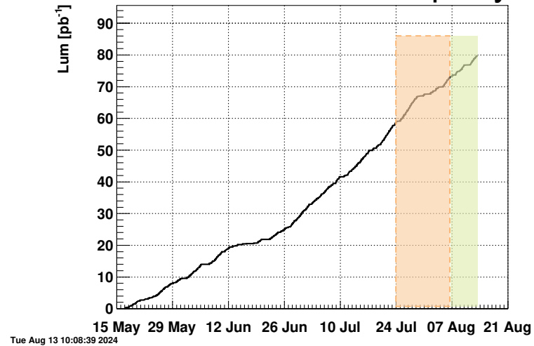
fcsJPsiAsy
