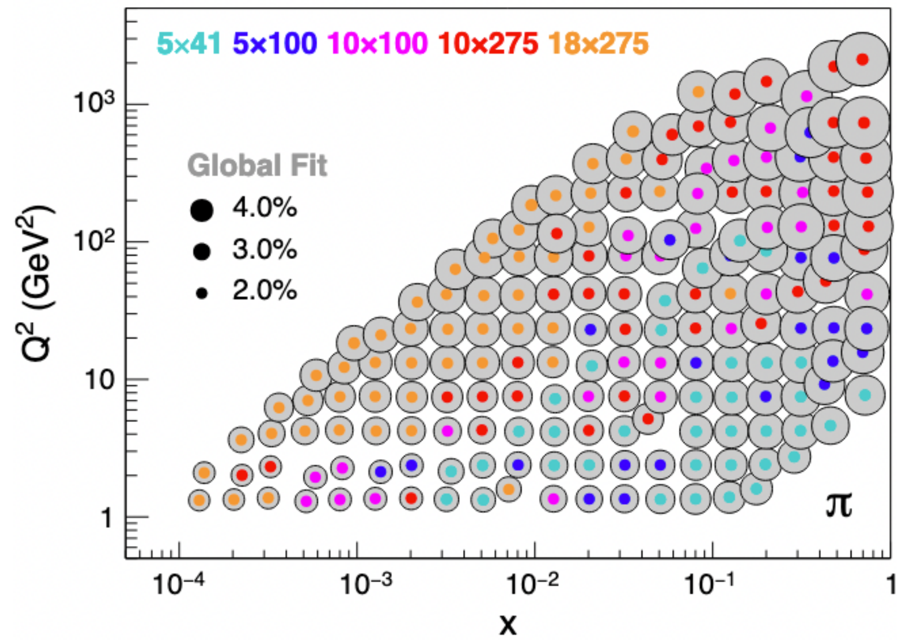
Unpolarised TMDs
