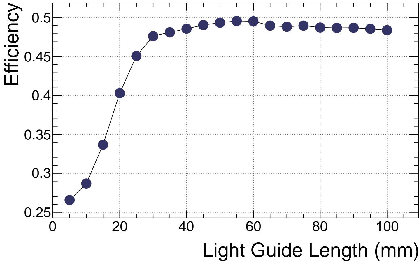
b7 air S13-BIC Efficiency vs. Length
