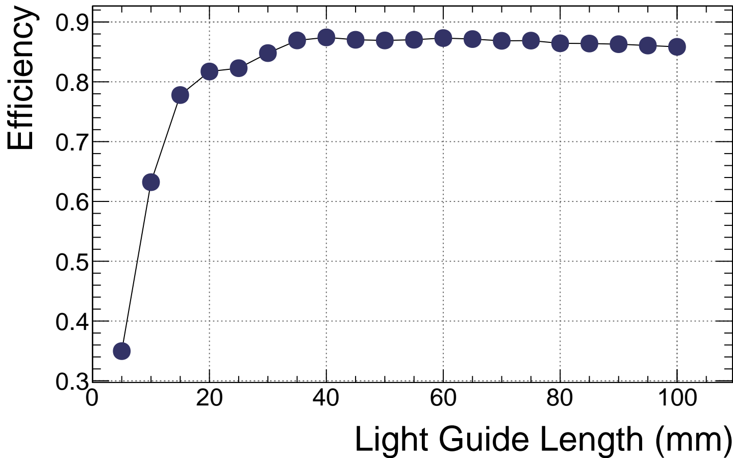
b3 cookie S13-BIC Efficiency vs. Length
