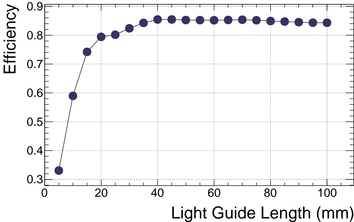
b4 cookie S13-BIC Efficiency vs. Length
