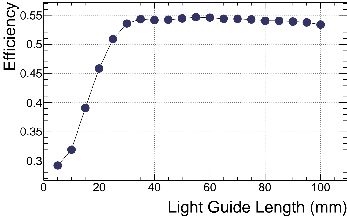
b3 air S13-BIC Efficiency vs. Length
