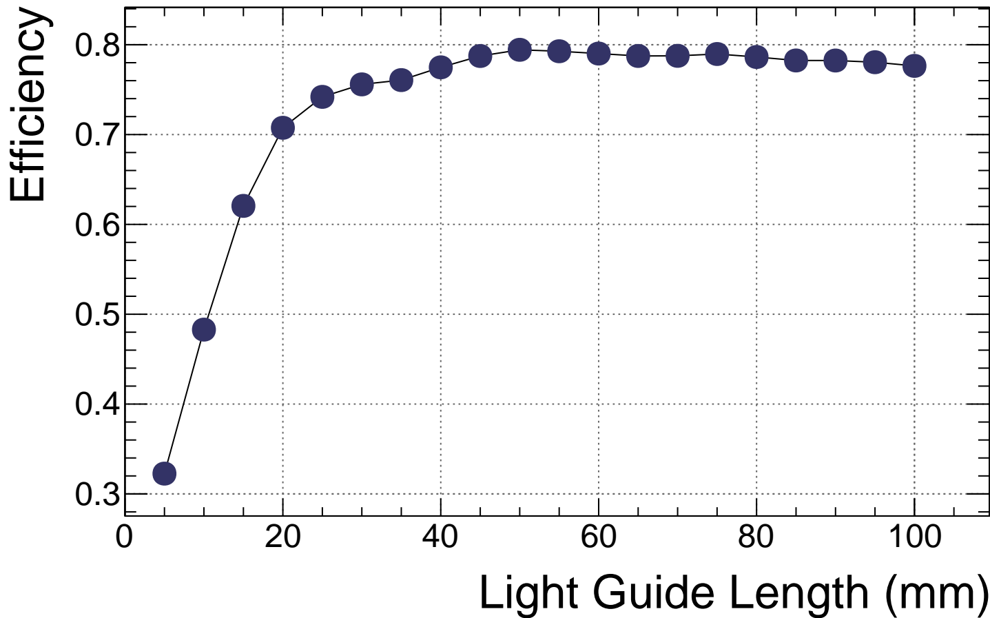
b9 cookie S13-BIC Efficiency vs. Length
