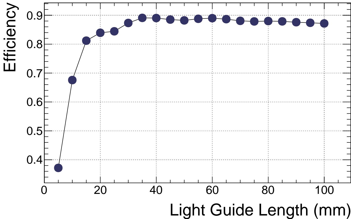
b2 cookie S13-BIC Efficiency vs. Length
