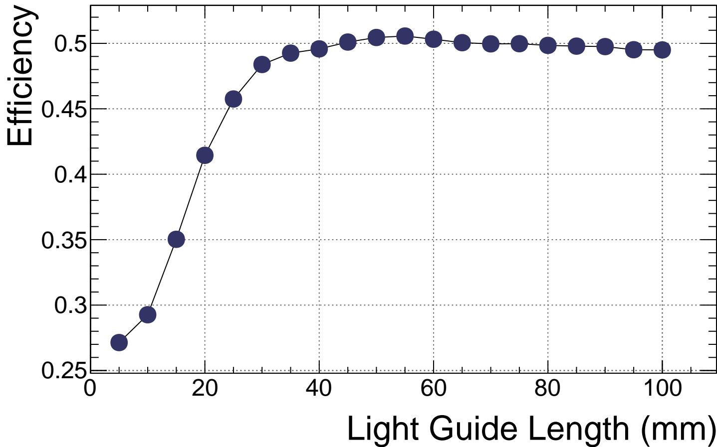
b6 air S13-BIC Efficiency vs. Length
