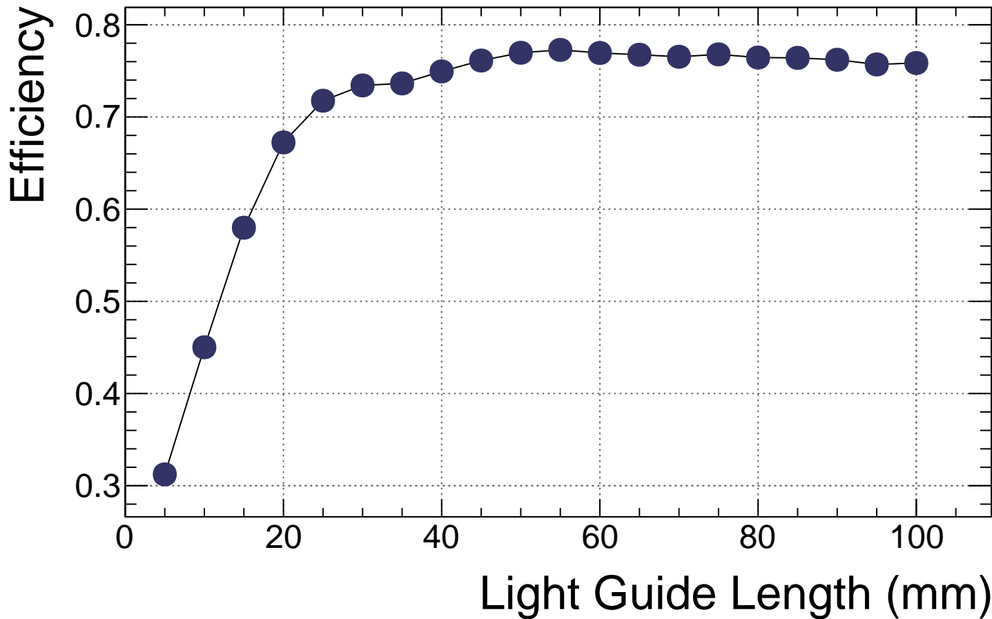
b11 cookie S13-BIC Efficiency vs. Length
