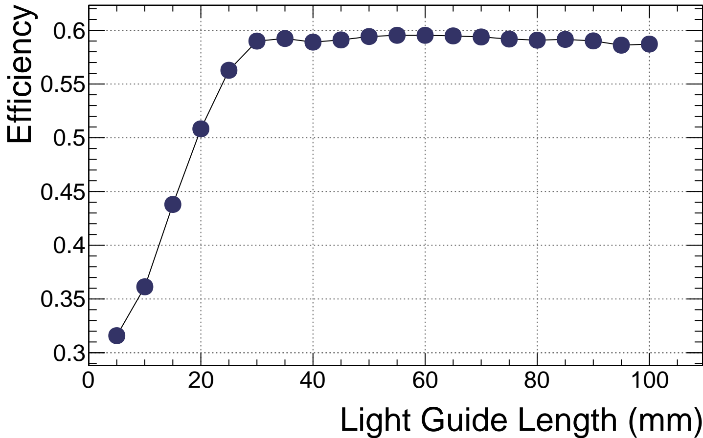
b1 air S13-BIC Efficiency vs. Length
