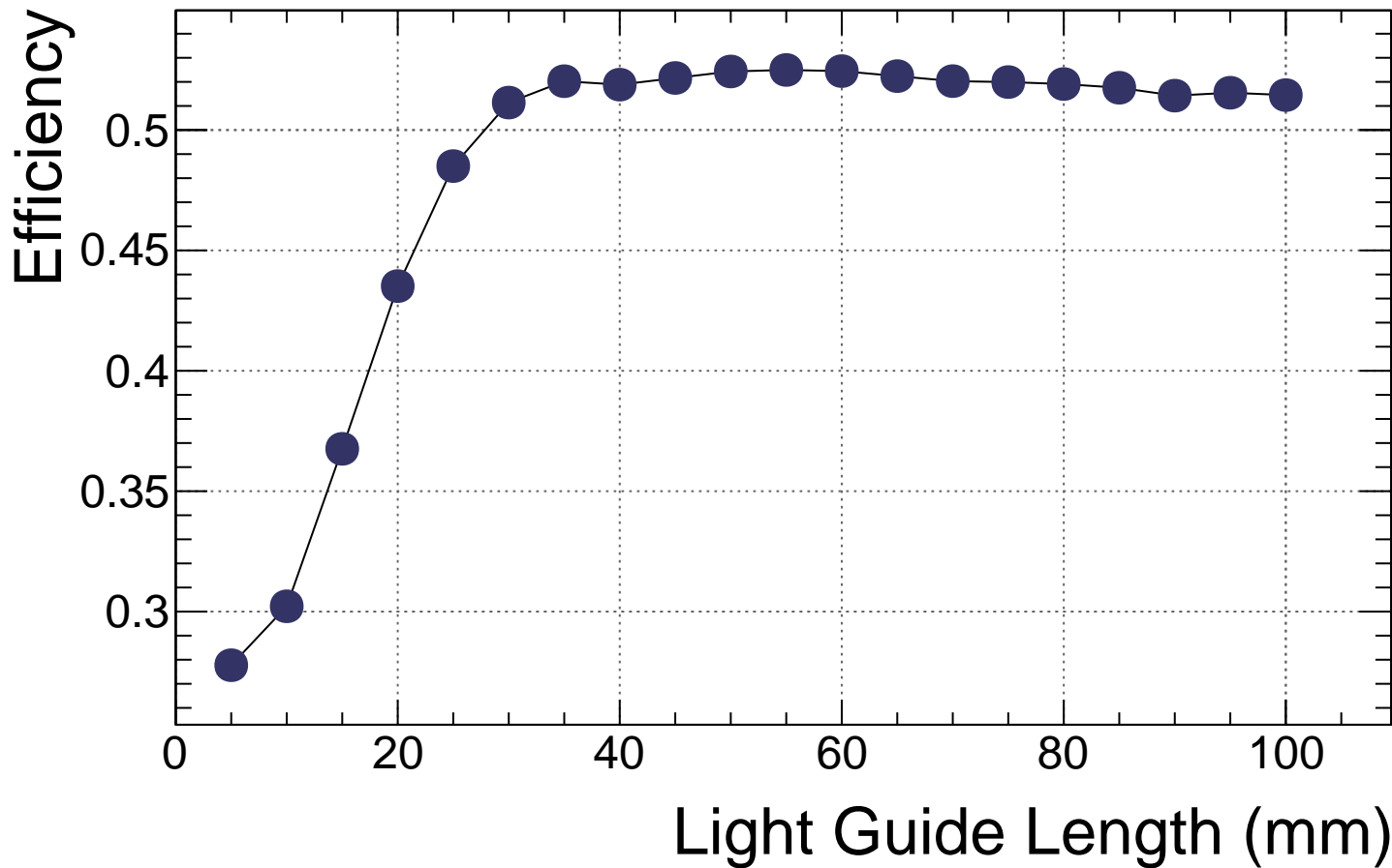
b4 air S13-BIC Efficiency vs. Length
