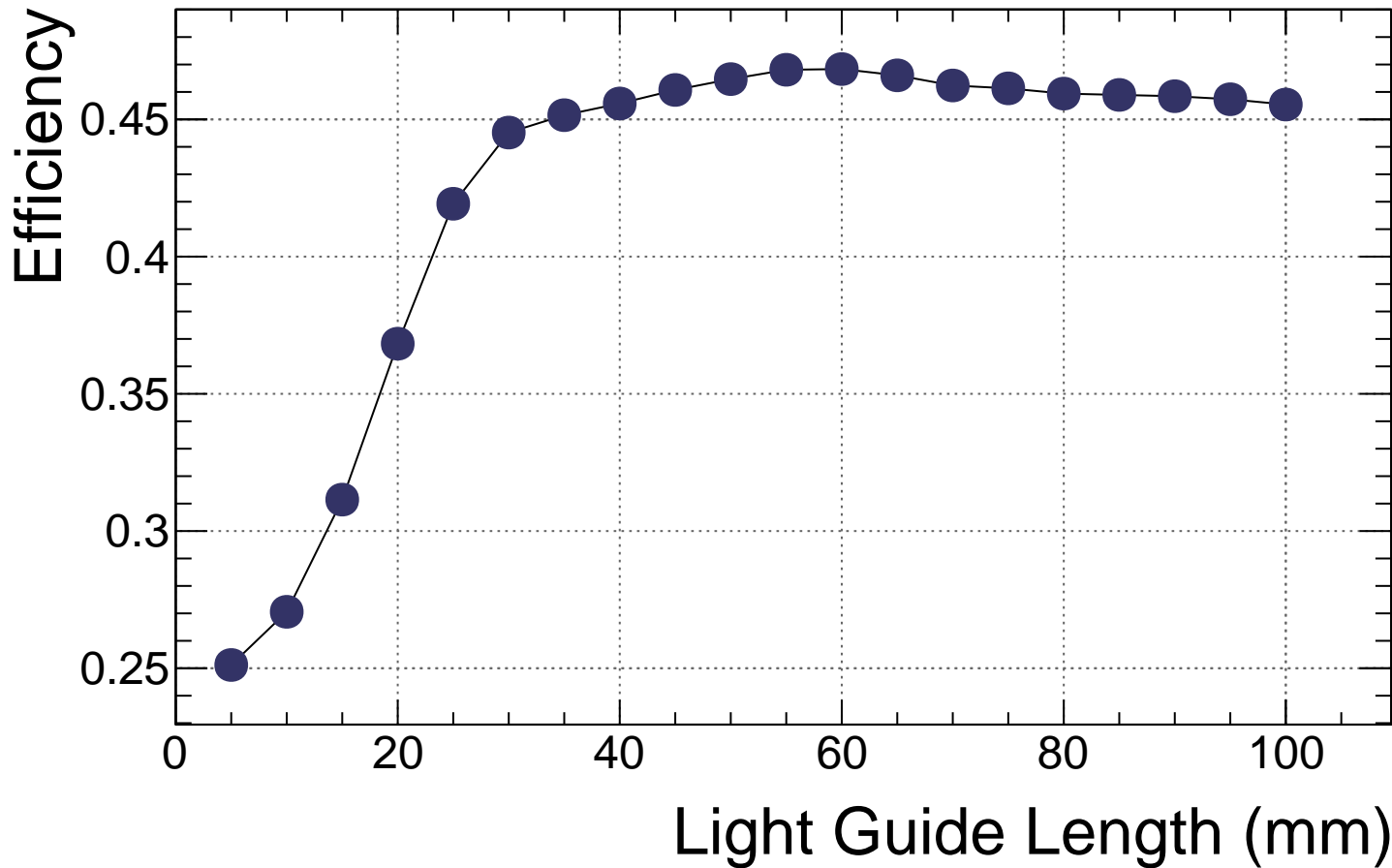
b10 air S13-BIC Efficiency vs. Length
