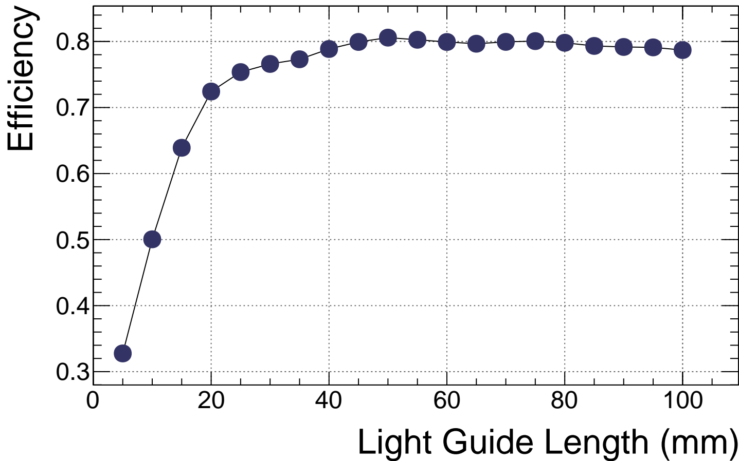
b8 cookie S13-BIC Efficiency vs. Length
