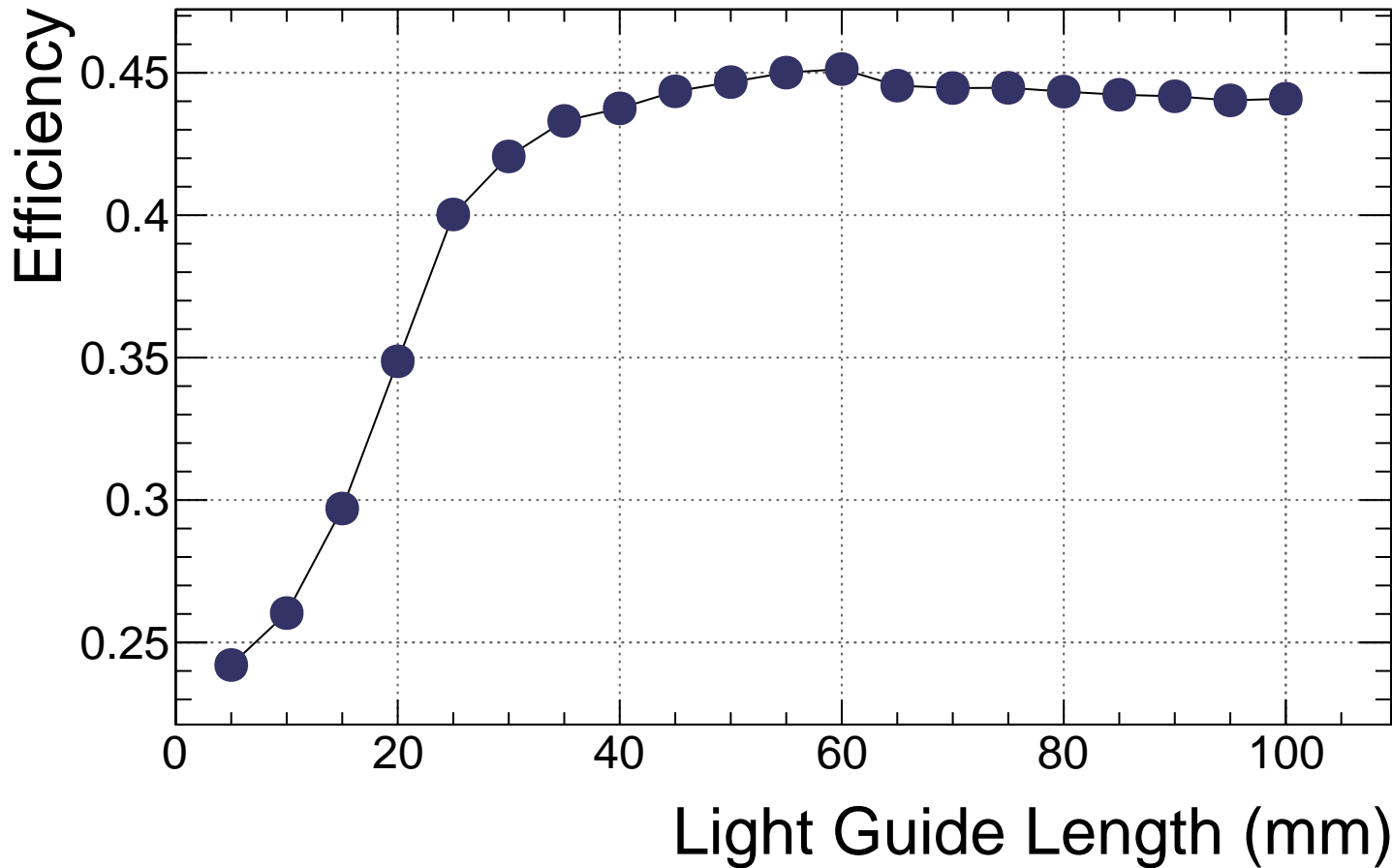
b12 air S13-BIC Efficiency vs. Length
