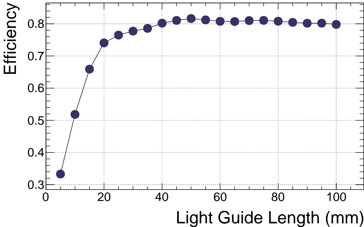
b7 cookie S13-BIC Efficiency vs. Length
