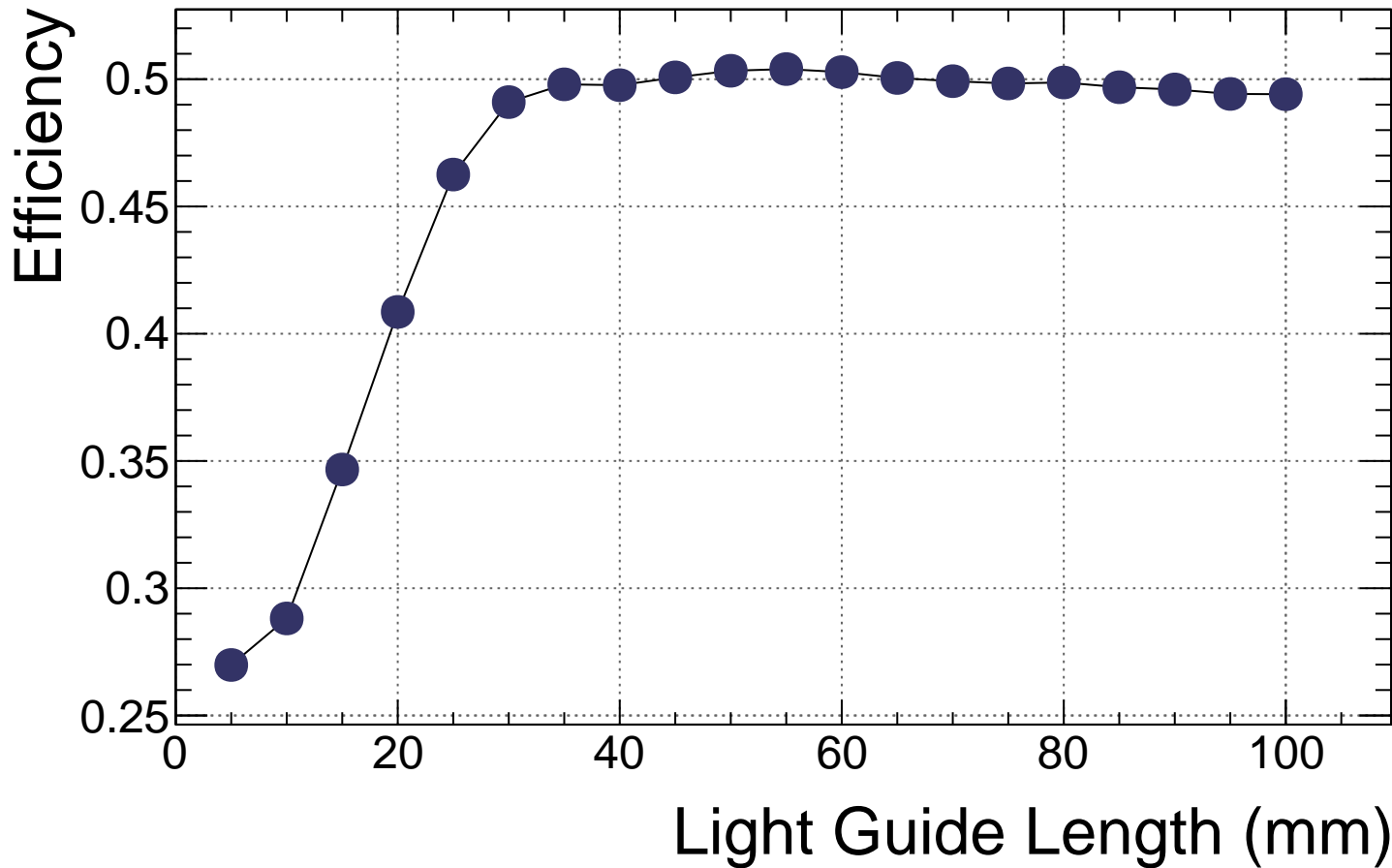
b5 air S13-BIC Efficiency vs. Length
