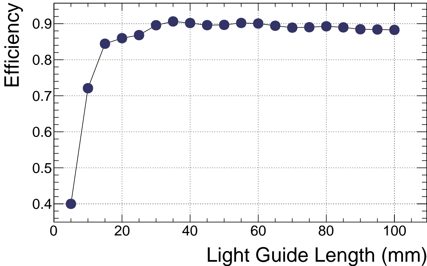
b1 cookie S13-BIC Efficiency vs. Length
