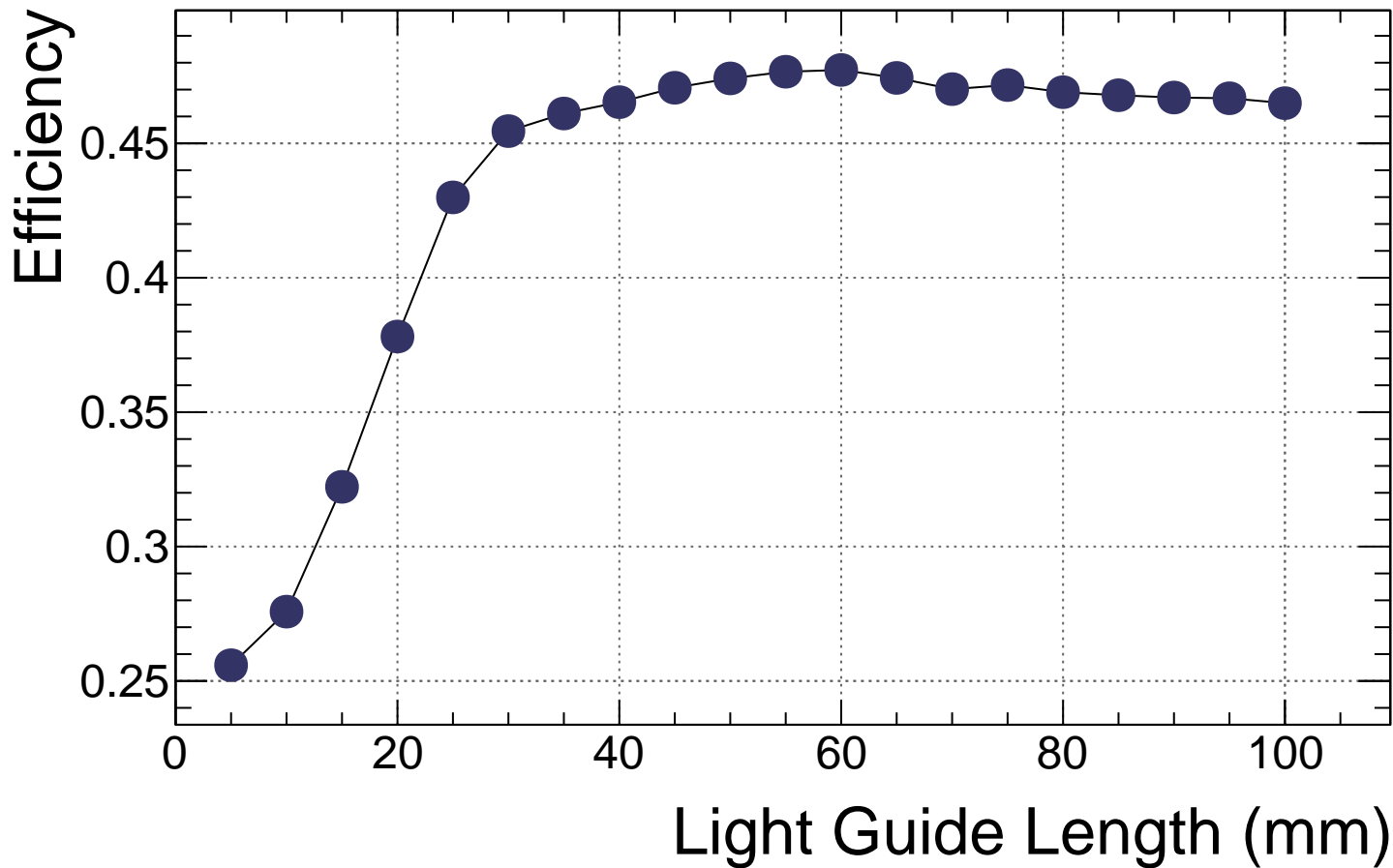
b9 air S13-BIC Efficiency vs. Length
