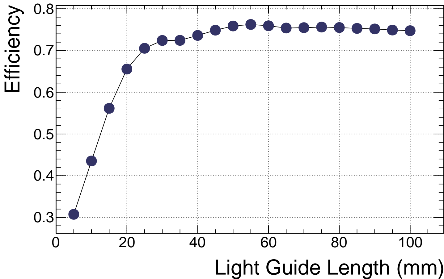
b12 cookie S13-BIC Efficiency vs. Length
