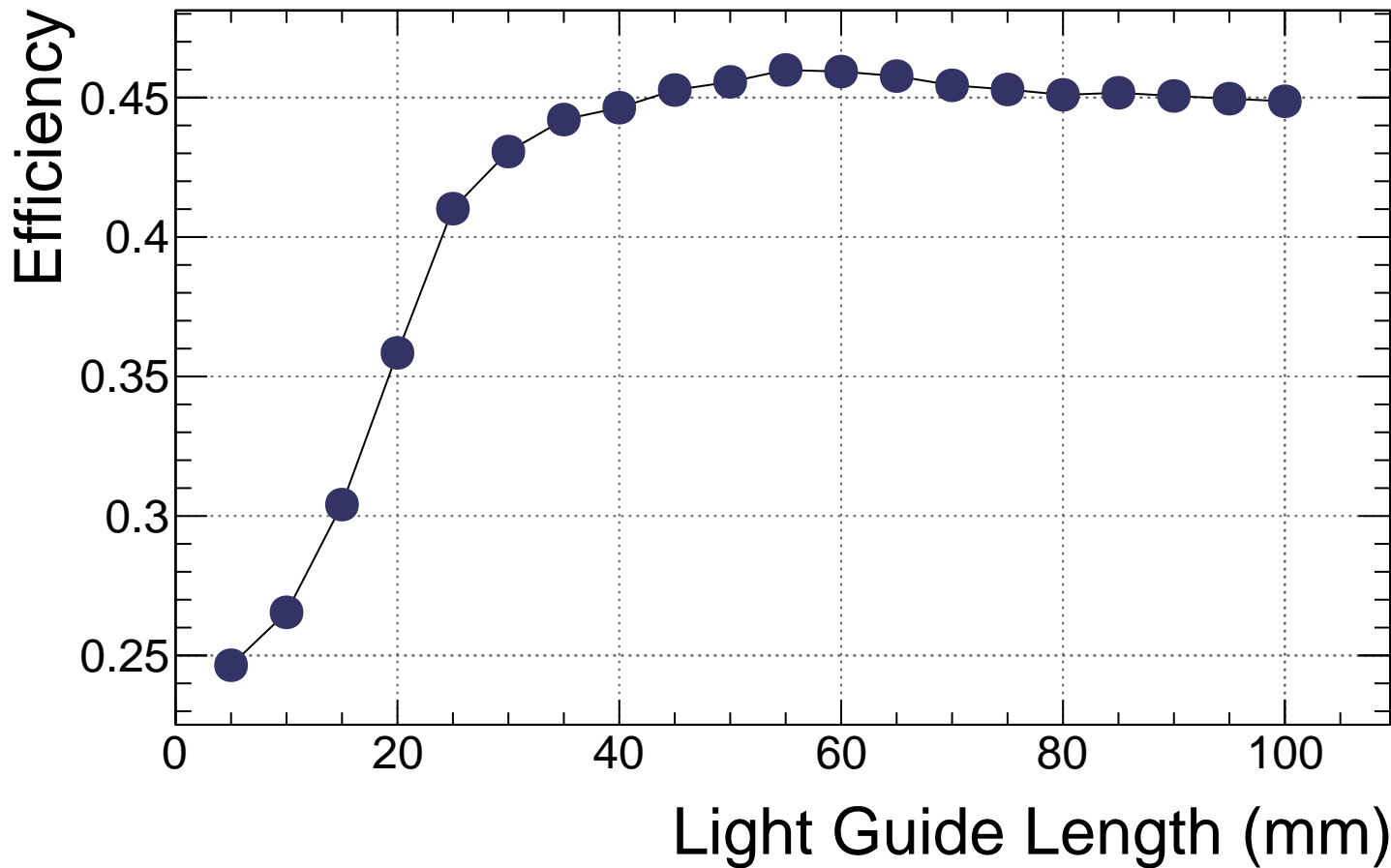
b11 air S13-BIC Efficiency vs. Length
