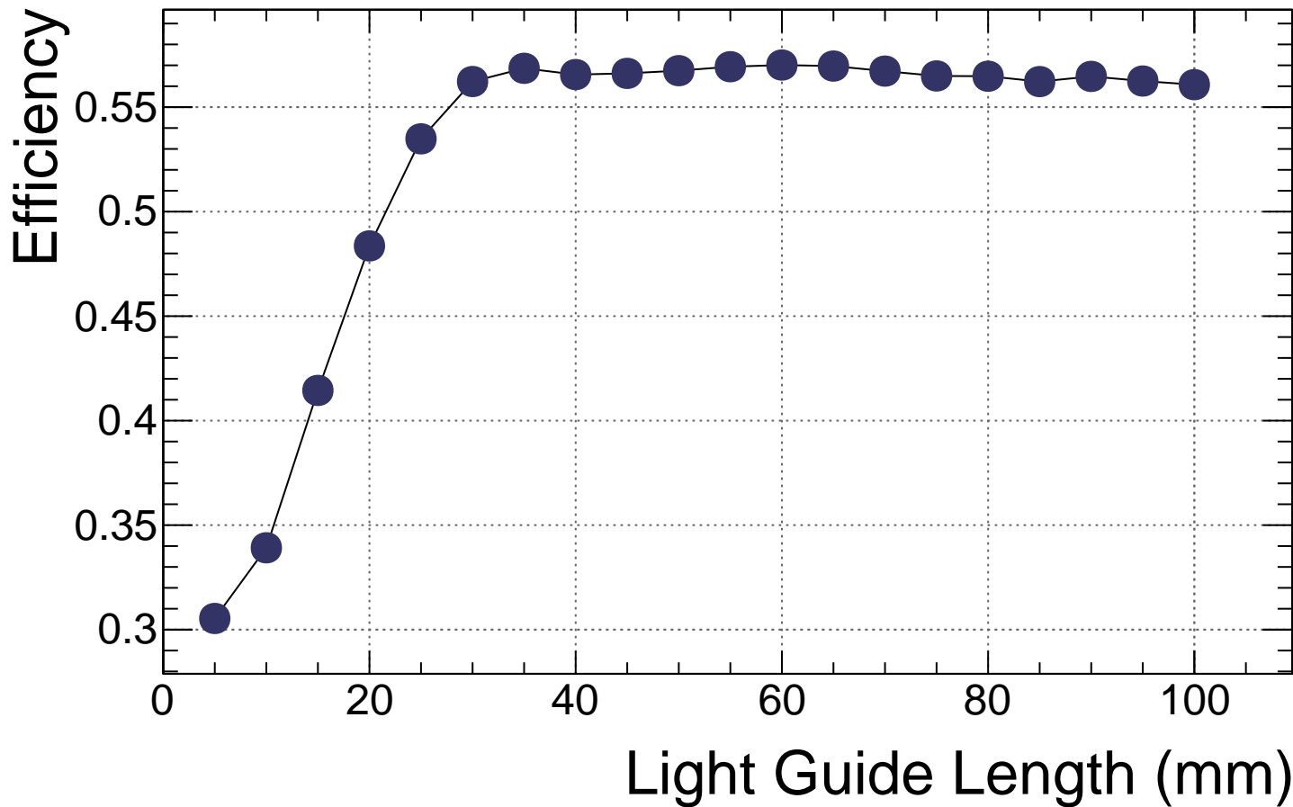
b2 air S13-BIC Efficiency vs. Length
