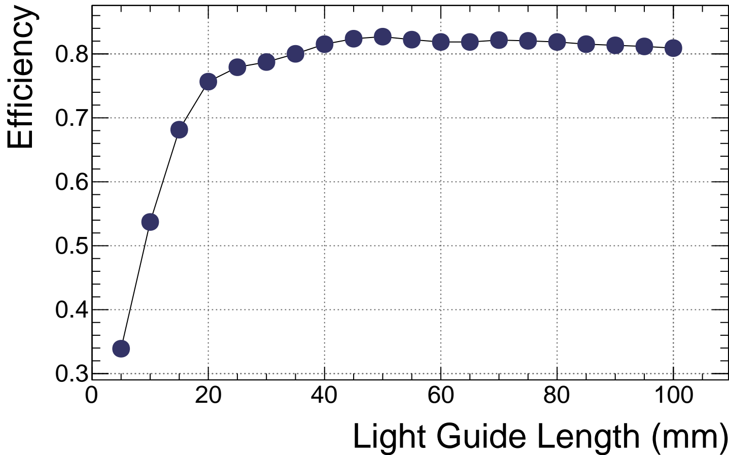
b6 cookie S13-BIC Efficiency vs. Length
