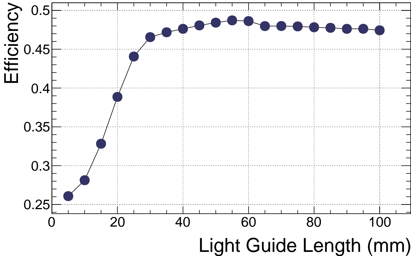
b8 air S13-BIC Efficiency vs. Length
