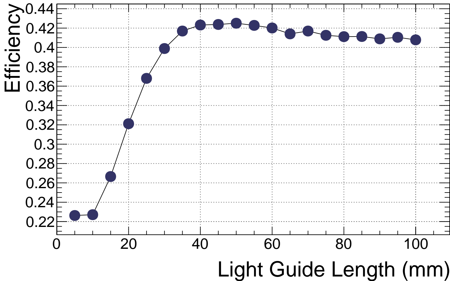
g10 air S12-GlueX Efficiency vs. Length
