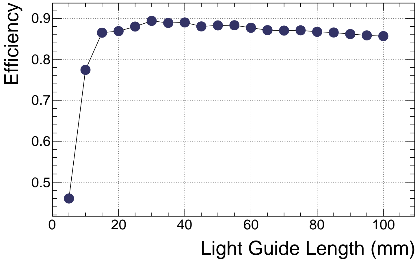
g1 cookie S12-GlueX Efficiency vs. Length
