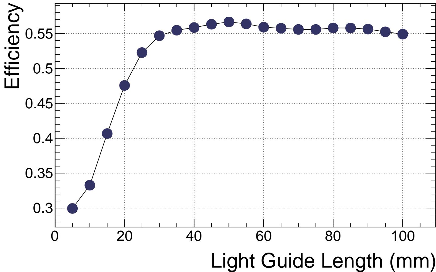
g6 air S12-GlueX Efficiency vs. Length
