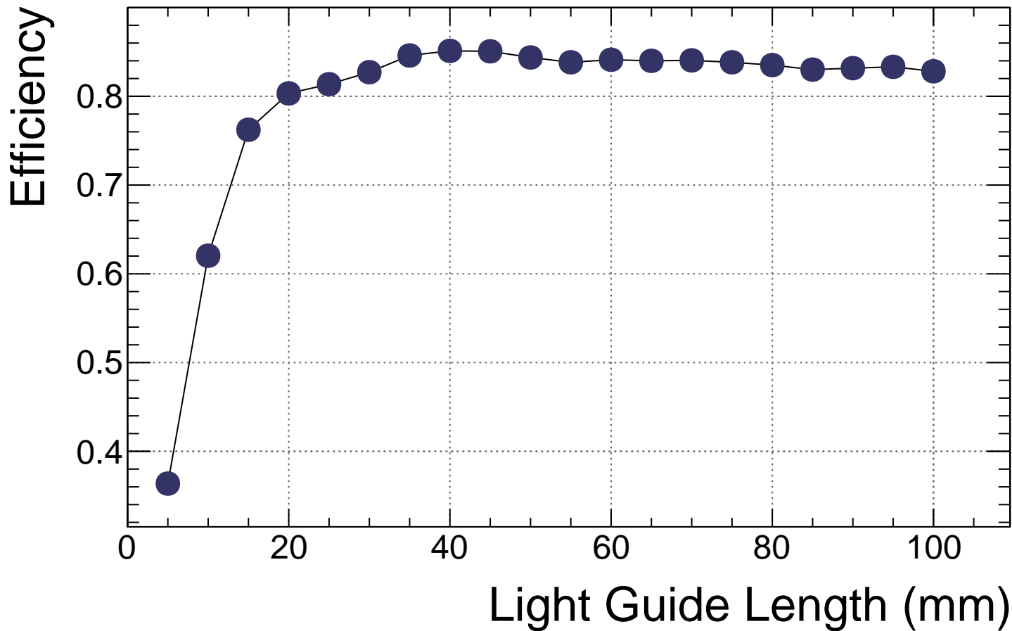
g6 cookie S12-GlueX Efficiency vs. Length
