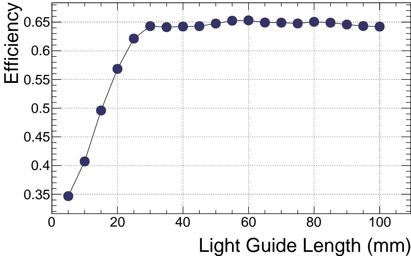
g1 air S12-GlueX Efficiency vs. Length
