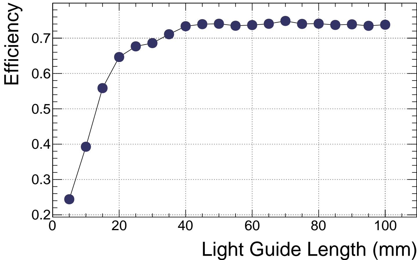
g10 cookie S12-GlueX Efficiency vs. Length
