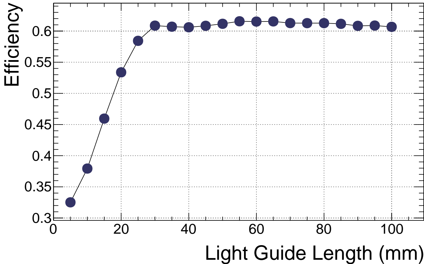
g3 air S12-GlueX Efficiency vs. Length
