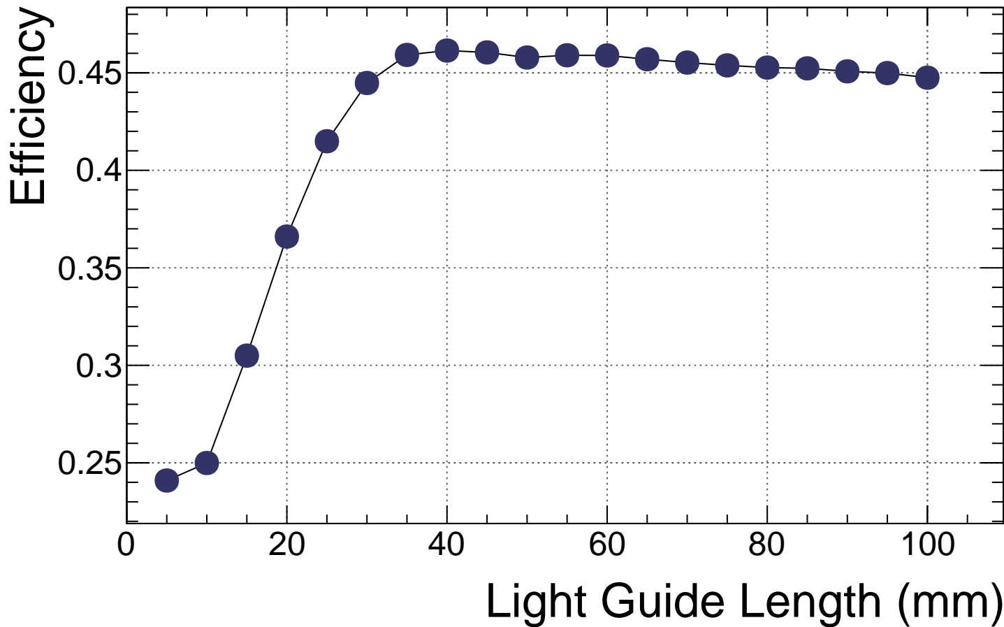
g7 air S12-GlueX Efficiency vs. Length
