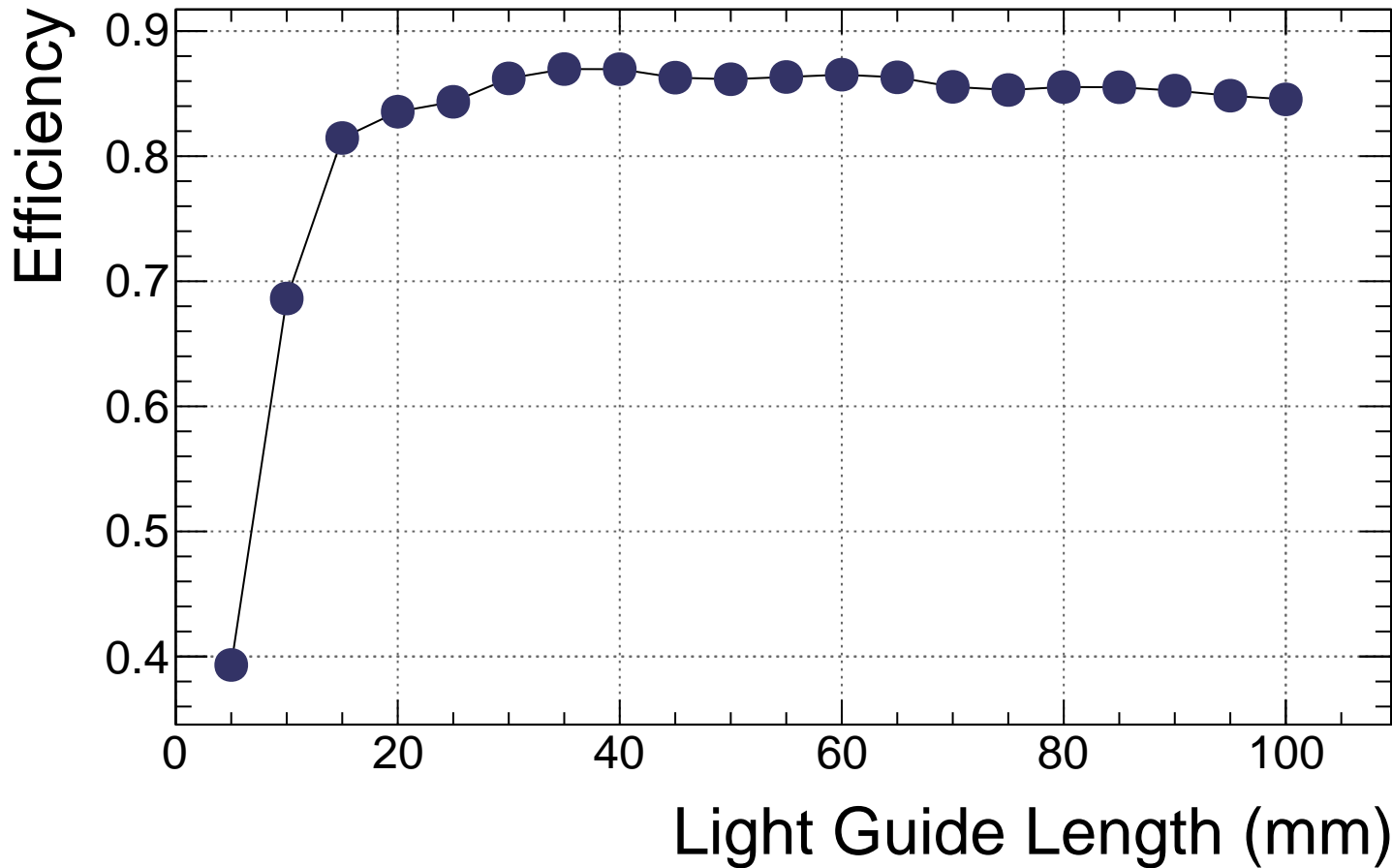
g4 cookie S12-GlueX Efficiency vs. Length
