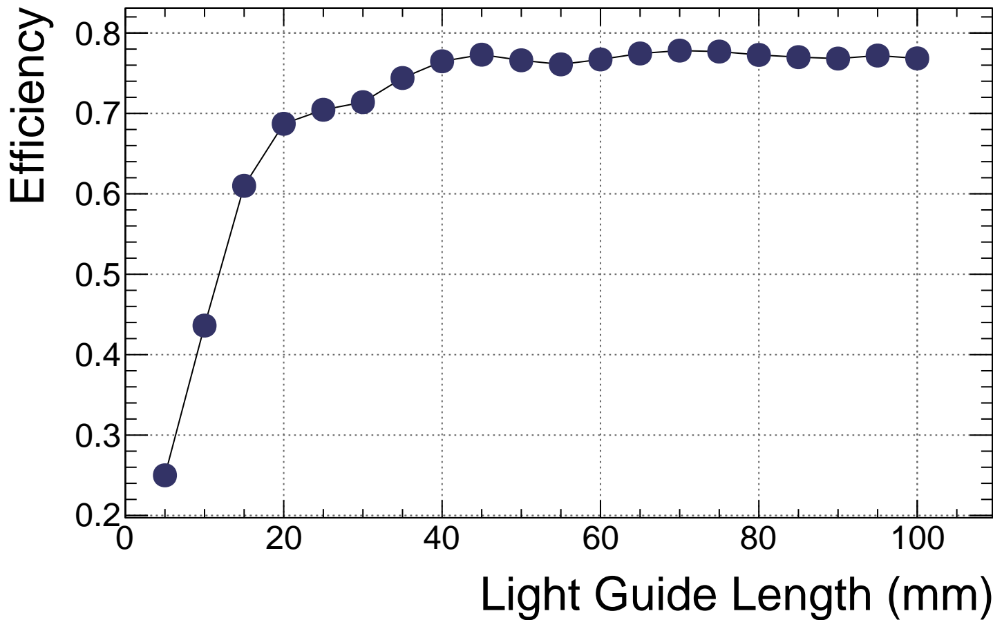
g8 cookie S12-GlueX Efficiency vs. Length
