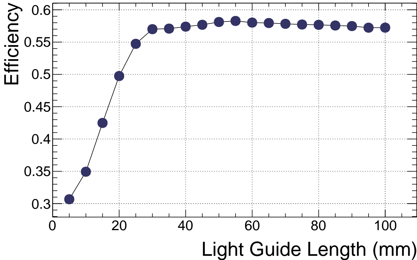
g5 air S12-GlueX Efficiency vs. Length
