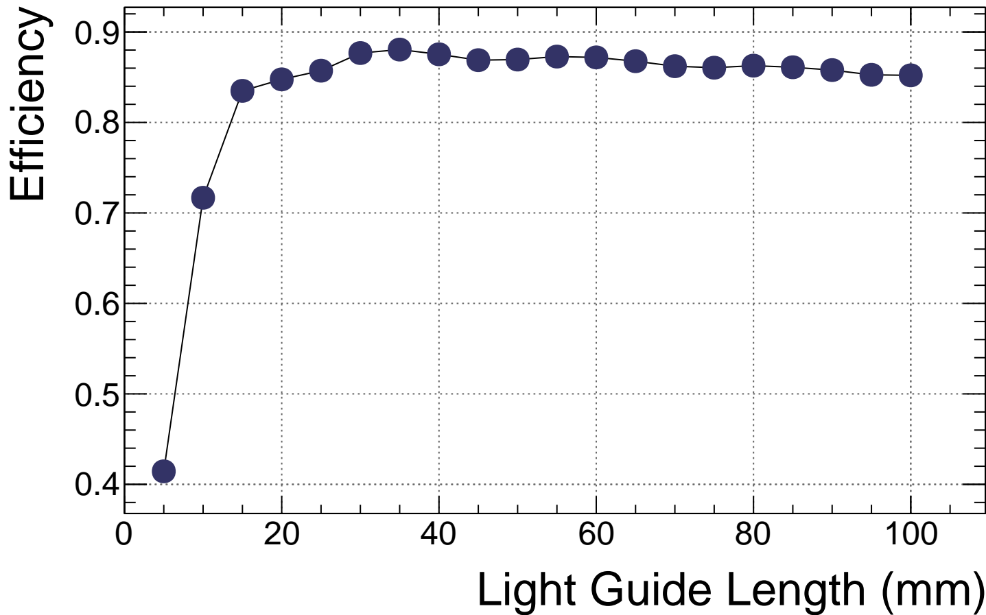
g3 cookie S12-GlueX Efficiency vs. Length
