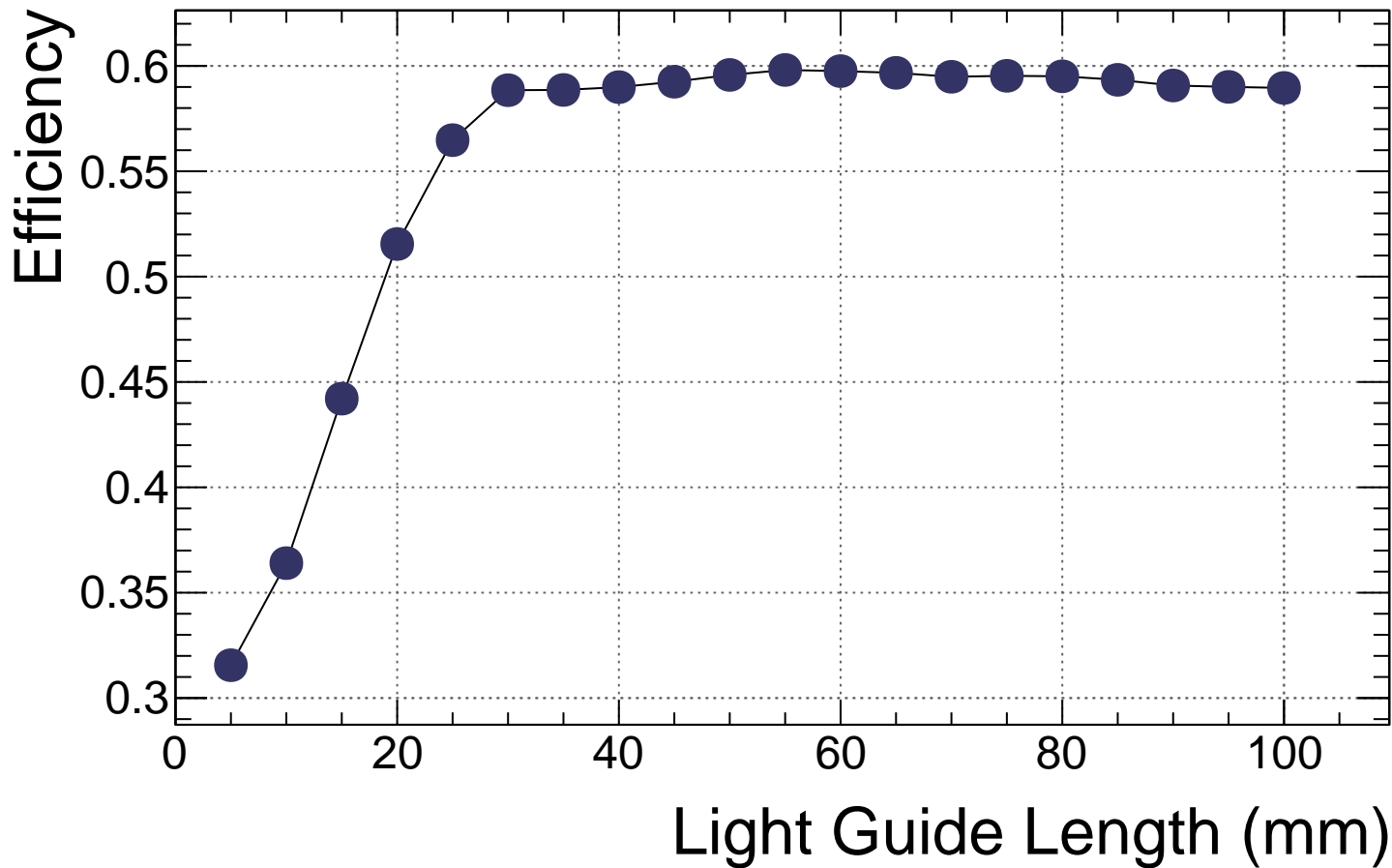
g4 air S12-GlueX Efficiency vs. Length
