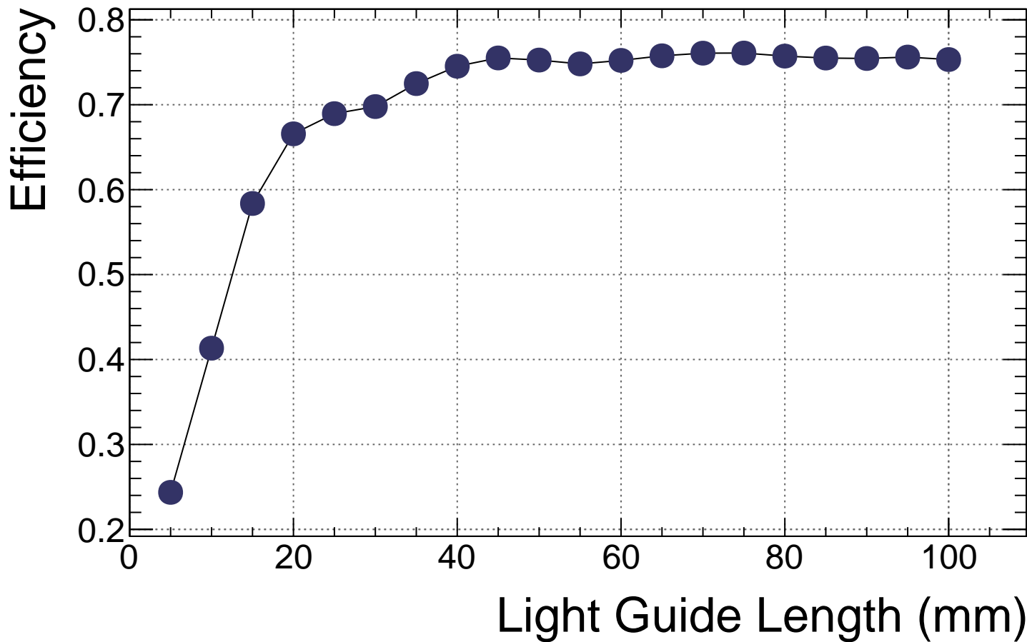
g9 cookie S12-GlueX Efficiency vs. Length
