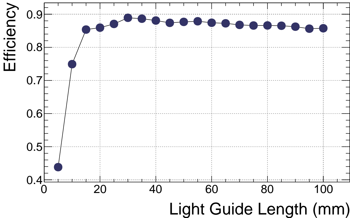
g2 cookie S12-GlueX Efficiency vs. Length
