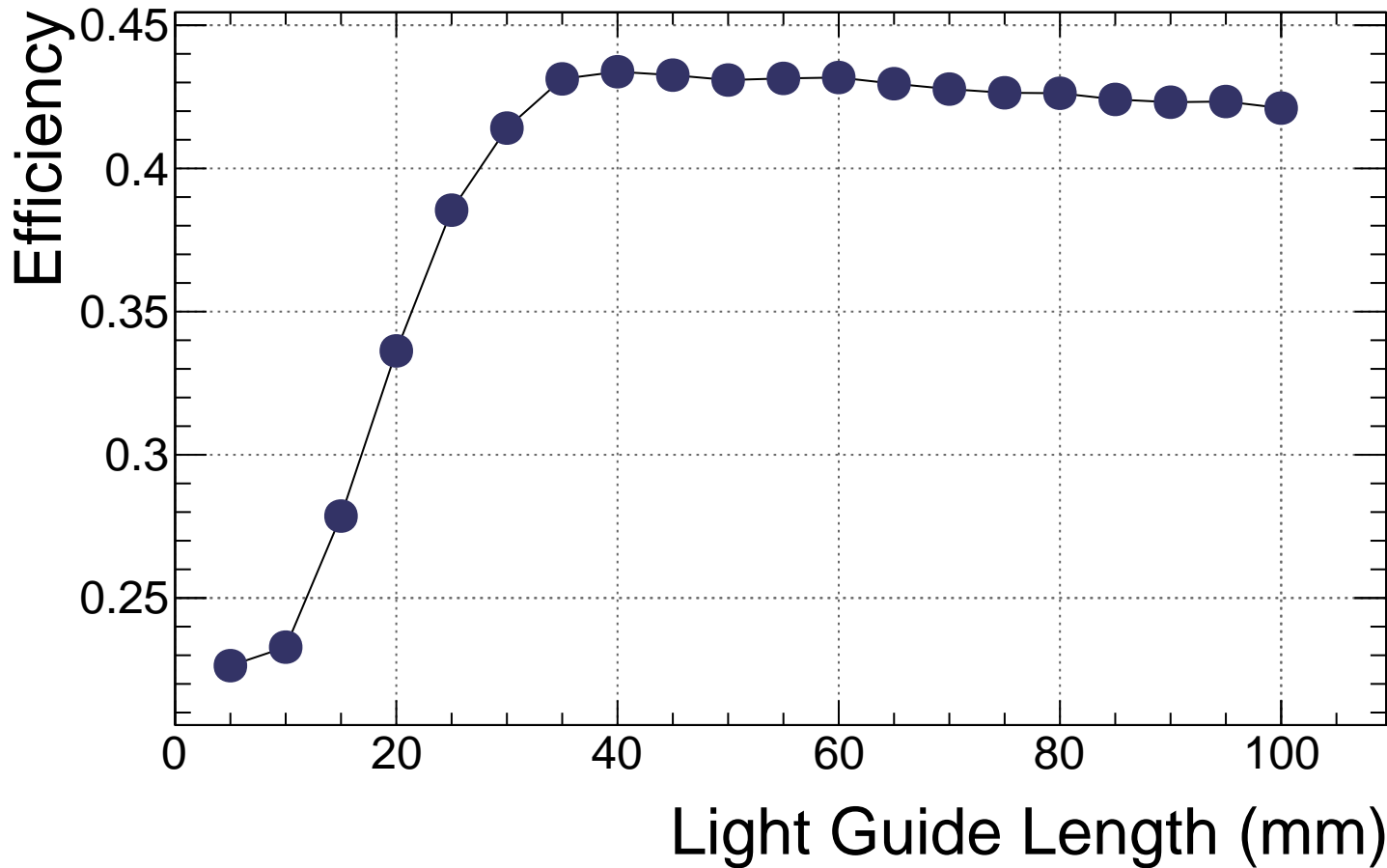
g9 air S12-GlueX Efficiency vs. Length
