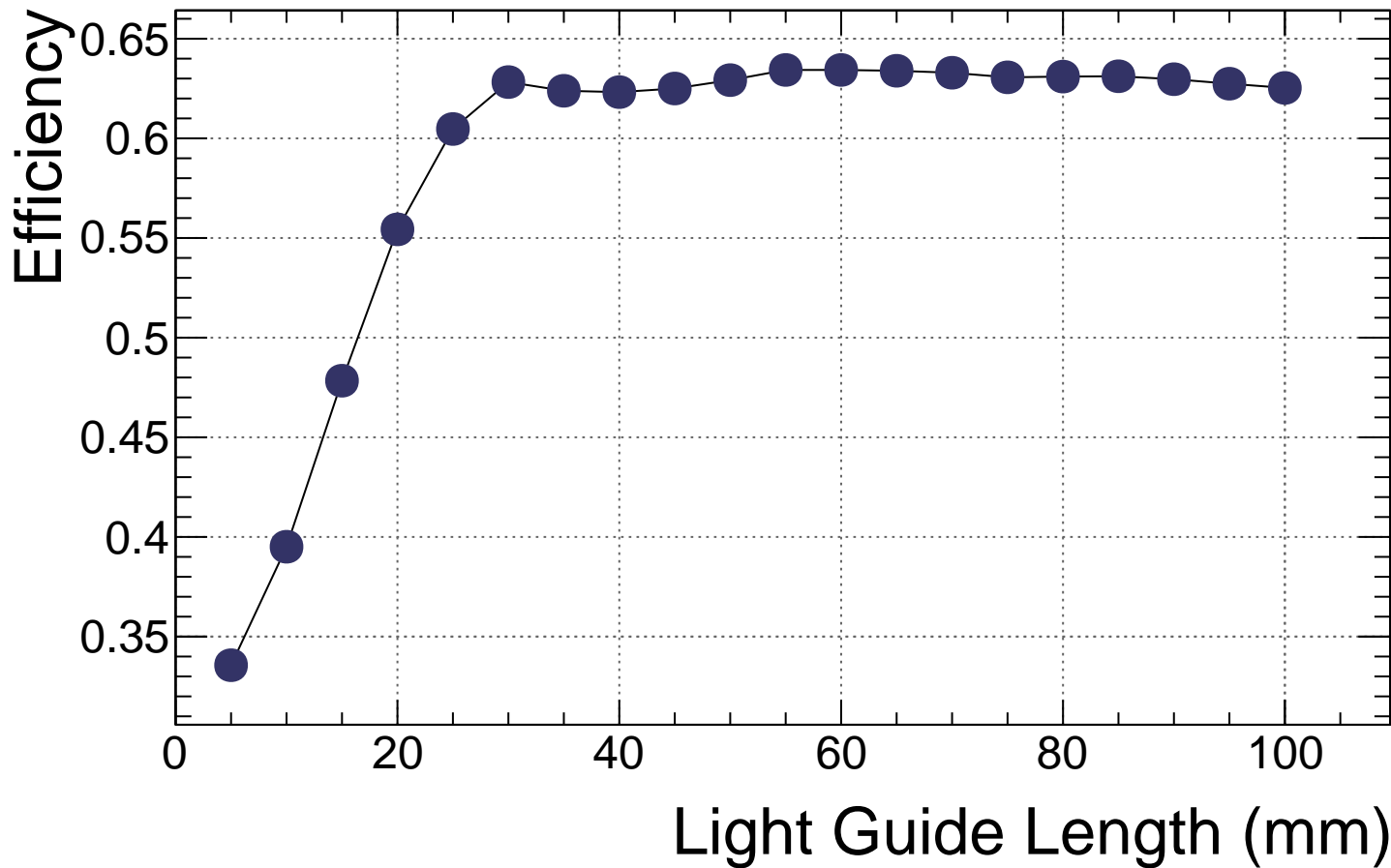
g2 air S12-GlueX Efficiency vs. Length
