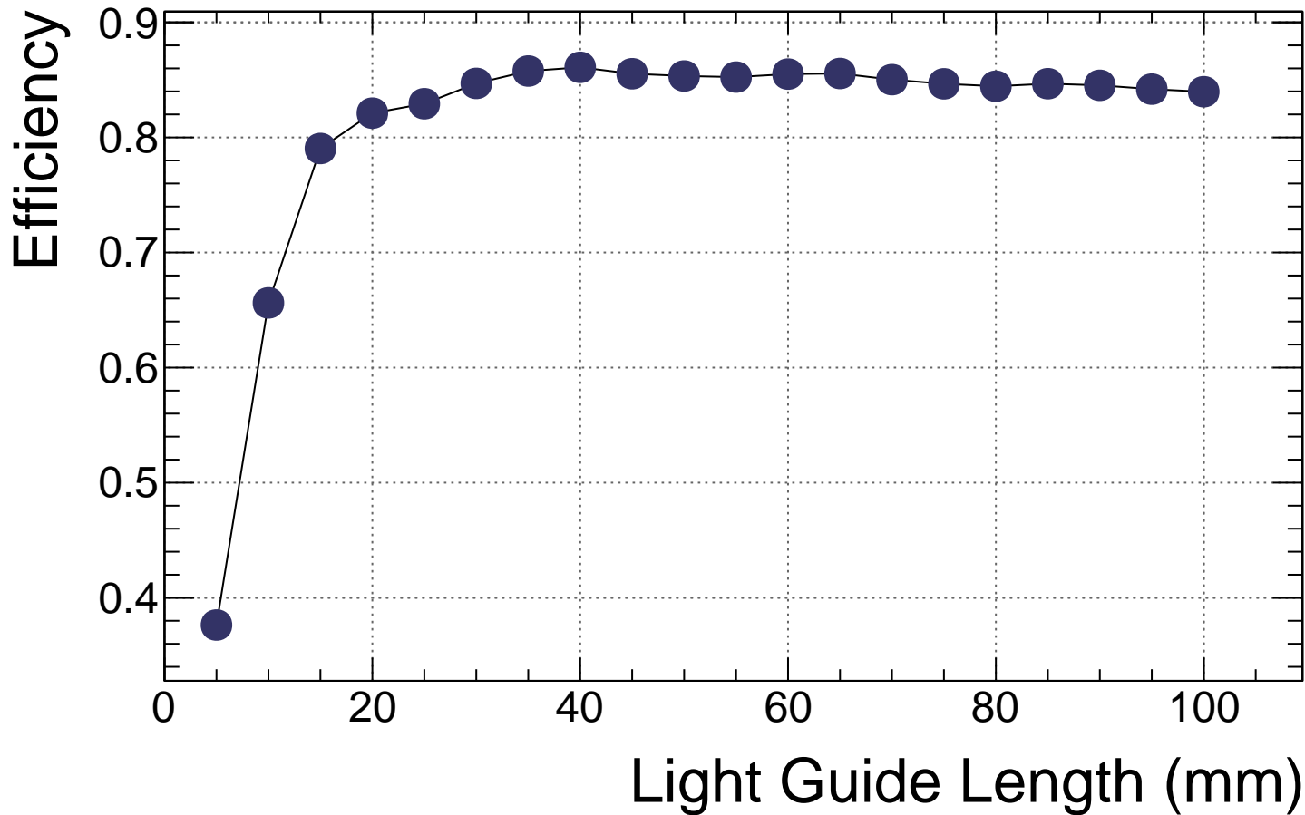
g5 cookie S12-GlueX Efficiency vs. Length
