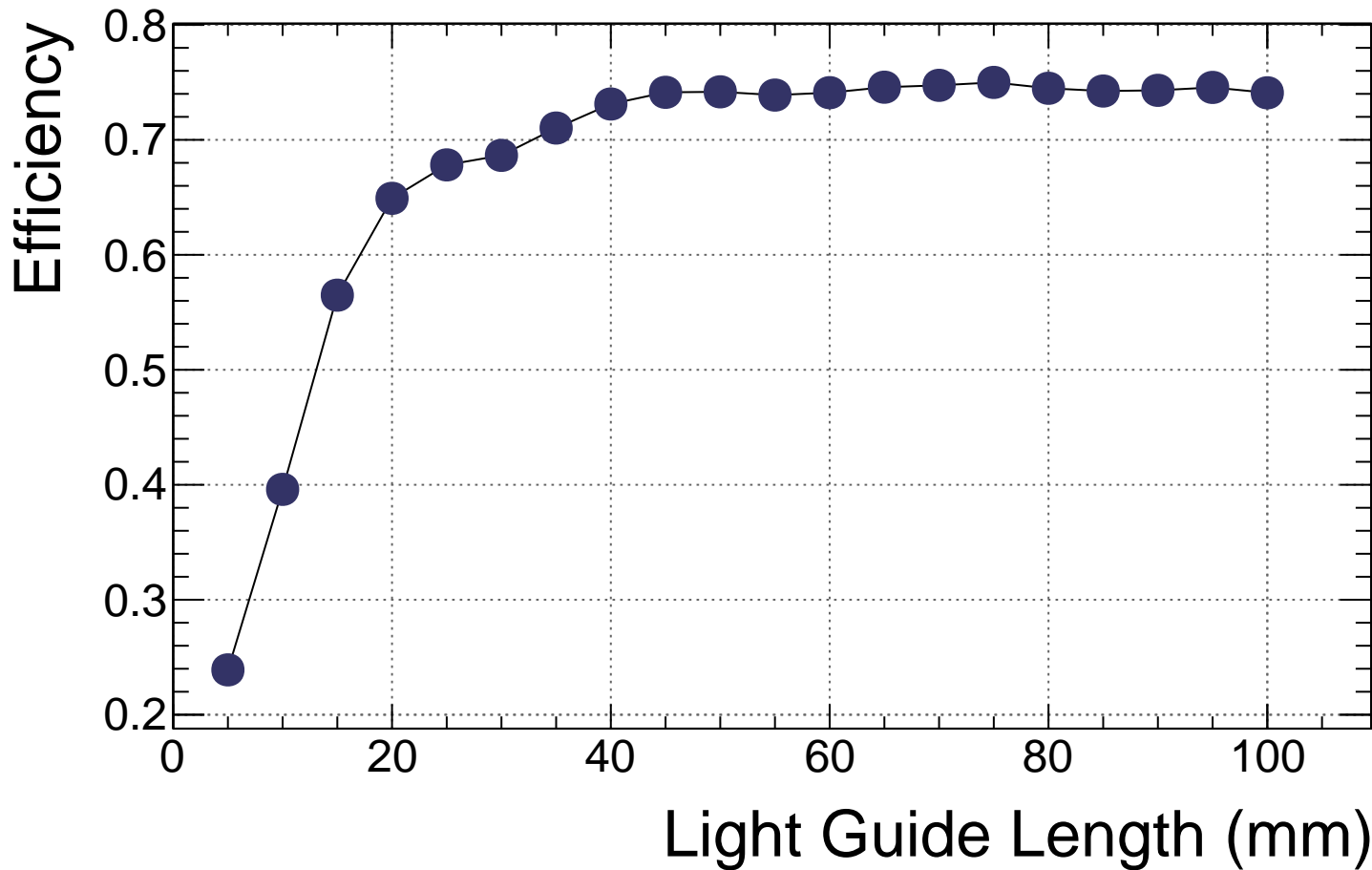
g10 cookie S12-GlueX Efficiency vs. Length
