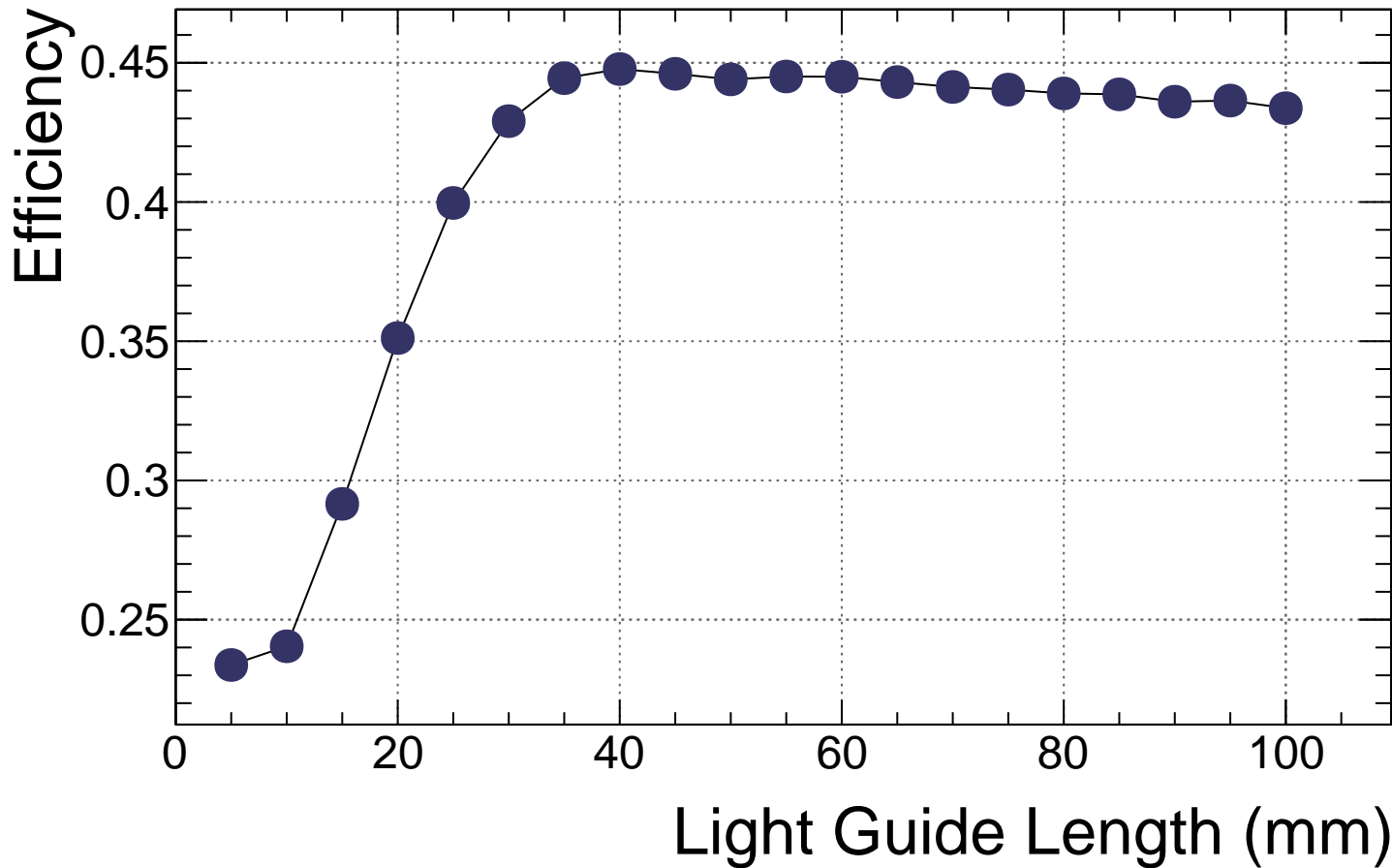
g8 air S12-GlueX Efficiency vs. Length
