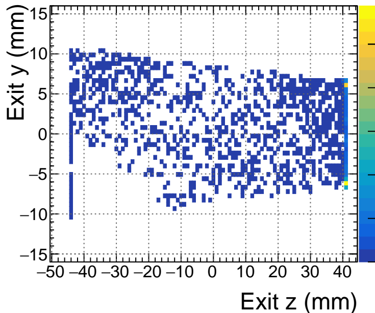
85 mm Exit y vs. z (Failure)
