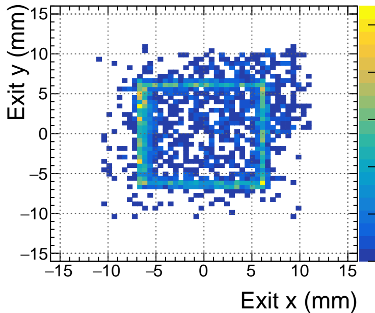
70 mm Exit y vs. x (Failure)
