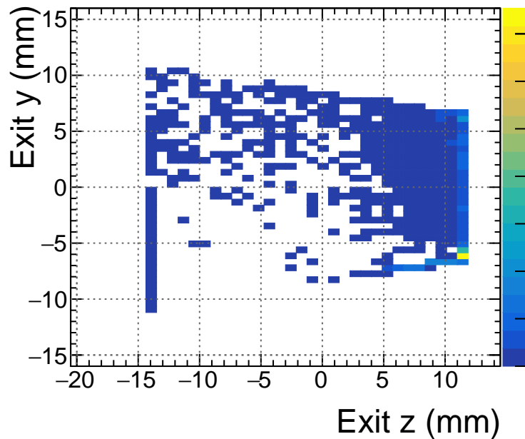
25 mm Exit y vs. z (Failure)
