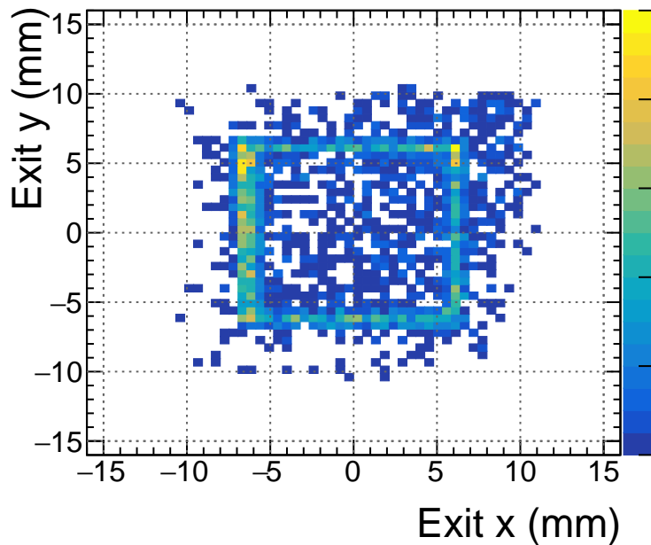
75 mm Exit y vs. x (Failure)
