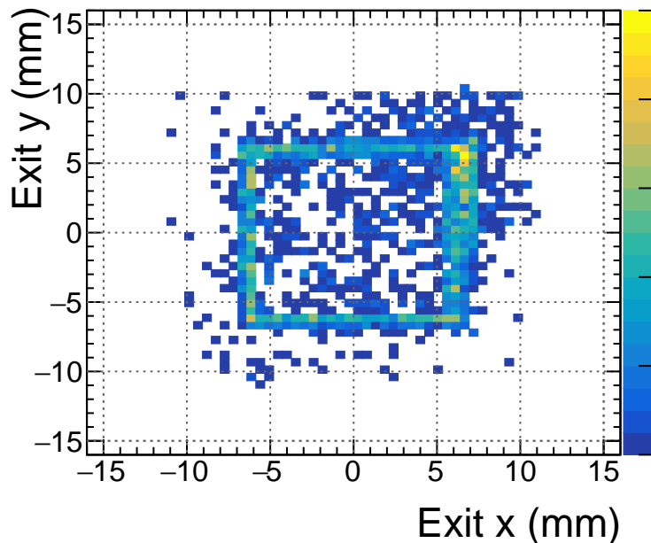
55 mm Exit y vs. x (Failure)
