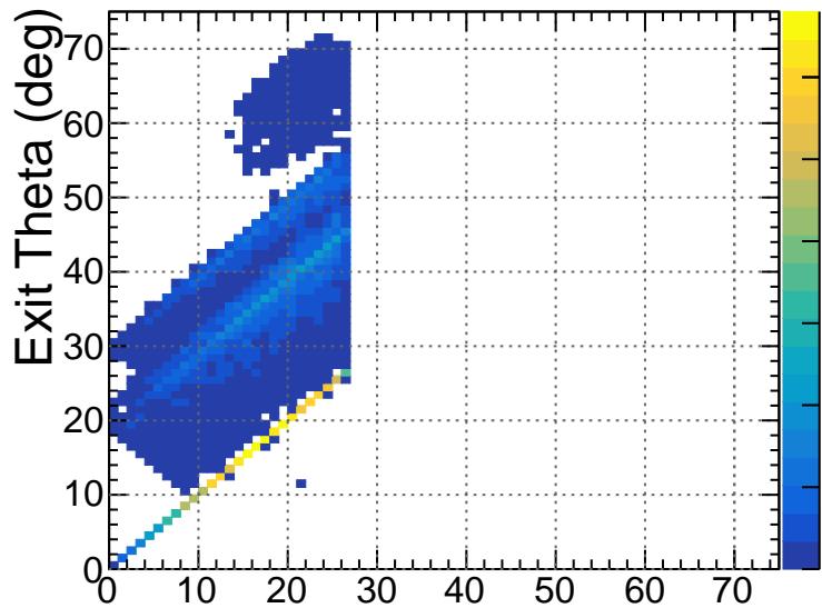
25 mm Exit Theta vs. Entrance Theta (Success)
