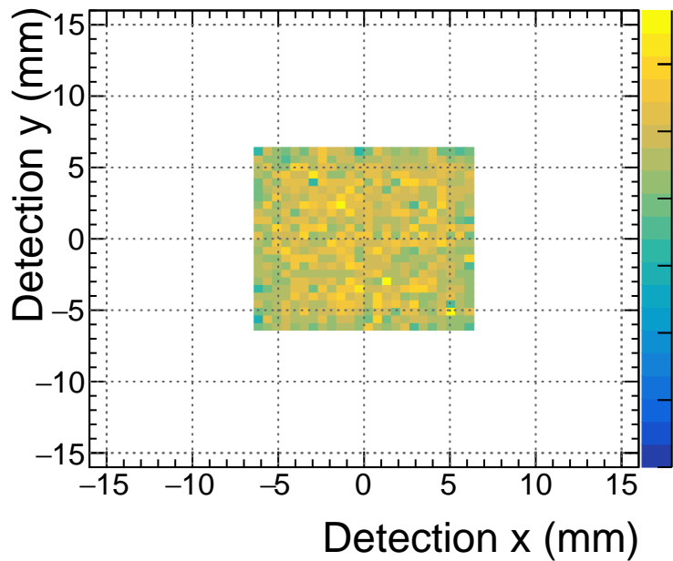
80 mm Detection y vs. x (Success)
