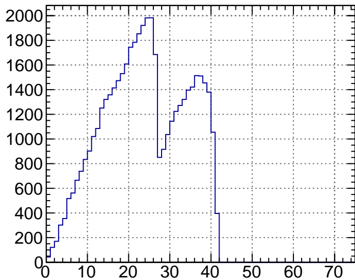
20 mm Exit Theta (Success)
