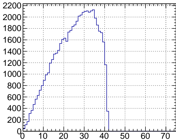
45 mm Exit Theta (Success)
