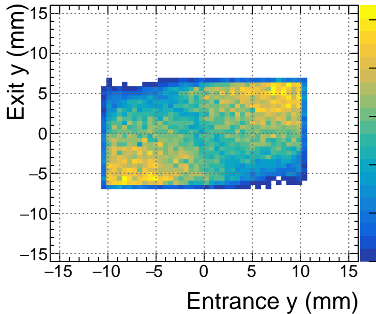
25 mm Exit y vs. Entrance y (Success)
