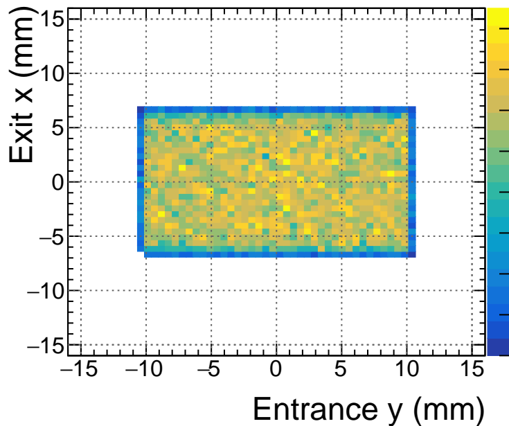
40 mm Exit x vs. Entrance y (Success)
