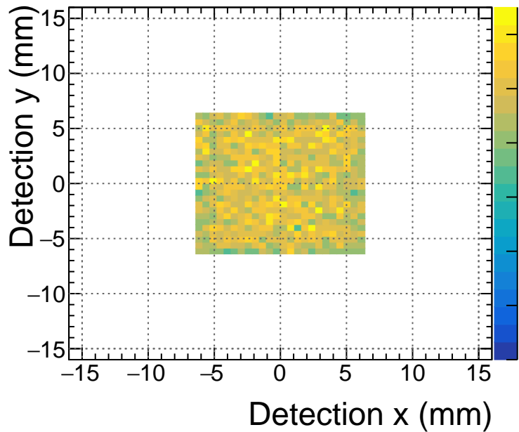
85 mm Detection y vs. x (Success)
