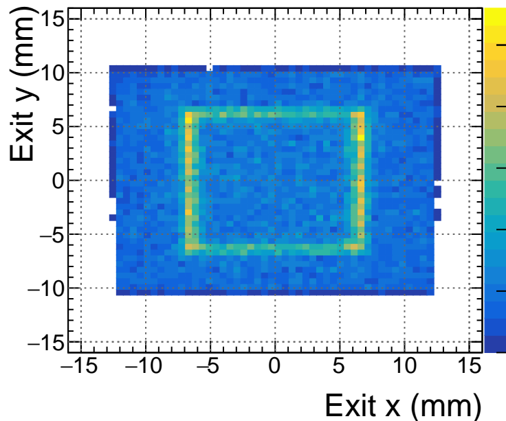
70 mm Exit y vs. x (Failure)
