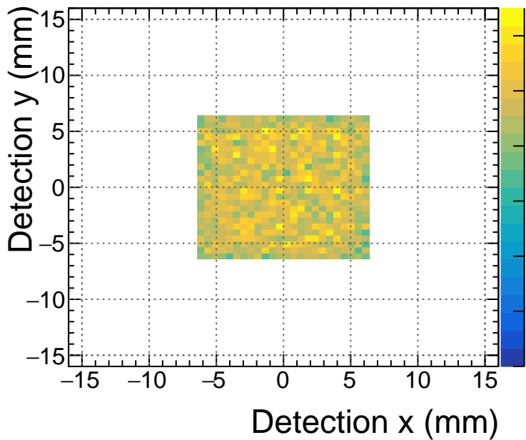
35 mm Detection y vs. x (Success)
