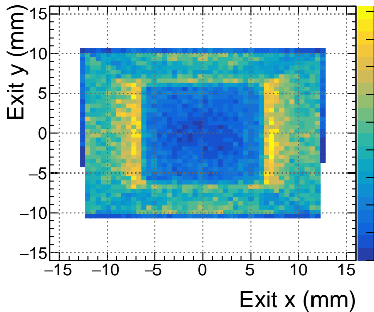
10 mm Exit y vs. x (Failure)
