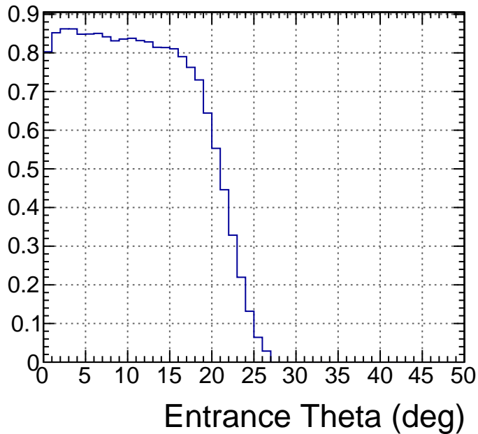
95 mm Entrance Theta Efficiency
