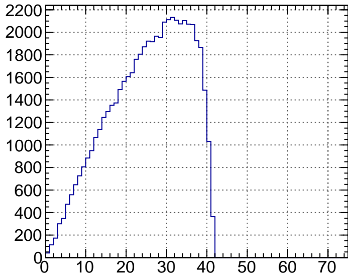
60 mm Exit Theta (Success)
