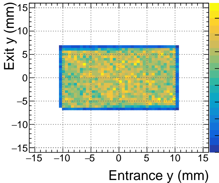
40 mm Exit y vs. Entrance y (Success)
