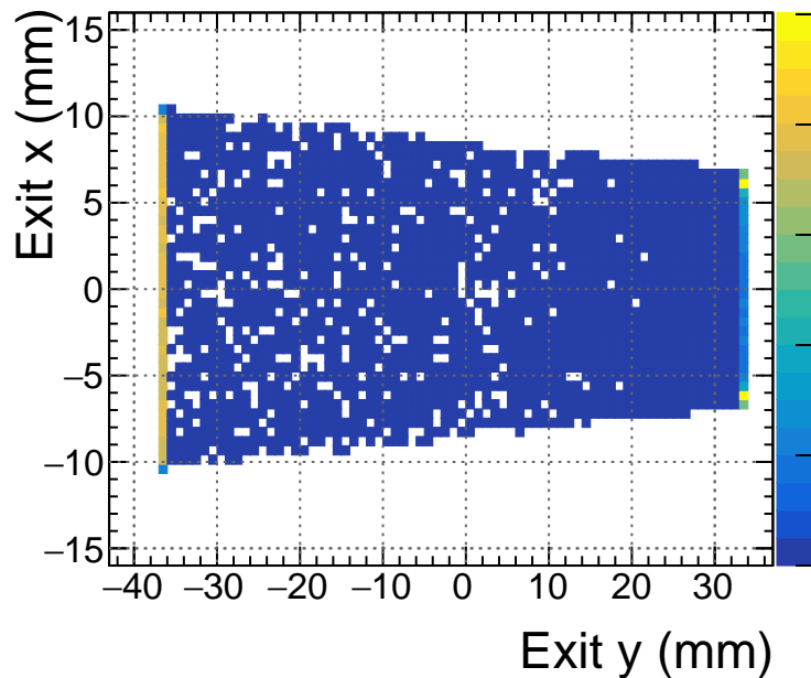
70 mm Exit y vs. z (Failure)
