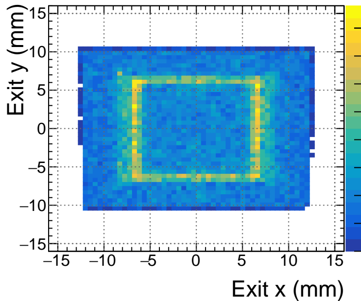
35 mm Exit y vs. x (Failure)
