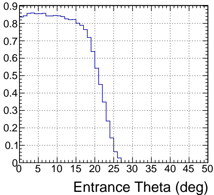
90 mm Entrance Theta Efficiency
