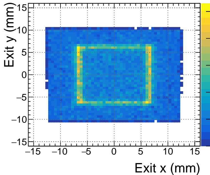
95 mm Exit y vs. x (Failure)
