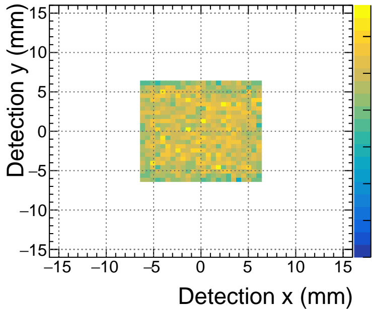
50 mm Detection y vs. x (Success)
