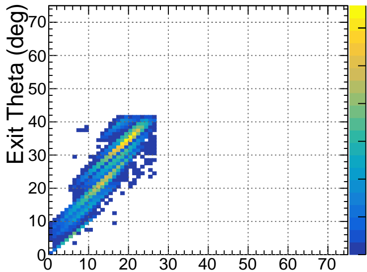
Entrance Theta (deg)
