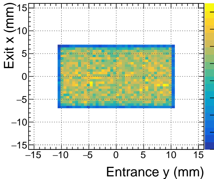
25 mm Exit x vs. Entrance y (Success)
