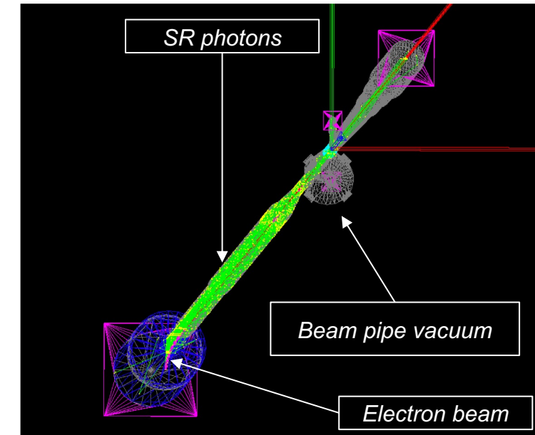
Geant4 geometry
