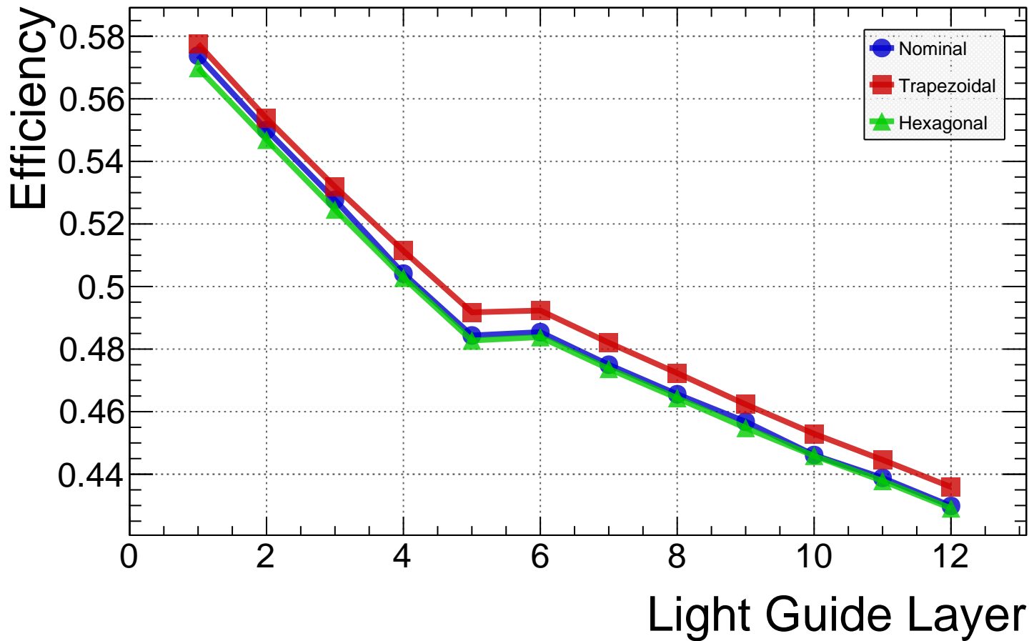
45 mm air S13-BIC Efficiency vs. Layer
