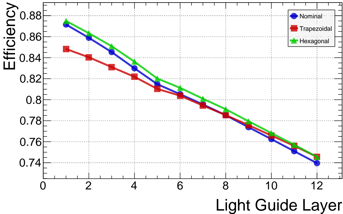
50 mm cookie S13-BIC Efficiency vs. Layer
