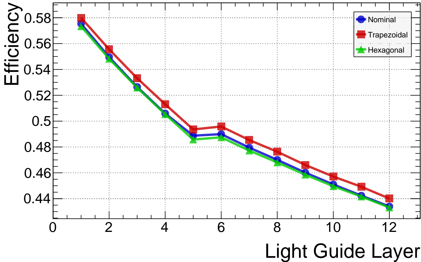
50 mm air S13-BIC Efficiency vs. Layer
