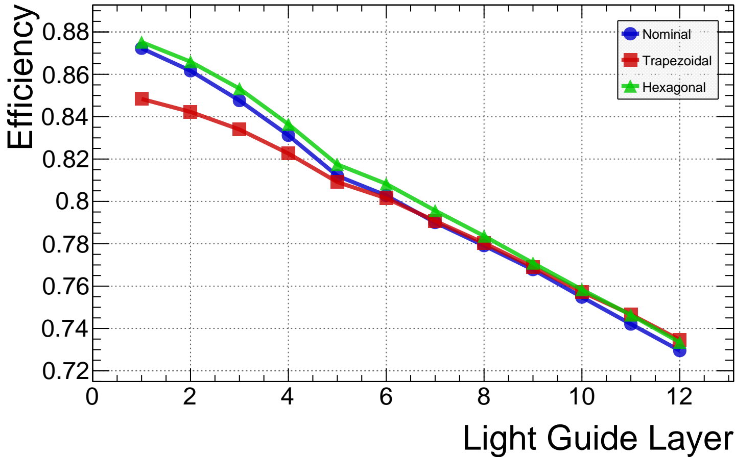
45 mm cookie S13-BIC Efficiency vs. Layer
