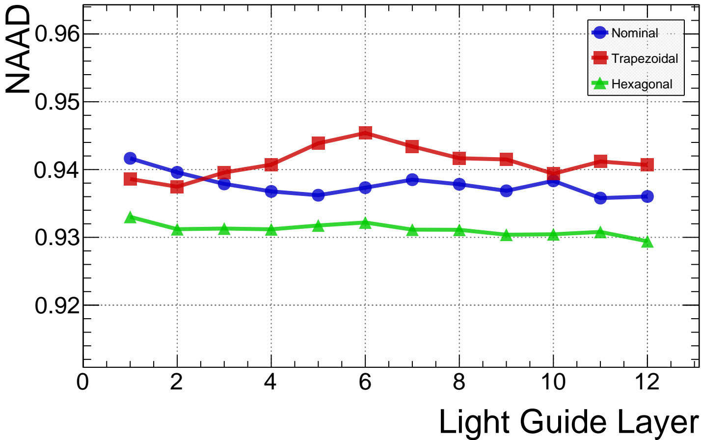
50 mm cookie S13-BIC NAAD vs. Layer
