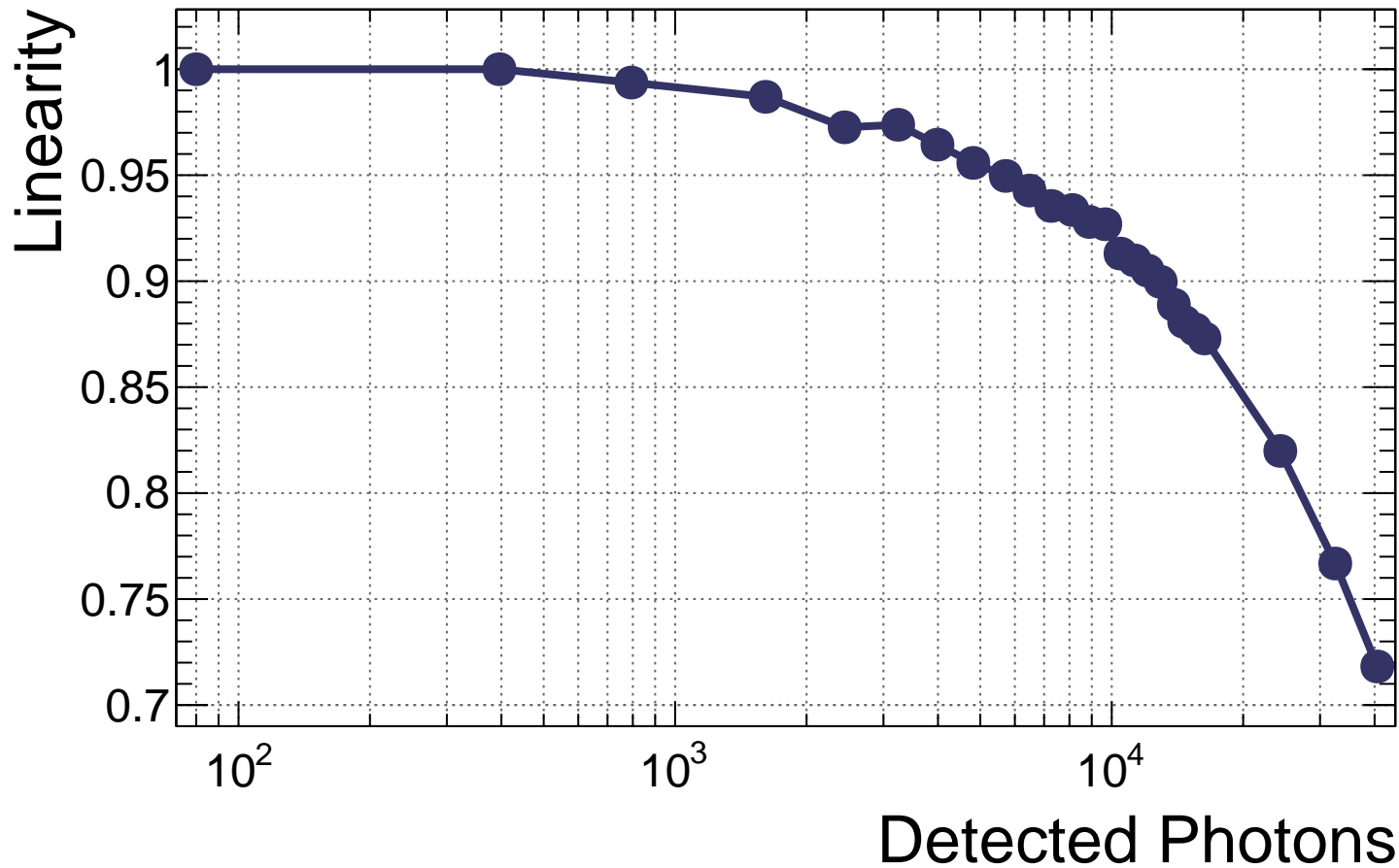
BIC Layer 5 50 mm cookie S13-BIC Linearity vs. Npe
