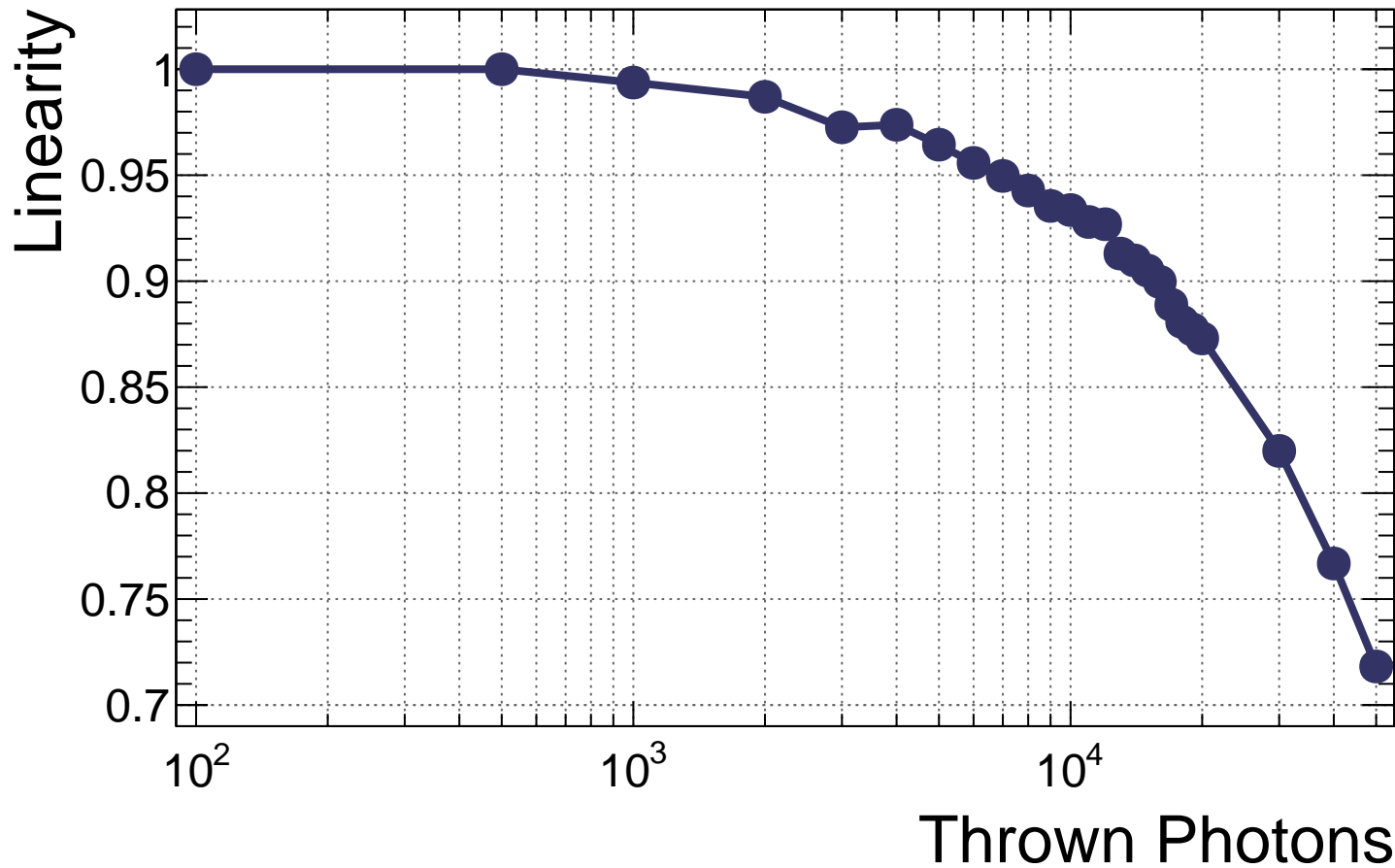
BIC Layer 5 50 mm cookie S13-BIC Linearity vs. Thrown Photons
