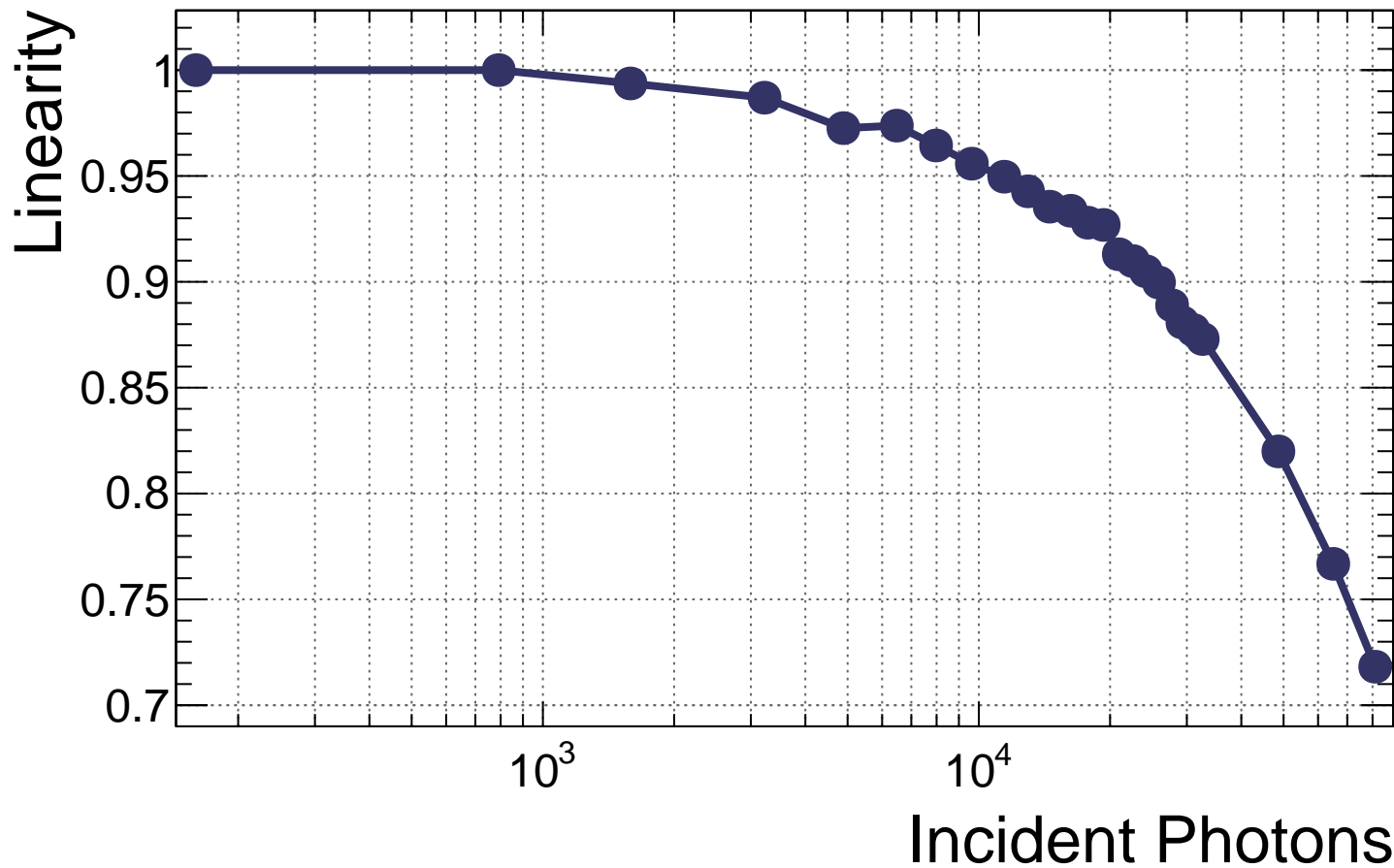
BIC Layer 5 50 mm cookie S13-BIC Linearity vs. Incident Photons (50% PDE)
