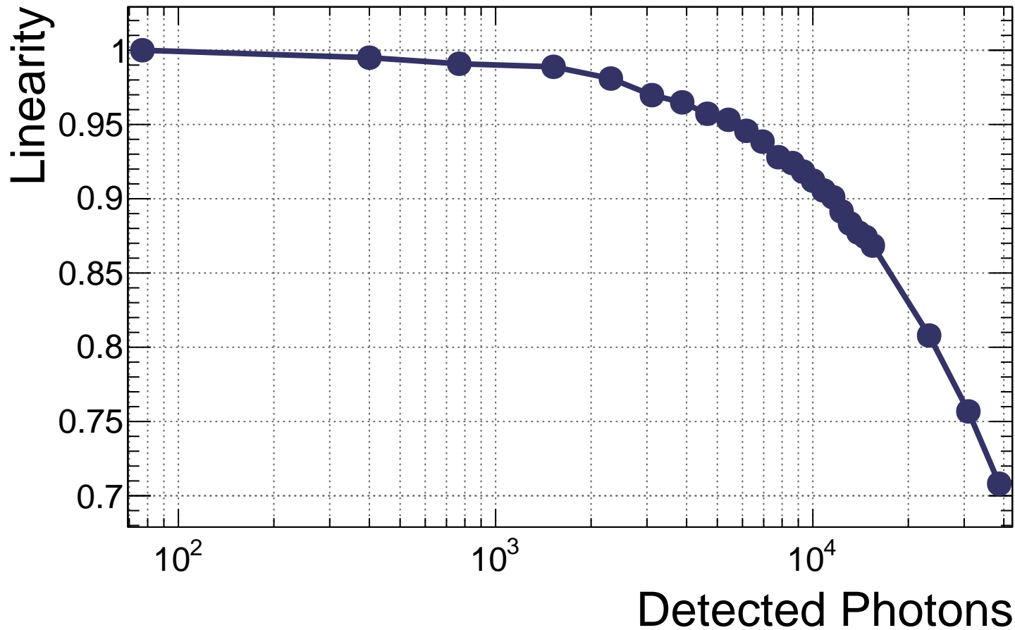
Quadrant Source BIC Layer 5 30 mm cookie S13-BIC Linearity vs. Npe
