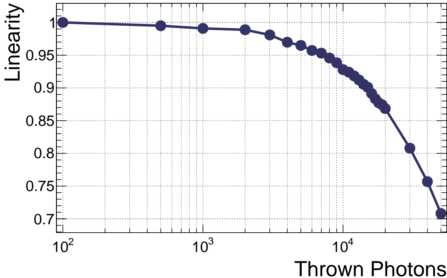
Quadrant Source BIC Layer 5 30 mm cookie S13-BIC Linearity vs. Thrown Photons
