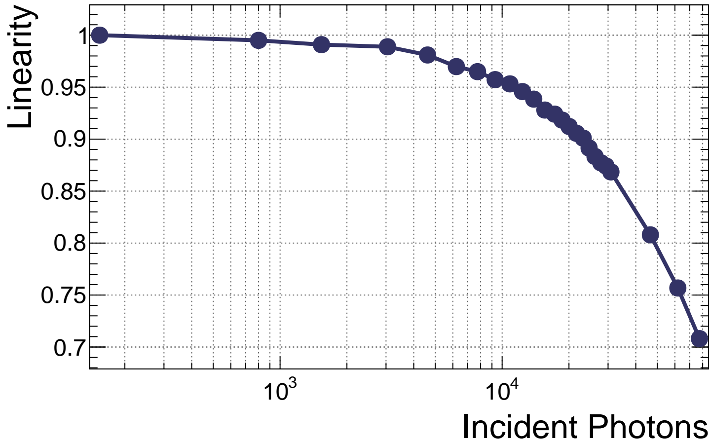
Quadrant Source BIC Layer 5 30 mm cookie S13-BIC Linearity vs. Incident Photons (50% PDE)
