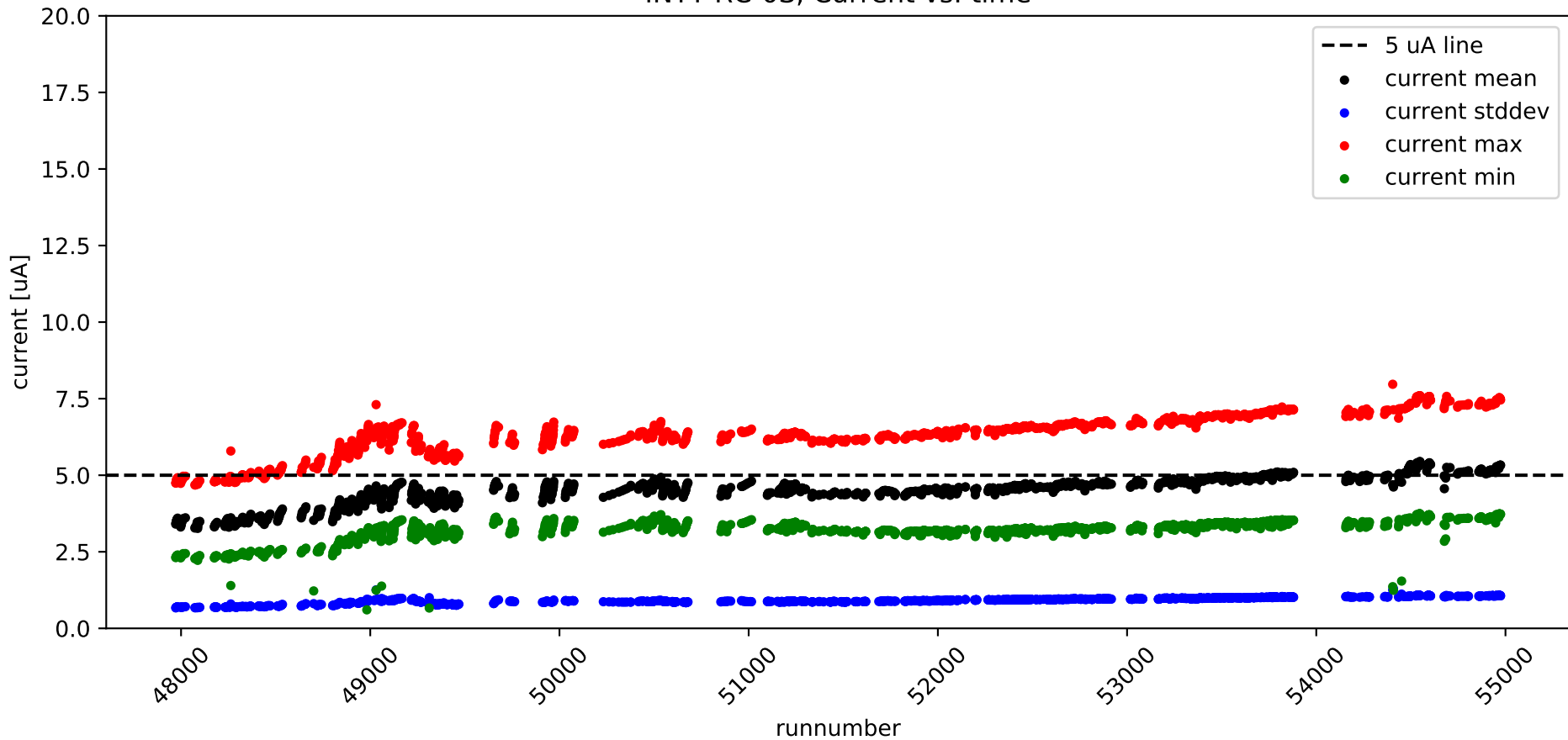
INTT RC-0S, Current vs. time
