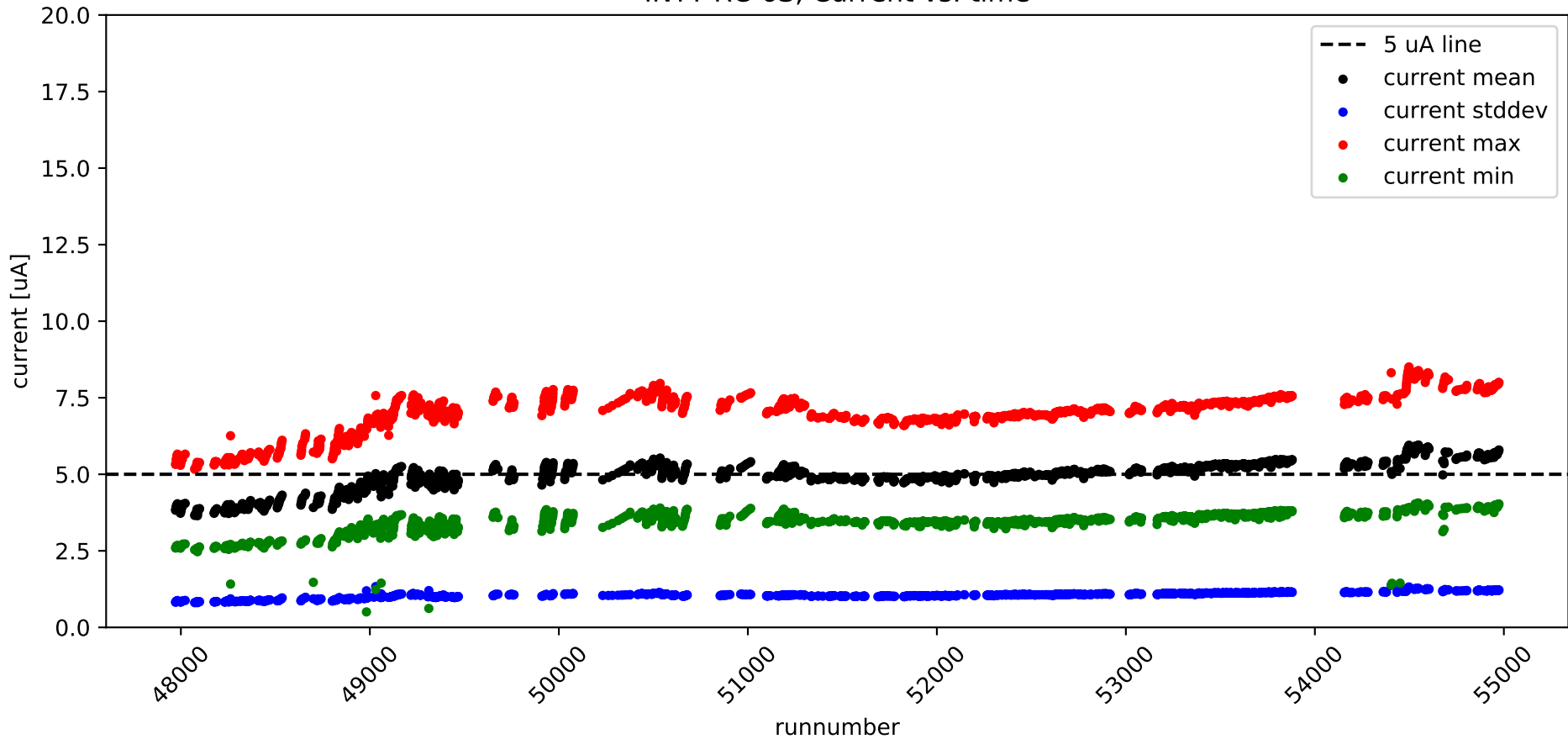
INTT RC-6S, Current vs. time
