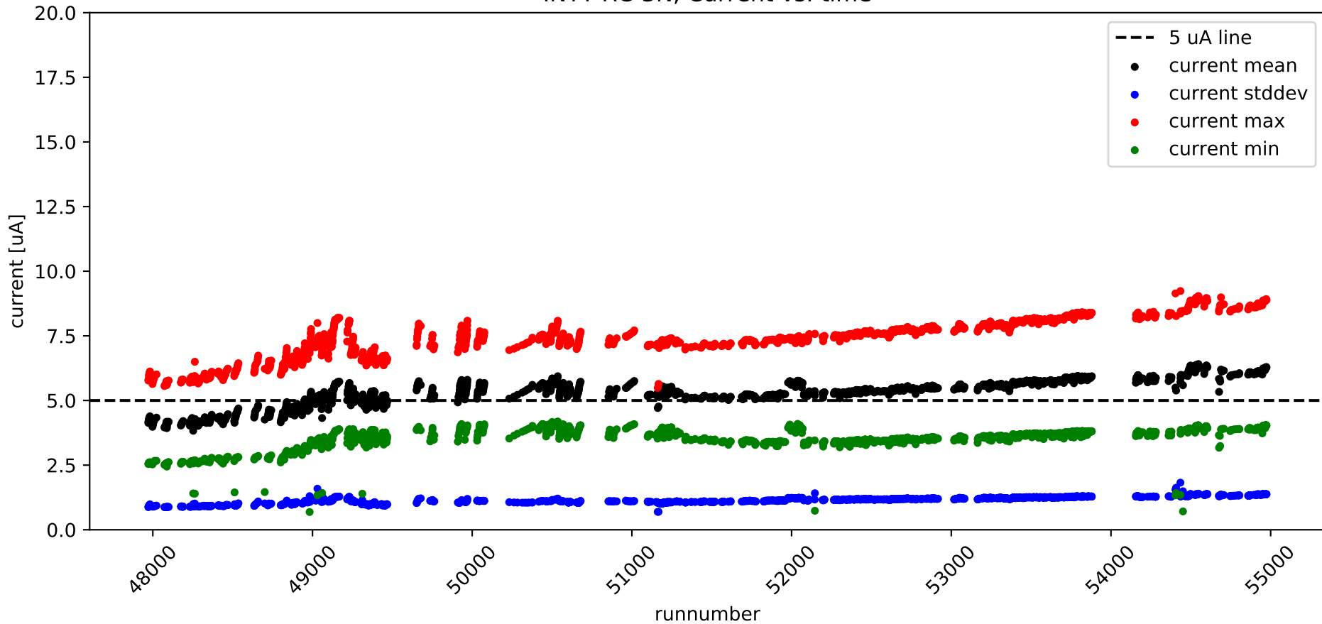
INTT RC-3N, Current vs. time
