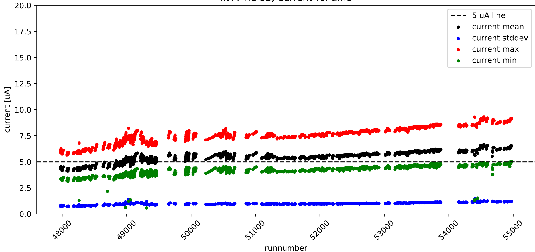
INTT RC-3S, Current vs. time
