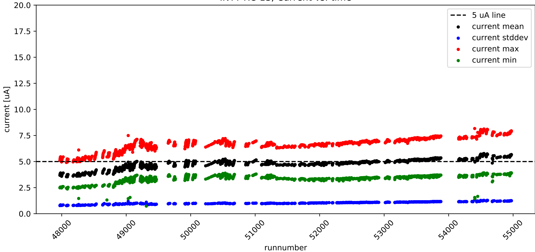
INTT RC-1S, Current vs. time
