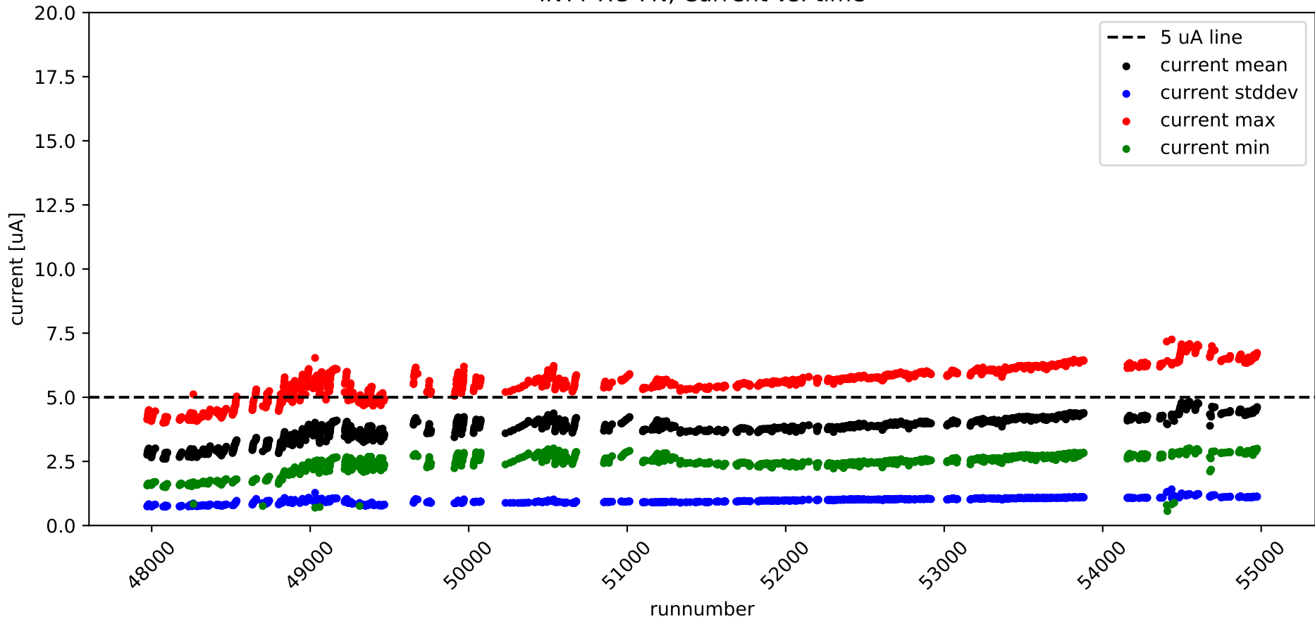
INTT RC-7N, Current vs. time
