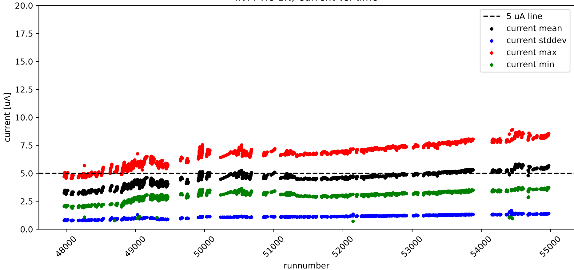
INTT RC-1N, Current vs. time
