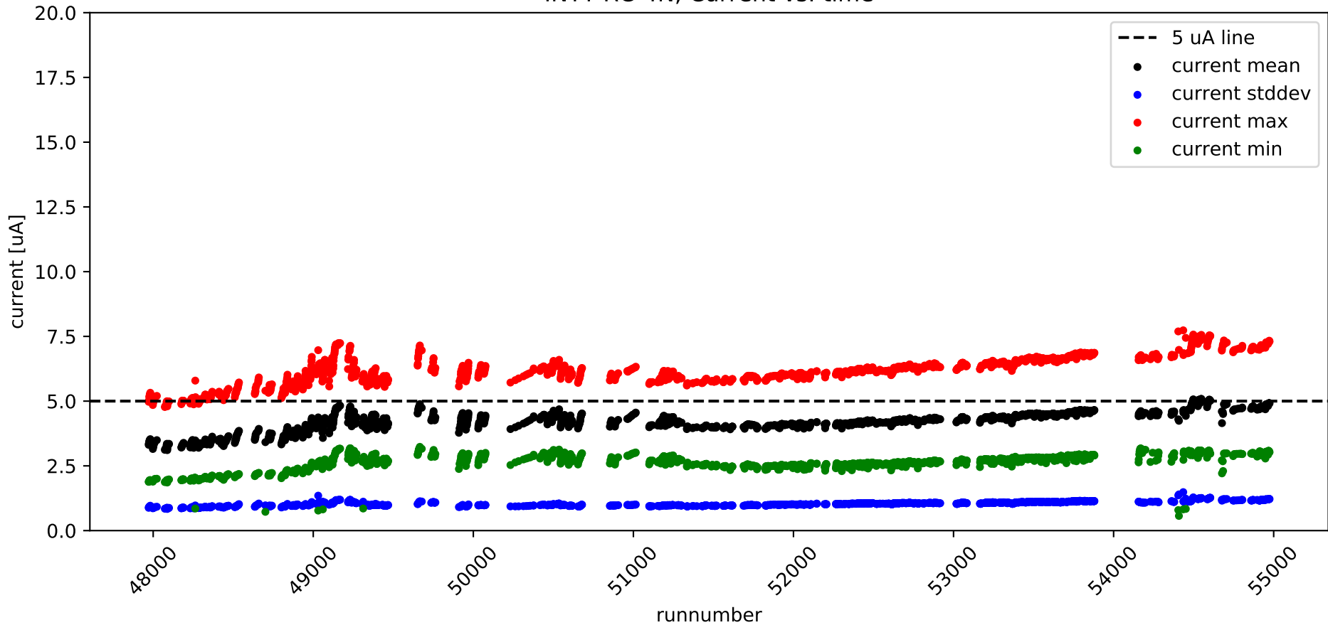
INTT RC-4N, Current vs. time
