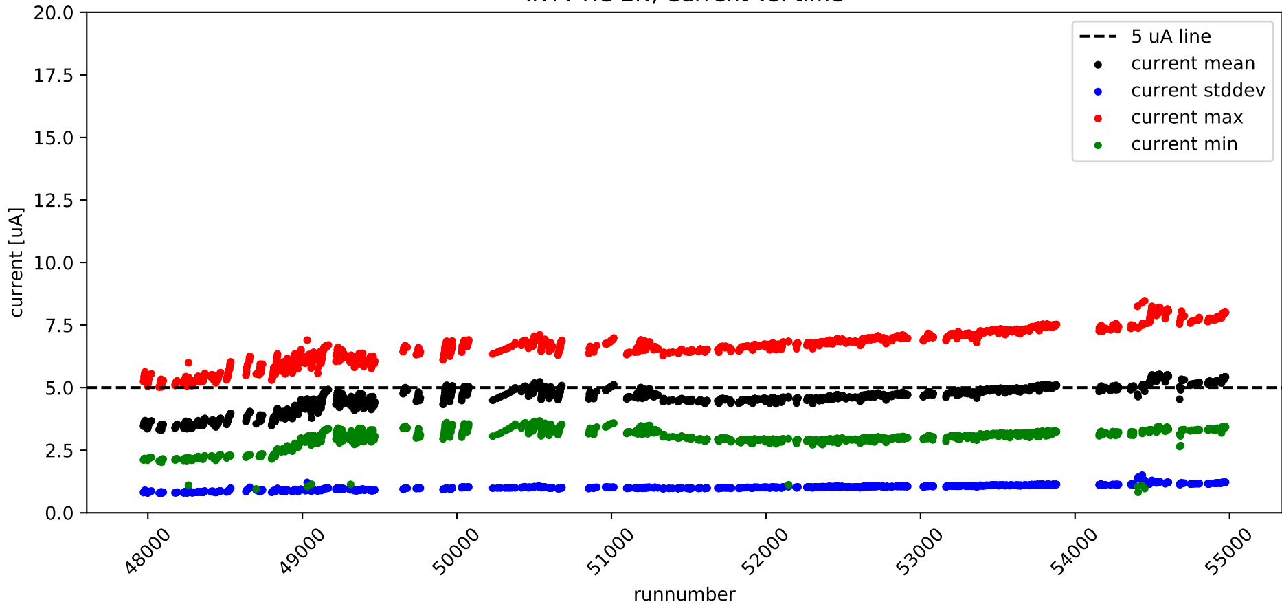
INTT RC-2N, Current vs. time
