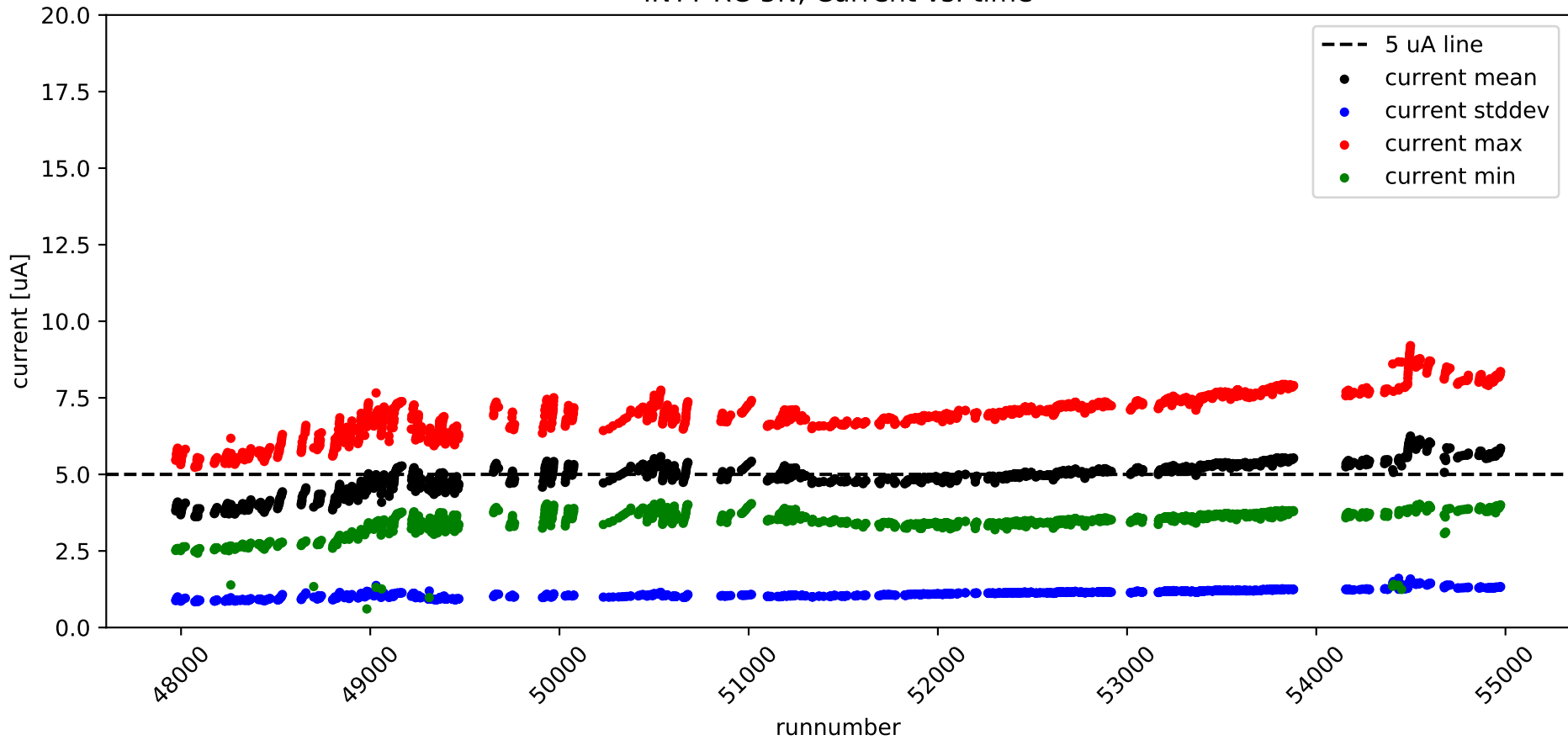
INTT RC-5N, Current vs. time
