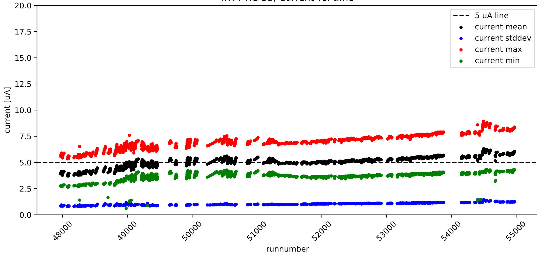
INTT RC-5S, Current vs. time
