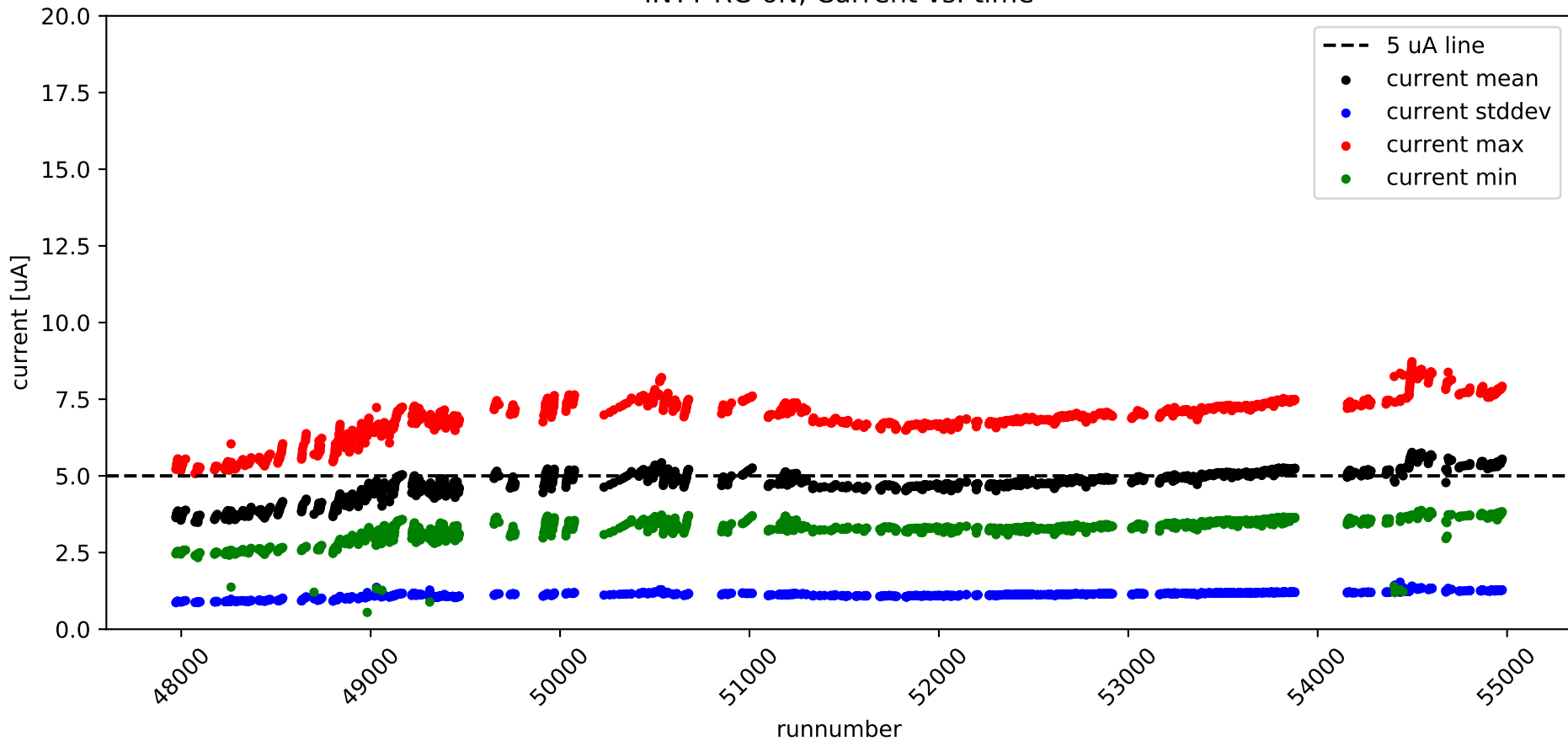
INTT RC-6N, Current vs. time
