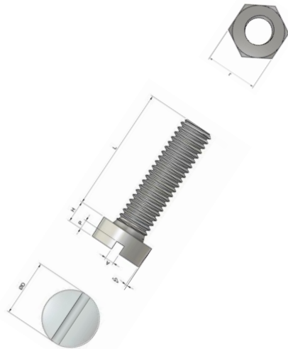
M1 SCREW & NUT FIXINGS
