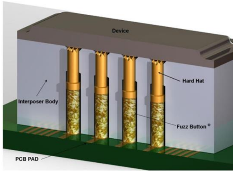
Hard Hat—Fuzz Button® Compressed With Device
