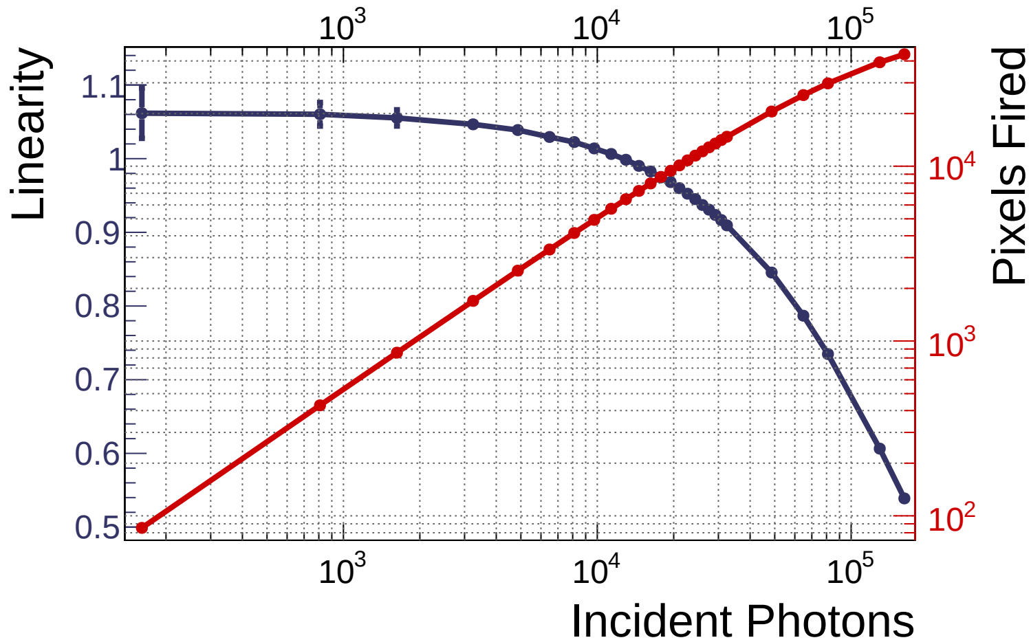
BIC Layer 5 50 mm cookie S13-BIC Linearity and Pixels Fired (50% PDE)
