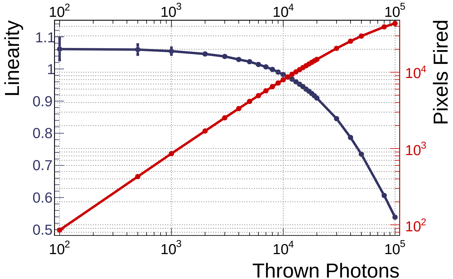
BIC Layer 5 50 mm cookie S13-BIC Linearity and Pixels Fired
