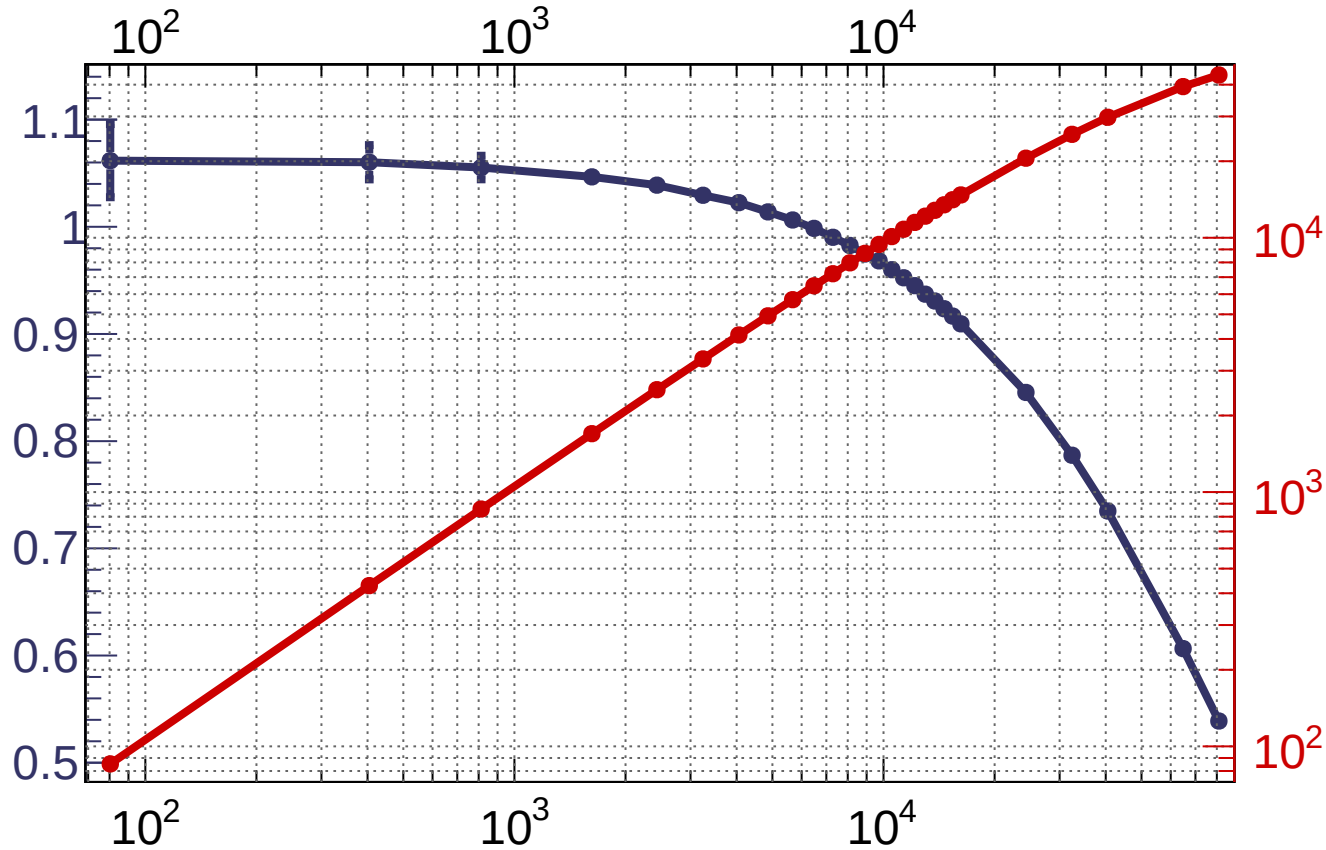
BIC Layer 5 50 mm cookie S13-BIC Linearity and Pixels Fired
