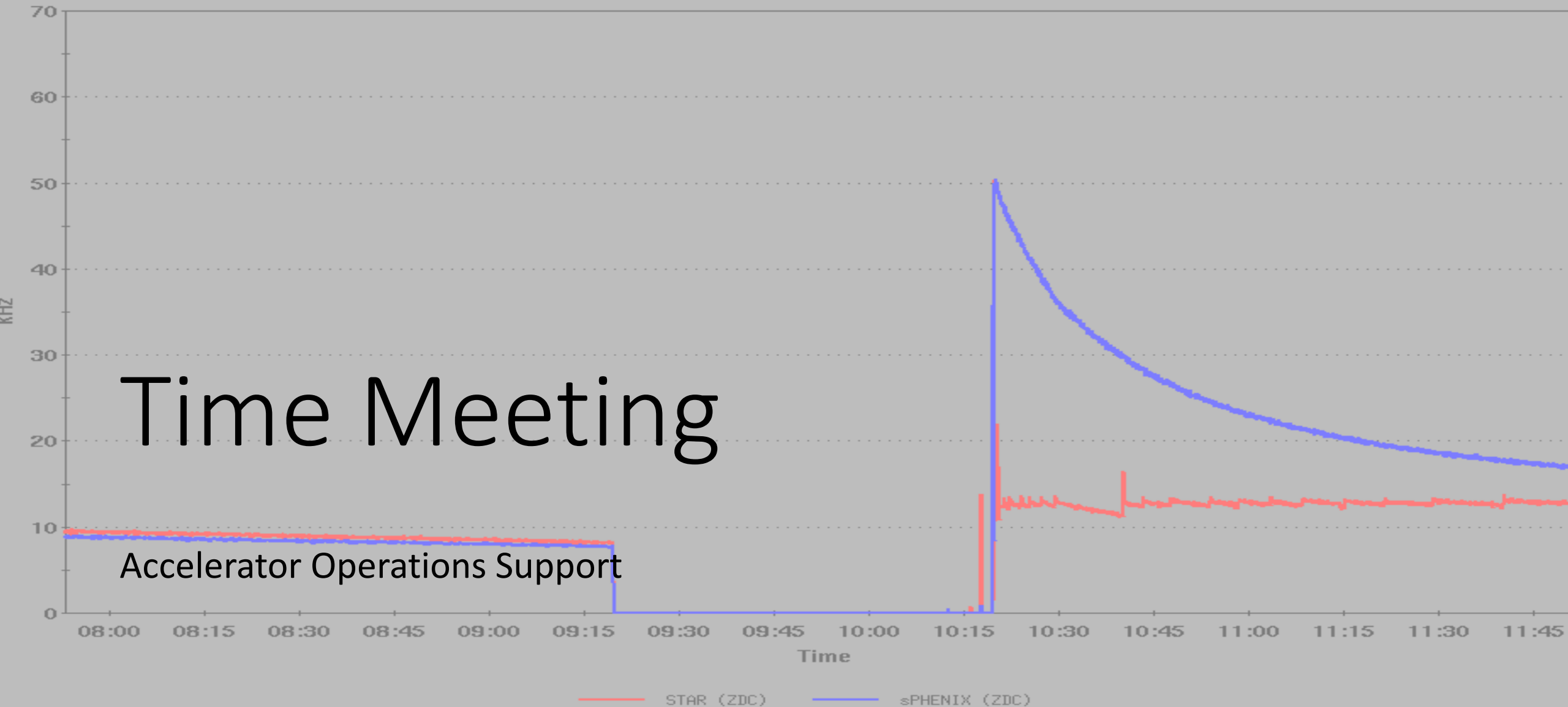
Experimental Event Rates, Tue Jun 17 11:54:01 EDT 2025
