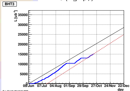
BHT3 (high- p_T )
