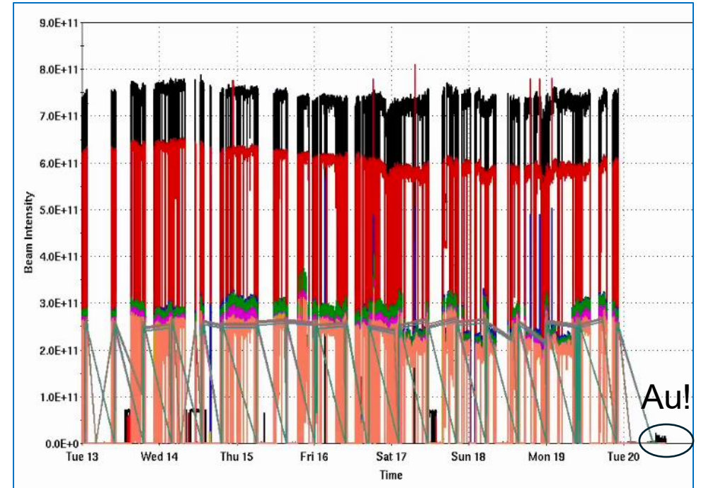
Injector Intensity (protons)
