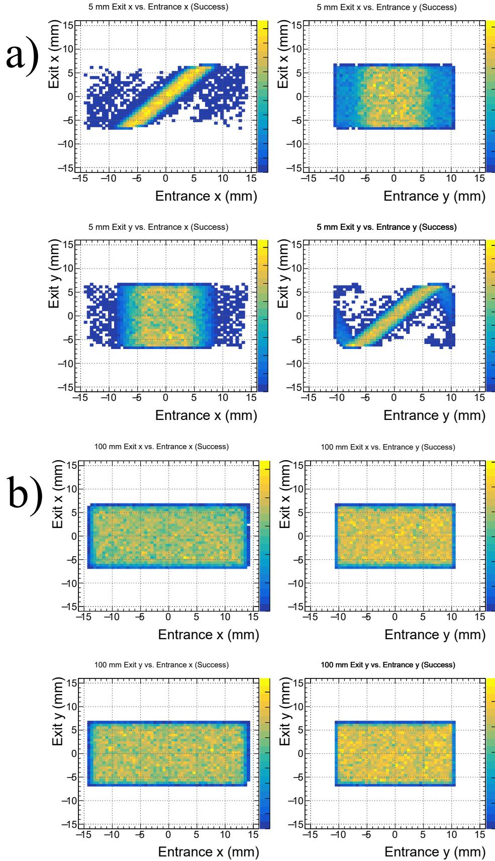
Figure 5: Example correlation plots of light guide entrance position and exit position of successful events for a) a 5-mm-long ‘b6’ guide (poor light mixing) and b) a 100-mm-long ‘b6’ guide (good light mixing). Plots normalized between values of 0 (blue) and 1 (yellow).
