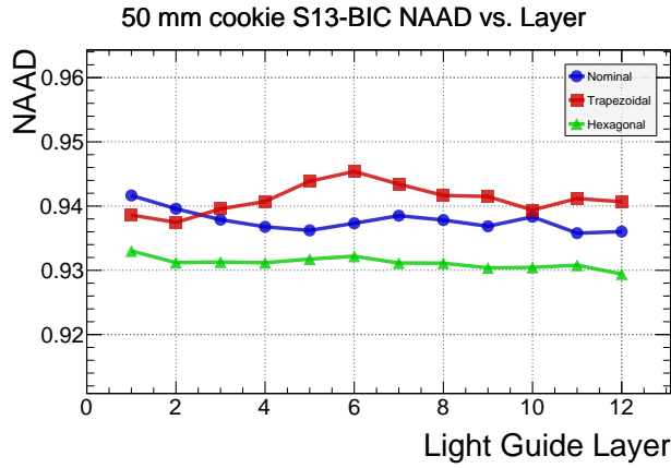
Figure 14: NAAD vs. layer number for 50-mm-long BIC guides of various shapes with a 1-mm-thick optical cookie assuming double-clad fibers (left) and single-clad fibers (right).
