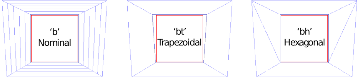
Figure 4: Geant4 renders of the Nominal (‘b’), trapezoidal (‘bt’), and hexagonal (‘bh’) BIC light guide shapes. The active SiPM area is shown in red.
