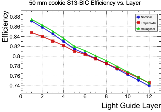
Figure 13: Efficiency vs. layer number for 50-mm-long BIC guides of various shapes with a 1-mm-thick optical cookie assuming double-clad fibers (left) and single-clad fibers (right).
