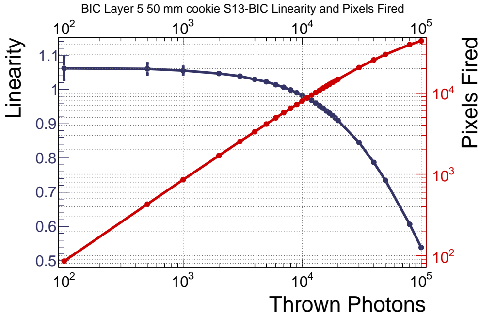
Figure 19: Average linearity and pixels fired vs. number of thrown photons for 50-mm-long, layer 5 nominal BIC light guides with a 1-mm-thick optical cookie assuming single-clad fibers.
