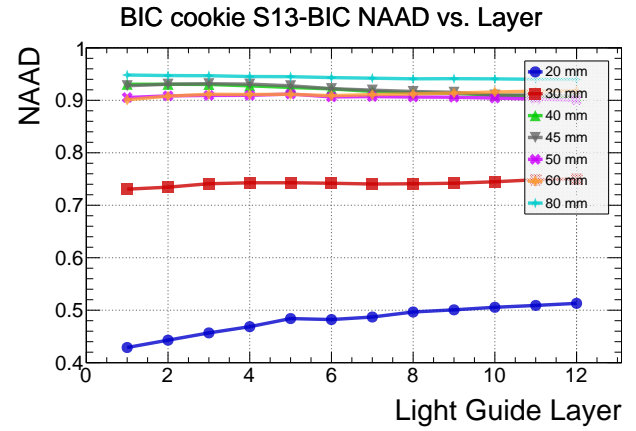
Figure 11: NAAD vs. layer number for nominal BIC guides of various lengths with a 1-mm-thick optical cookie assuming double-clad fibers (left) and single-clad fibers (right).
