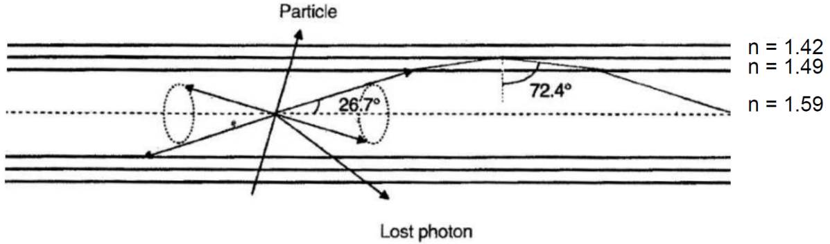
Figure 1: Visual representation of the maximum polar angle of scintillation light that escapes the end of a double-clad Kuraray fiber [2].
