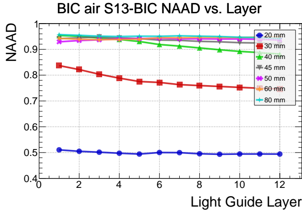
Figure 8: NAAD vs. layer number for double-clad fibers and nominal BIC guides of various lengths with a 0.5 mm air gap (left) and a 1-mm-thick optical cookie (right).
