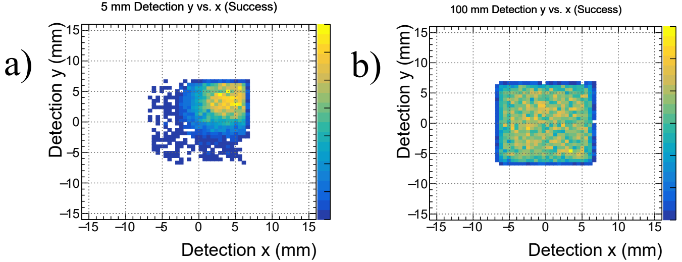
Figure 6: Example detection plots of SiPM array hit position of successful events using a quadrant source for a) a 5-mm-long ‘b6’ guide (poor light mixing) and b) a 100-mm-long ‘b6’ guide (good light mixing). Plots normalized between values of 0 (blue) and 1 (yellow).
