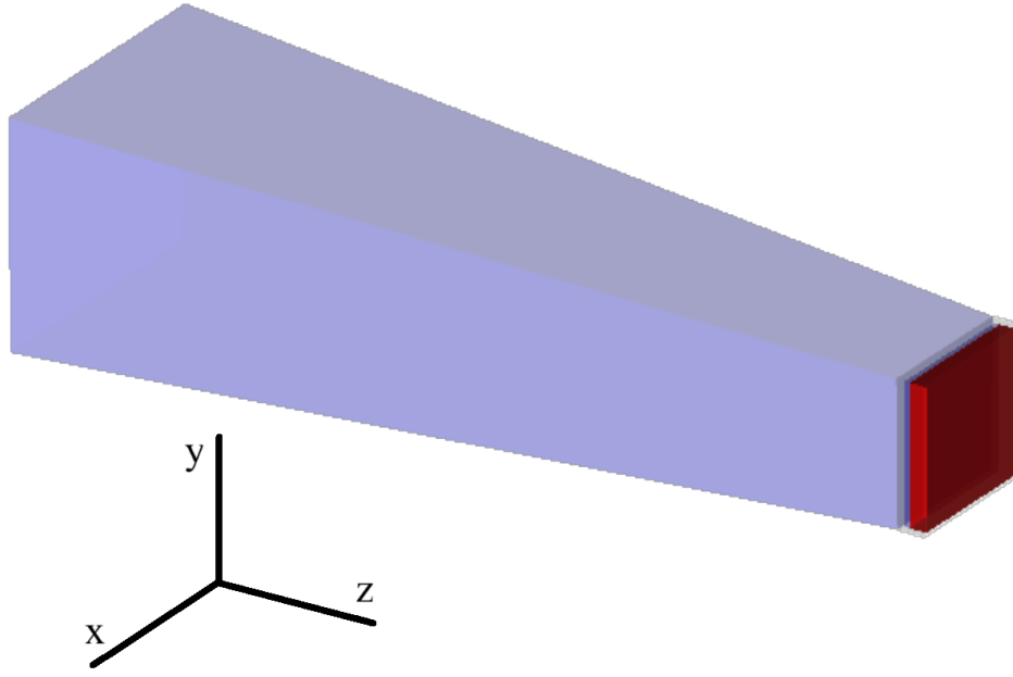
Figure 2: Geant4 rendering of the simulation setup used in Elton’s Geant3 studies featuring a g6 light guide and a SiPM separated by a 0.5 mm air gap.
