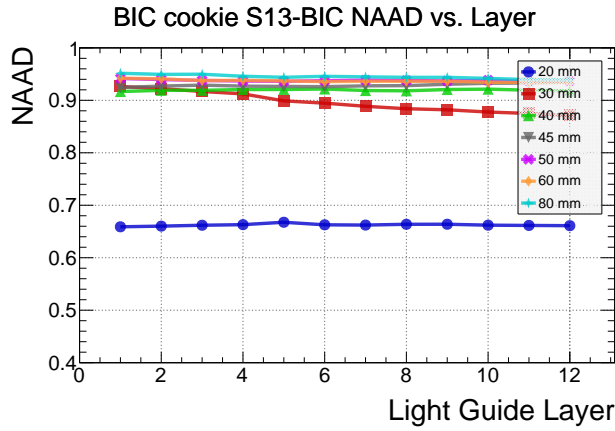
Figure 11: NAAD vs. layer number for nominal BIC guides of various lengths with a 1-mm-thick optical cookie assuming double-clad fibers (left) and single-clad fibers (right).
