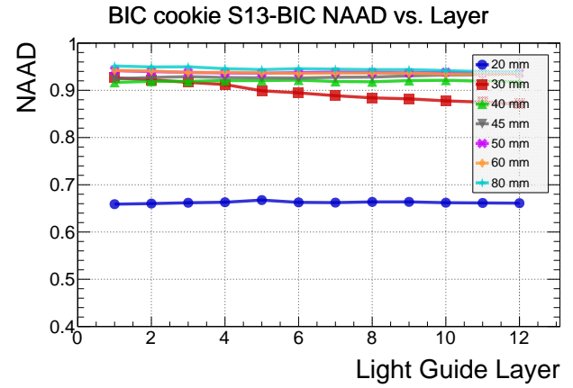
Figure 8: NAAD vs. layer number for double-clad fibers and nominal BIC guides of various lengths with a 0.5 mm air gap (left) and a 1-mm-thick optical cookie (right).
