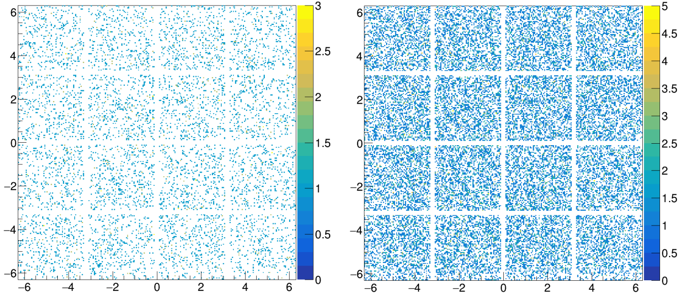
Figure 18: Detection plots, binned such that each histogram bin corresponds to one SiPM pixel 50\text{ }\mu\text{m} in pitch, from quadrant source simulations of a 50-mm-long, layer 5 nominal BIC light guide with a 1-mm-thick optical cookie and single-clad fibers showing events with 10000 thrown photons (left) 40000 thrown photons (right).
