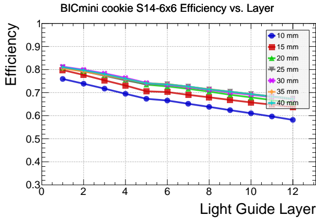
Figure 16: Efficiency vs. layer number (left) and NAAD vs. layer number (right) for double-clad fibers and BIC mini guides of various lengths with a 1-mm-thick optical cookie and an S14 SiPM.
