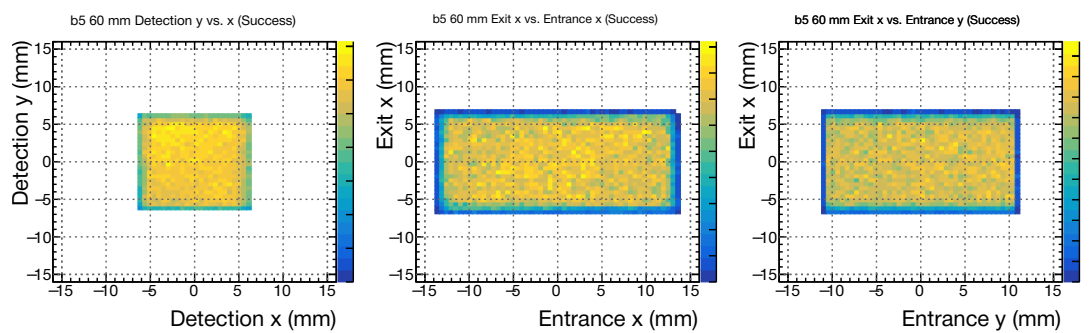
Figure 9: Detection (left) and correlation (middle and right) plots for BIC guides of various lengths (rows) with double-clad fibers and a 1-mm-thick optical cookie. Plots normalized between values of 0 (blue) and 1 (yellow).
