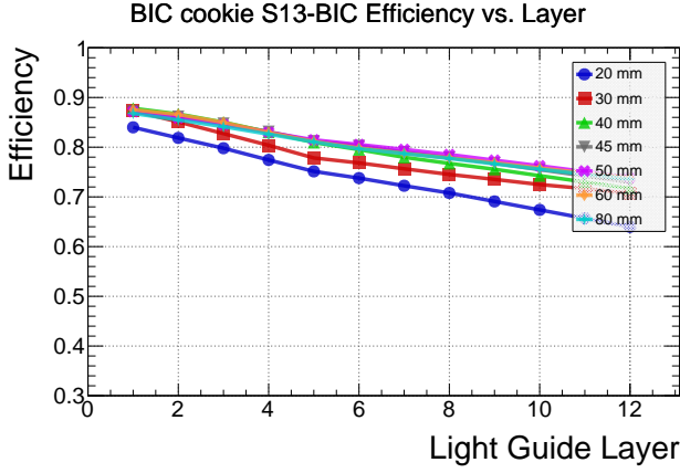
Figure 10: Efficiency vs. layer number for nominal BIC guides of various lengths with a 1-mm-thick optical cookie assuming double-clad fibers (left) and single-clad fibers (right).
