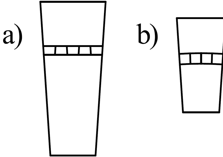
Figure 3: Light guide layout scheme for a) ePIC's BIC sector and b) GlueX's BCAL module. Diagrams are to-scale relative to each other. Layer 7 light guides are shown in each diagram.
