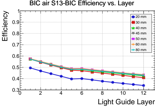
Figure 7: Efficiency vs. layer number for double-clad fibers and nominal BIC guides of various lengths with a 0.5 mm air gap (left) and a 1-mm-thick optical cookie (right).
