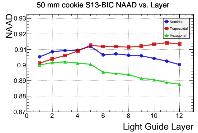
Figure 14: NAAD vs. layer number for 50-mm-long BIC guides of various shapes with a 1-mm-thick optical cookie assuming double-clad fibers (left) and single-clad fibers (right).
