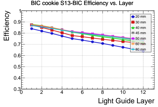
Figure 7: Efficiency vs. layer number for double-clad fibers and nominal BIC guides of various lengths with a 0.5 mm air gap (left) and a 1-mm-thick optical cookie (right).
