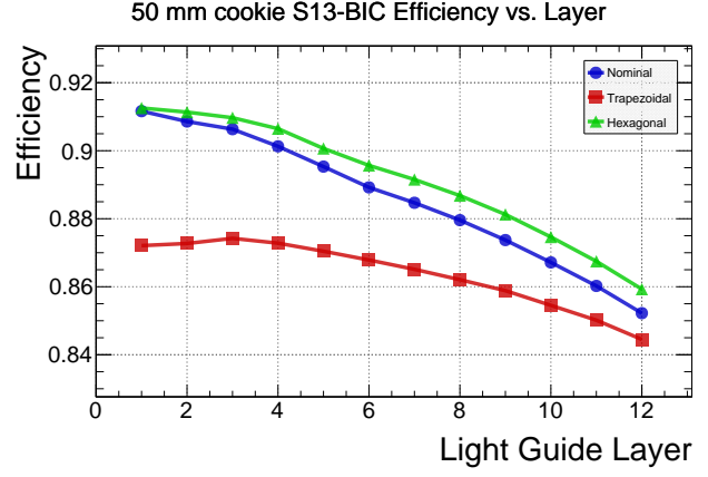
Figure 13: Efficiency vs. layer number for 50-mm-long BIC guides of various shapes with a 1-mm-thick optical cookie assuming double-clad fibers (left) and single-clad fibers (right).
