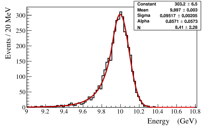
Fig. 9. Energy distribution deposited by 10 GeV beam photons. The spectrum is fit to a Crystal Ball function.
