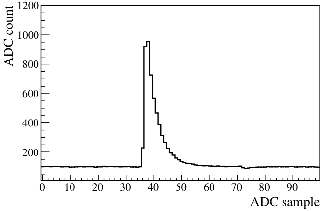
Fig. 4. A typical flash ADC signal pulse obtained from a \text{PbWO}_3 module.
