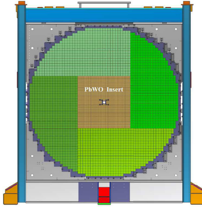
Fig. 15. FCAL frame with calorimeter modules installed: PbWO 4 crystals (brown area), lead glass blocks (green). The photon beam passes through the hole in the middle of the calorimeter. (For interpretation of the references to color in this figure legend, the reader is referred to the web version of this article.)
