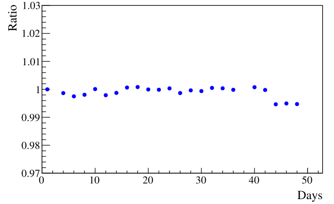
Fig. 6. Ratio of signal ADC amplitudes from the LED pulser to the \alpha -source measured by the reference PMT during different run periods of the 48-day long PrimEx- \eta experiment. The ratio is normalized to data in the beginning of the run.
