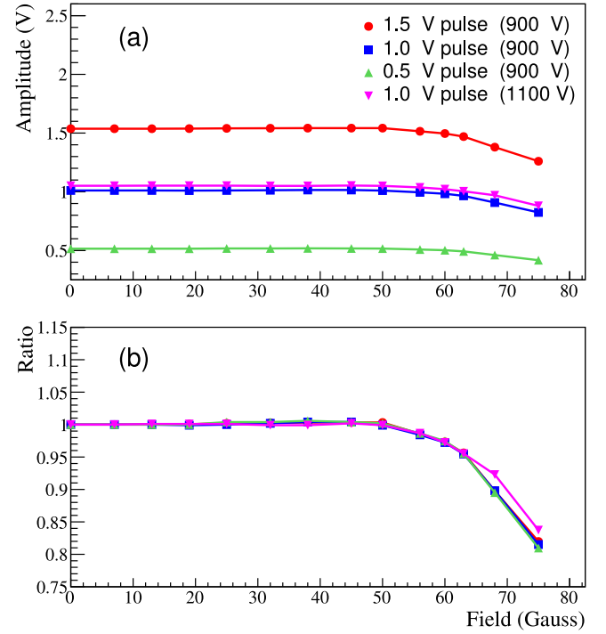
Fig. 17. Signal amplitudes of shielded PMT induced by an LED as a function of the magnetic field (a). Amplitudes, normalized to measurements without magnetic field (b). The PMT response was measured for different intensities of light pulse and HV settings as shown by different polymarkers.
