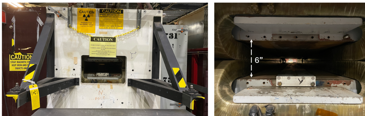
Figure 2 18D72 dipole (left) has a 6" high bore (right).
