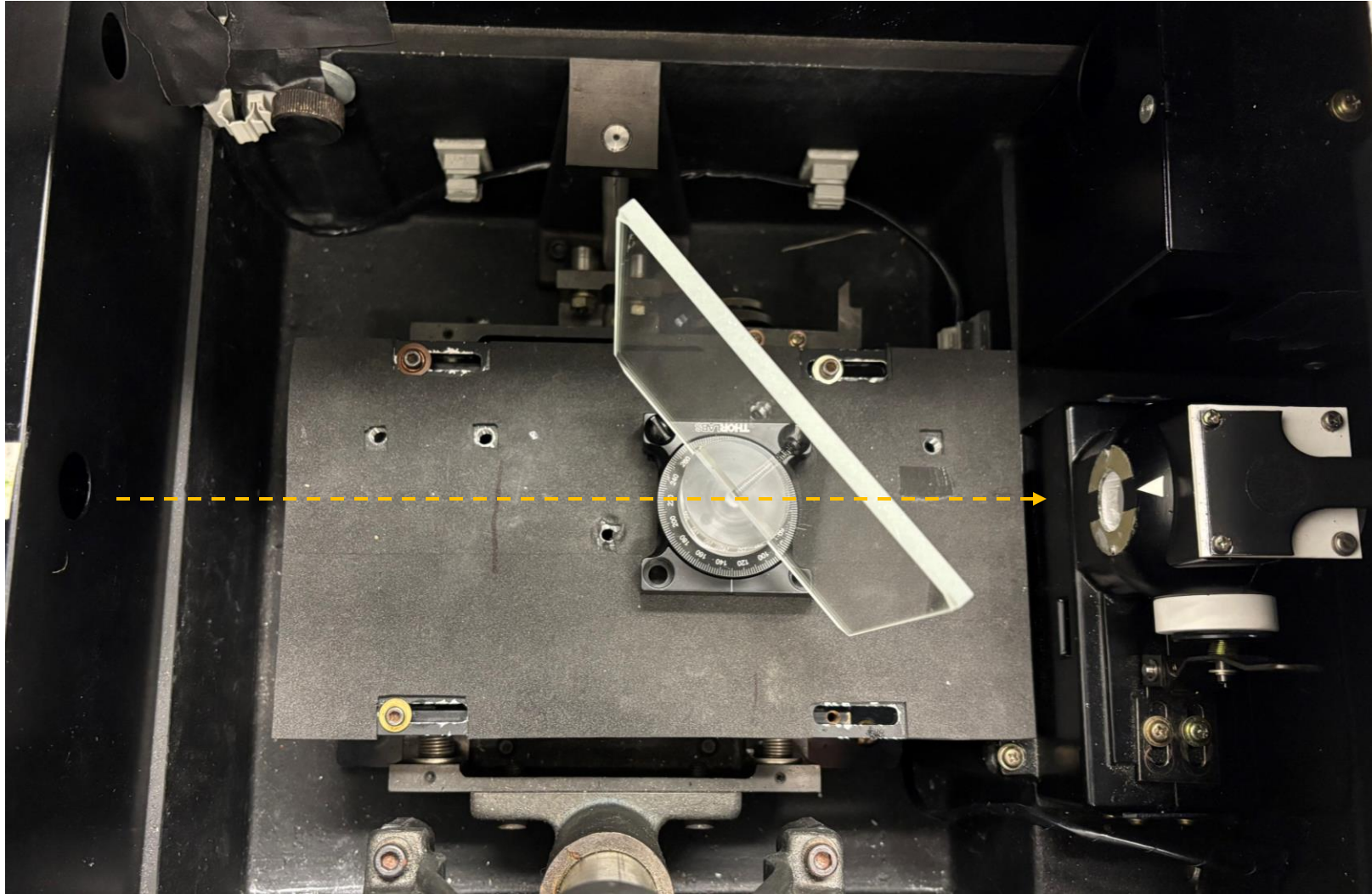
Window mounted in Hitachi spectrophotometer chamber
