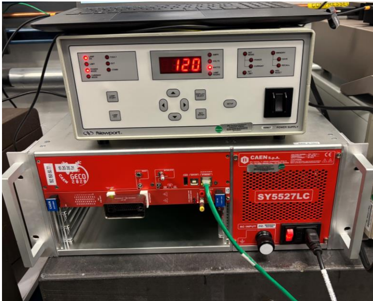
Light source power supply and Caen crate for HRPPD power module
