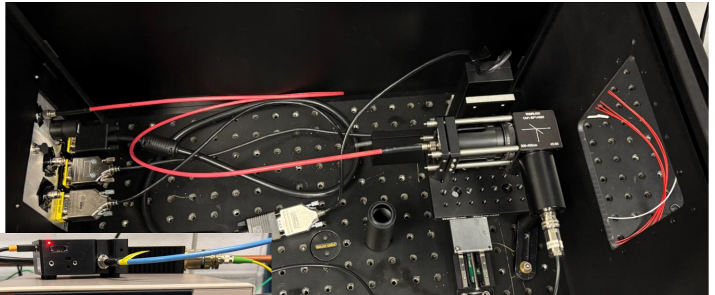
Inside darkbox - scanner head with light input fiber And monitoring photodiode
