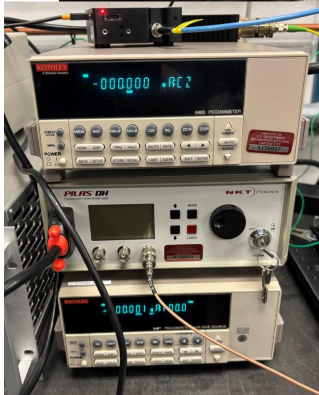
Kiethley 6487 voltage source / picoammeters PiLas Laser Controller
