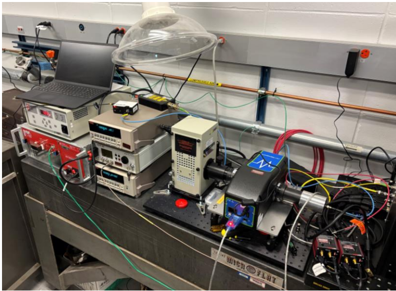
Full equipment setup on test bench.
