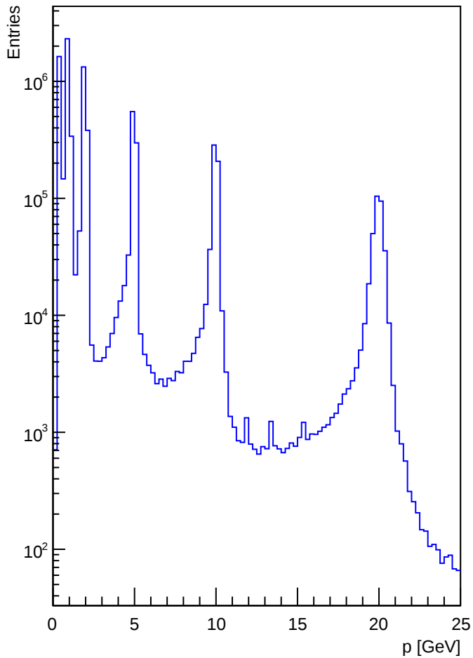
Track p distribution for e-
