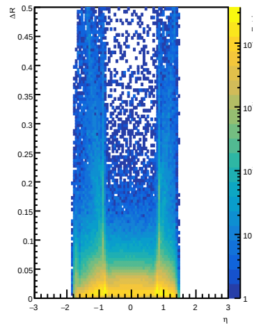
EcalBarrelTrackClusterMatches \Delta R vs \eta for e-
