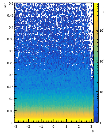
EcalBarrelTrackClusterMatches \Delta R vs \phi for e-
