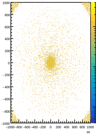
LFHCALTrackClusterMatches dxdy for e-
