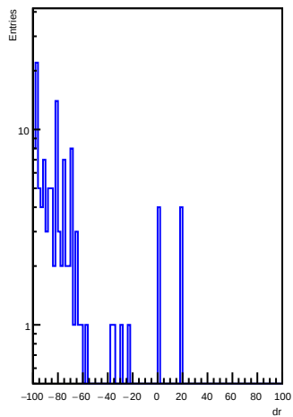
HcalEndcapNTrackClusterMatches dr for e-
