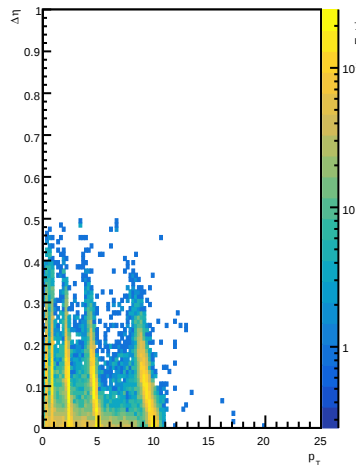
LFHCALTrackClusterMatches \Delta \eta for e-
