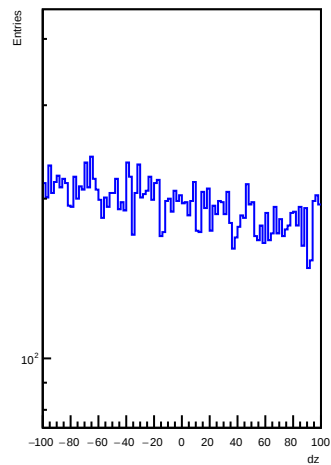
EcalEndcapPTrackClusterMatches dz for e-
