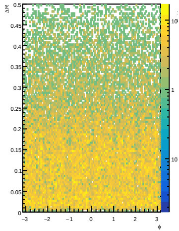
LFHCALTrackClusterMatches \Delta R vs \phi for e-
