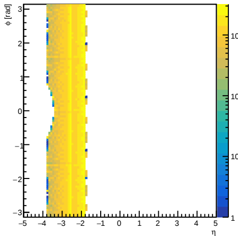
HcalEndcapNClusters eta-phi location for e-
