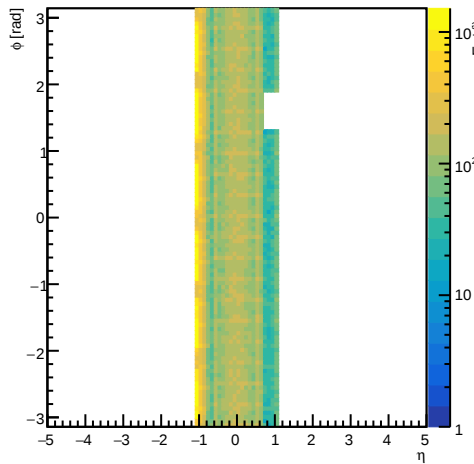
HcalBarrelClusters eta-phi location for e-
