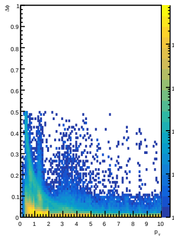
EcalBarrelTrackClusterMatches \Delta \phi for e-
