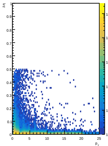
EcalBarrelTrackClusterMatches \Delta \eta for e-
