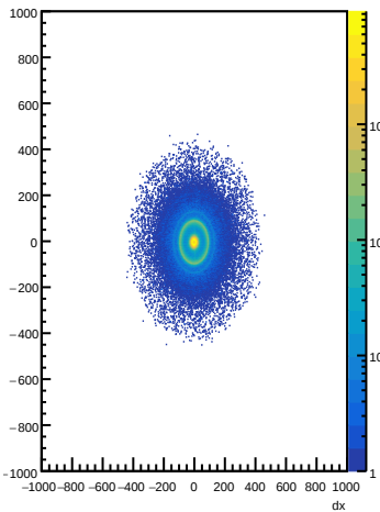
EcalBarrelTrackClusterMatches dxdy for e-
