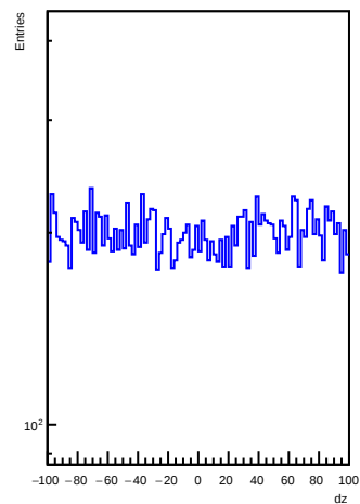
HcalBarrelTrackClusterMatches dz for e-
