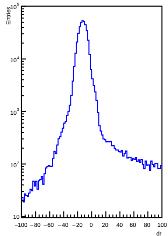
EcalEndcapNTrackClusterMatches dr for e-
