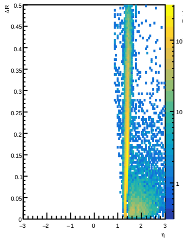
LFHCALTrackClusterMatches \Delta R vs \eta for e-
