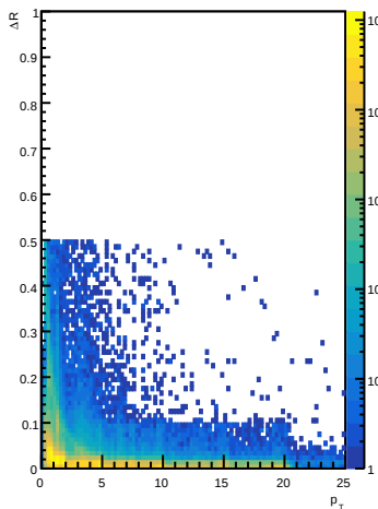
EcalBarrelTrackClusterMatches \Delta R for e-
