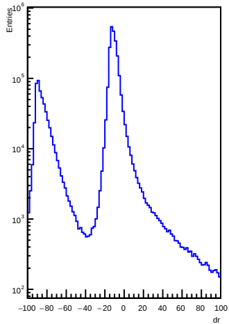
EcalBarrelTrackClusterMatches dr for e-
