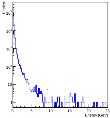
HcalEndcapNClusters energy distribution for e-
