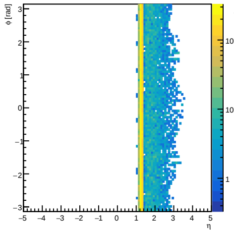
LFHCALClusters eta-phi location for e-
