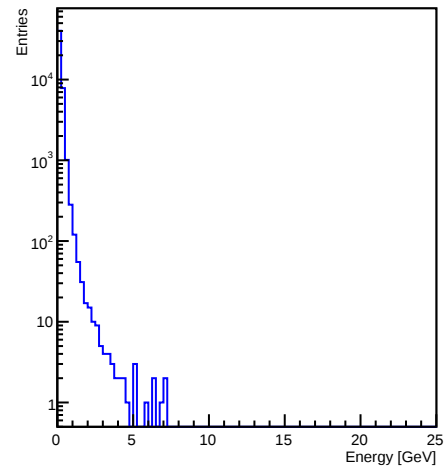
LFHCALClusters energy distribution for e-
