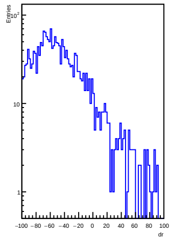
LFHCALTrackClusterMatches dr for e-
