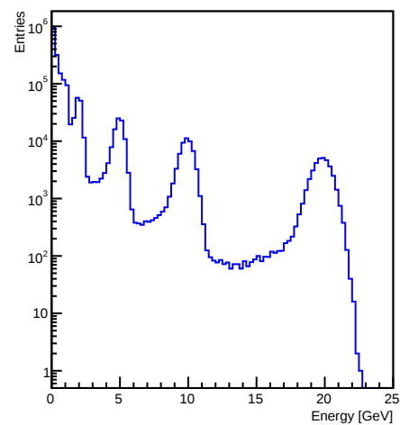
LFHCALClusters energy distribution for e-
