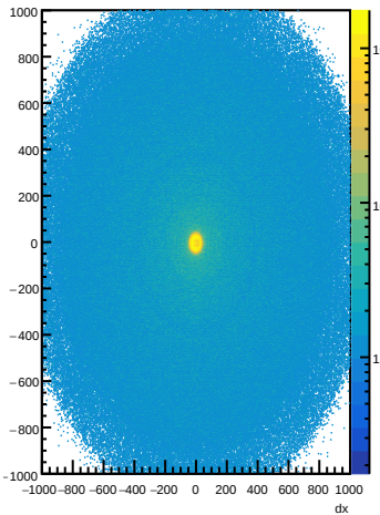
EcalEndcapPTrackClusterMatches dxdy for e-
