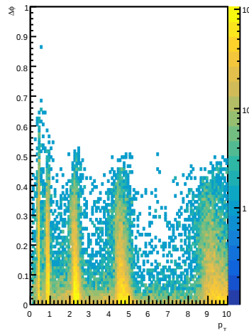
LFHCALTrackClusterMatches \Delta \phi for e-
