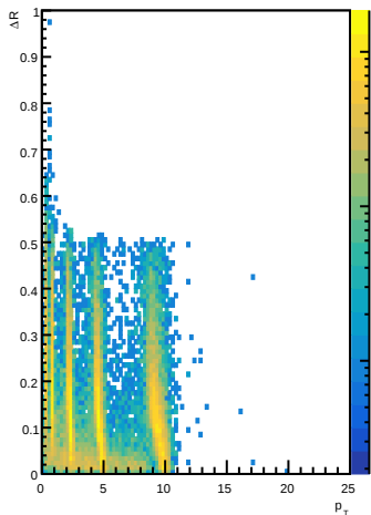
LFHCALTrackClusterMatches \Delta R for e-
