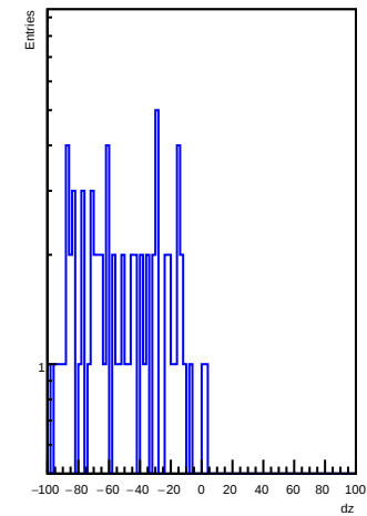
LFHCALTrackClusterMatches dz for e-
