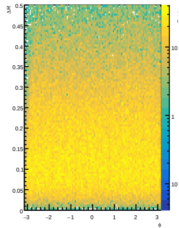
HcalBarrelTrackClusterMatches \Delta R vs \phi for e-
