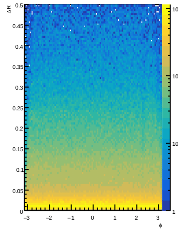
EcalEndcapPTrackClusterMatches \Delta R vs \phi for e-
