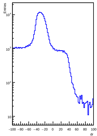
EcalEndcapPTrackClusterMatches dr for e-
