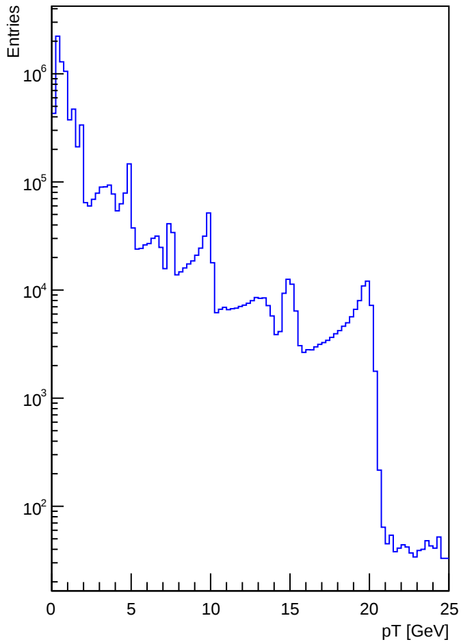
Track pT distribution for e-
