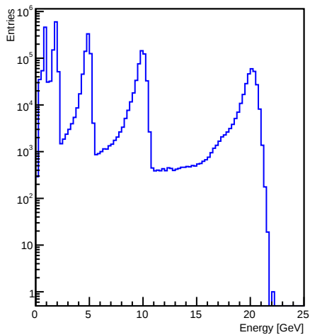
HcalBarrelClusters energy distribution for e-
