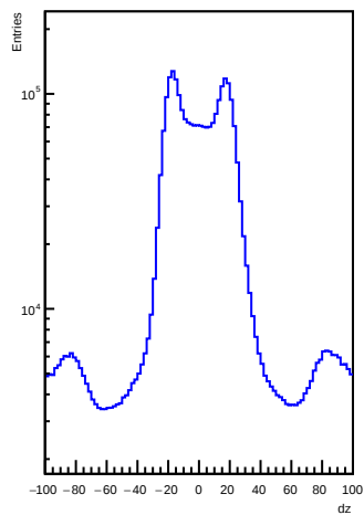
EcalBarrelTrackClusterMatches dz for e-
